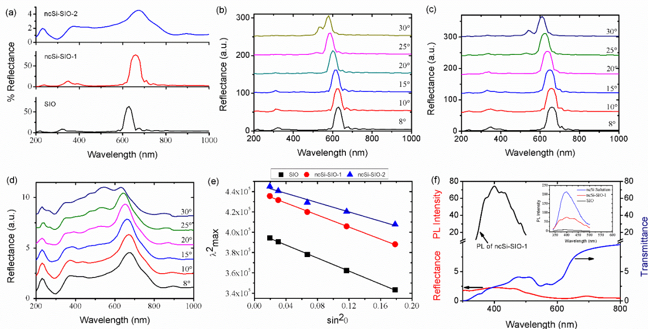
Fig. 2. (a) Reflection spectra of SIO, SIO-1 and SIO-2 samples recorded at an incidence angle of 8° to the opal surface normal. (b) Angle-resolved reflection spectra of SIO (c) ncSi-SIO-1 and (d) ncSi-SIO-2 samples recorded at incidence angles 8° to 30°. (e) Plot of \sin^2\theta vs \lambda_{\text{max}}^2 of the three opals. (f) PL emission spectra of ncSi-SIO-1 collected at 60° angle to the opal surface normal (black line) and optical reflection and transmission spectra of the same sample at 60° incidence (red and blue lines). The PL emission spectra of ncSi-SIO-1, SIO before infiltration and ncSi solution are presented as inset of (f).
