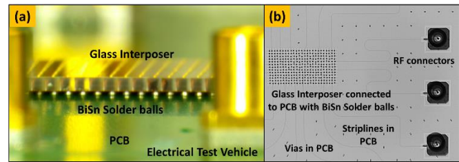
Fig. 10. (a) Side view of the electrical test vehicle showing the Bi-Sn solder balls bonding the glass interposer on the PCB for RF characterization. This side view is pictured after the Bi-Sn solder reflow and before epoxy underfilling. (b) X-ray imaging analysis of the electrical test vehicle.
