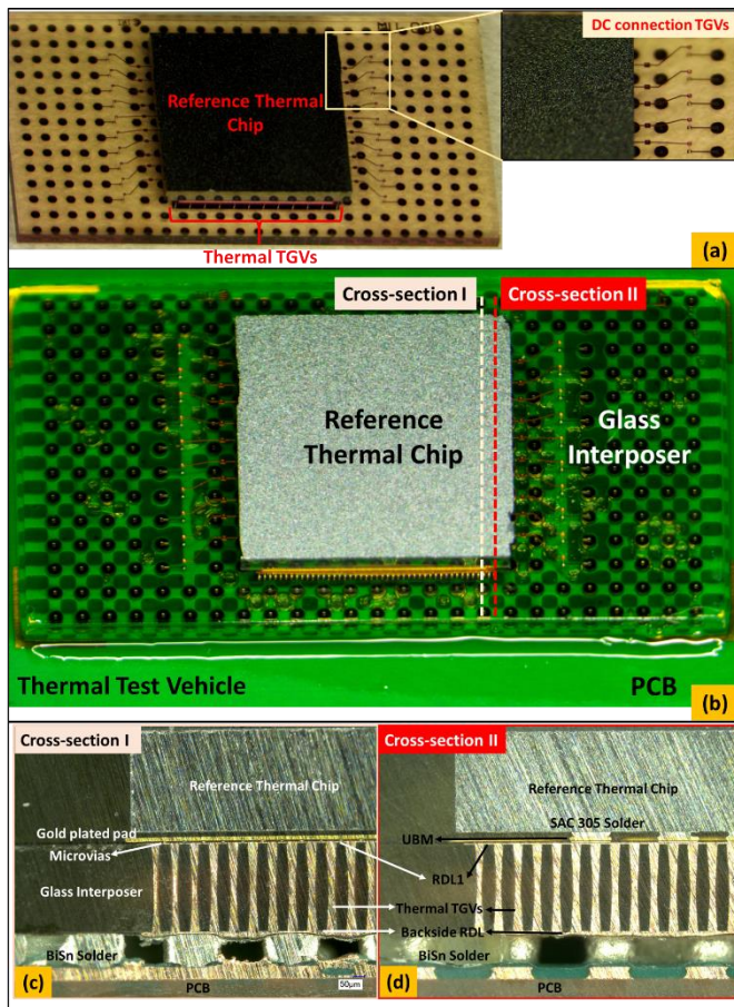
Fig. 4. (a) Perspective view of the subassembly containing flip-chip bonded reference thermal chip on glass interposer. (b) Top view of the thermal test vehicle showing assembled reference thermal chip and glass interposer (thermal TGV pitch of 100 \mu\text{m} ) on PCB, with underfill between the reference thermal chip-glass interposer and glass interposer-PCB interfaces. The cross-sectional lines are specified in the figure. (c) Cross-sectional view of the thermal test vehicle along cross-sectional line 1. (d) Cross-sectional view of the thermal test vehicle along cross-sectional line 2.
