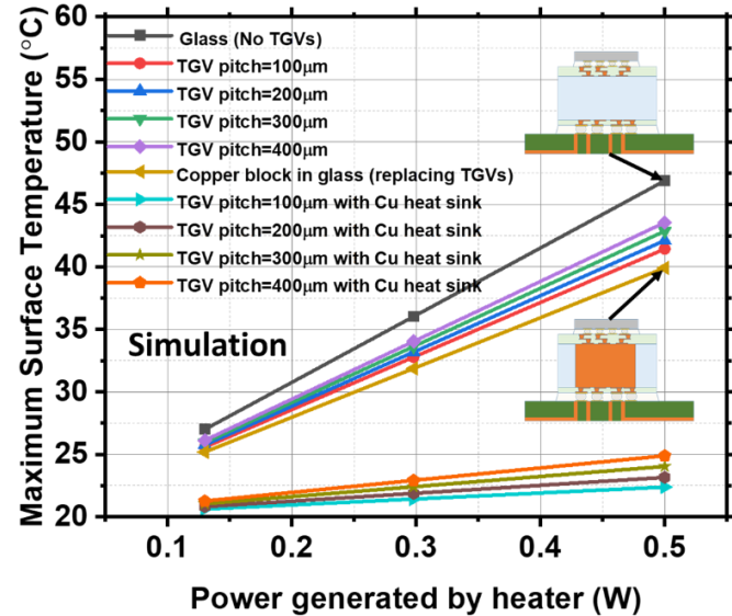
Fig. 9. Variation of the chip's maximum surface temperature with variation in the TGV pitch (100 \mu\text{m} , 200 \mu\text{m} , 300 \mu\text{m} and 400 \mu\text{m} ). The figure also shows a significant decrease in maximum surface temperature with a heat sink embedded in the PCB, where the heat sink is the same size as that of the chip.
