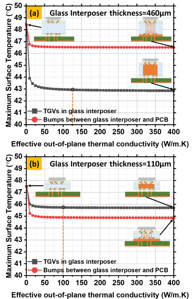
Fig. 8. Simulated variation in the chip's maximum surface temperature with the change in out-of-plane effective thermal conductivity of TGVs and bumps between glass interposer and PCB (with underfill) when the glass thickness/TGV height is (a) 460 \mu\text{m} and (b) 110 \mu\text{m} respectively. PCB (with underfill).
