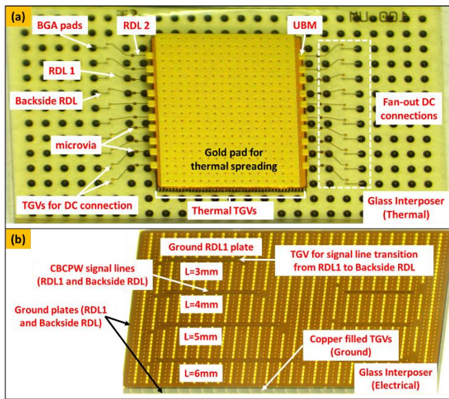
Fig. 3. Perspective view of the fabricated glass interposer for (a) thermal characterization with 100 \mu\text{m} pitch thermal TGVs in the interposer; (b) electrical characterization which includes CPW transmission lines on top and bottom of the glass surface which is interconnected through TGVs.
