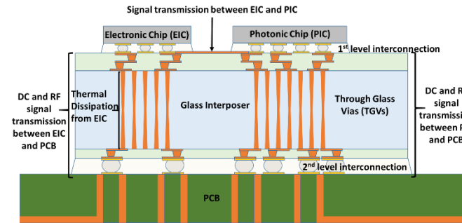
Fig. 1. A 2.5D glass interposer package consisting of co-packaged electronic (EIC) and photonic (PIC) chips bonded on the glass interposer (first-level interconnections); which is subsequently bonded on the PCB (second-level interconnections).
