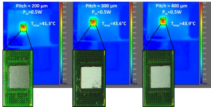
Fig. 5. Infrared thermal measurement showing surface temperature of the flip-chip bonded reference thermal chip on the glass interposer in thermal test vehicle exhibiting thermal TGV pitches of 200, 300 and 400 \mu\text{m} .
