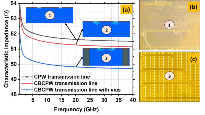
Fig. 12. (a) Variation of characteristic impedance with frequency for the CPW transmission line on glass, conductor backed CPW transmission line (CBCPW) and CBCPW transmission line with via fence connecting the side grounds to the backside ground on top and bottom of the glass interposer with their respective electric field distributions at 20 GHz. (b) shows the top view of the fabricated CPW transmission line on the glass interposer with no backside ground and TGVs and (c) shows the top view of the fabricated CBCPW transmission line with TGVs in the glass interposer.
