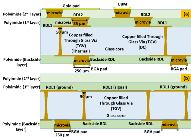
Fig. 2. Details of the glass interposer stackup for (a) thermal characterization with different components such as BGA pads, thermal and DC connection TGVs, microvias, RDL wiring and UBM; (b) electrical characterization with different components such as RDL wiring, signal and ground TGVs, microvias and BGA pads.
