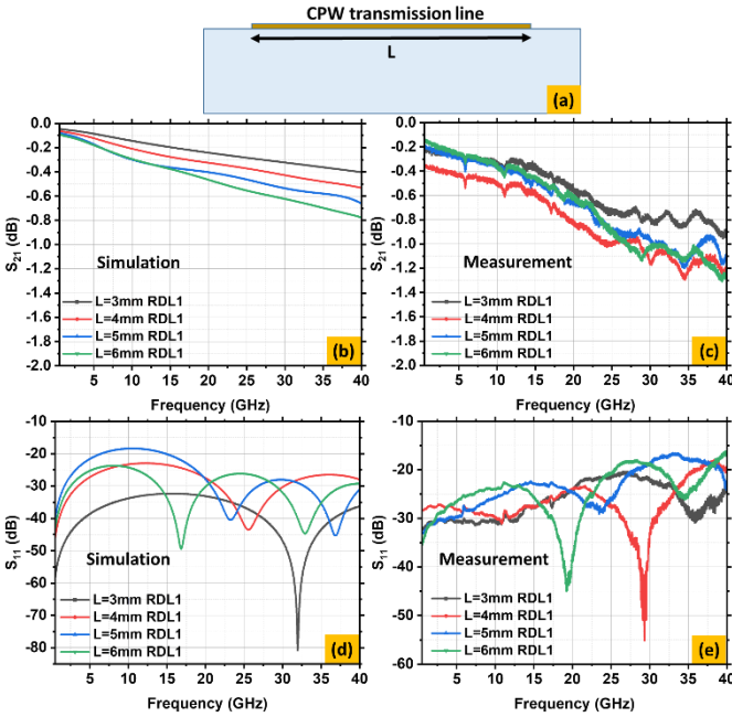
Fig. 11. (a) Schematic showing CPW transmission line on glass. (b) Simulated and (c) measured insertion loss for the CPW transmission line (RDL1) with varying lengths on glass. (d) Simulated and (e) measured return loss for CPW transmission lines on glass with varying lengths.
