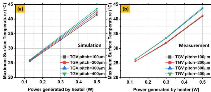
Fig. 7. Comparison of the (a) simulated and (b) measured maximum surface temperatures of the backside of the flip-chip attached reference chip in the thermal test vehicle using different TGV pitches in the glass interposer with increasing input power of the heater loopback in the chip.
