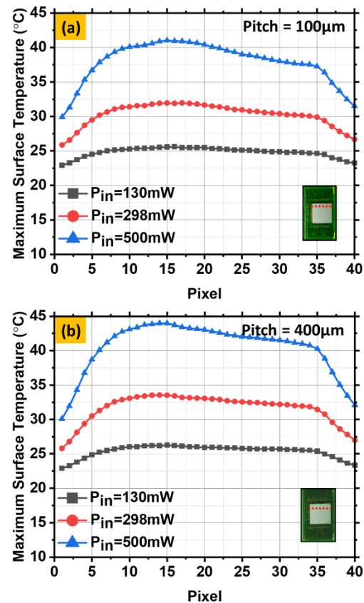
Fig. 6. Maximum surface temperature measurement across the topside of the flip-chip attached reference thermal chip (along the horizontal axis shown as dashed lines in the inset for (a) 100 \mu\text{m} and (b) 400 \mu\text{m} pitch TGVs with increasing input powers of the heater loopback ( P_{\text{in}} ). The heater loopback at the corner of the chip is being operated in both (a) and (b).
