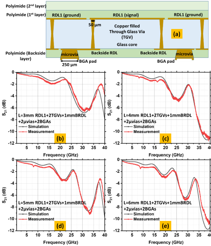
Fig. 13. (a) Schematic showing glass interposer for electrical characterization. Simulated and measured insertion loss results for the glass interposer with different lengths of the RDL1 line on top (b) 3 mm, (c) 4 mm, (d) 5 mm and (e) 6 mm.
