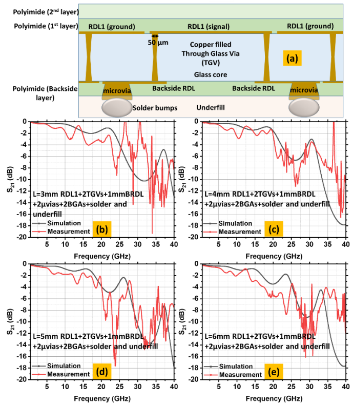
Fig. 15. Schematic showing the electrical test vehicle for characterization (with de-embedded PCB losses). Simulated and measured insertion loss results for the de-embedded test vehicle with different lengths of the RDL1 line (b) 3 mm, (c) 4 mm, (d) 5 mm and (e) 6 mm.
