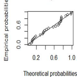
P-P plot
