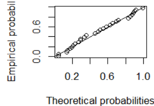
P-P plot
