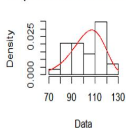
Empirical and theoretical de
