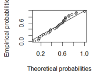
P-P plot
