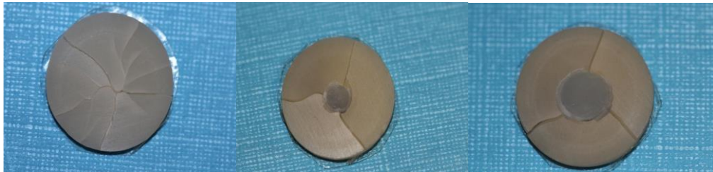
a) b) c) Figure 4.3. Photograph of lithium disilicate glass-ceramic disc substrates exhibiting a) a classic high-strength fracture pattern for an intact specimen b) a low-strength fracture pattern for a 3 mm representative endodontic access cavity repaired with a high modulus of elasticity resin composite, c) a low-strength fracture pattern for a 5 mm representative endodontic access cavity repaired with a high modulus of elasticity resin composite.
