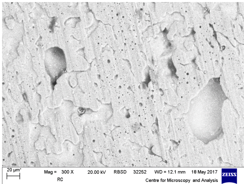
Figure 9.5. Scanning electron micrograph (×300) of the debonded surface of a resin composite (Tetric Evoceram) substrate which demonstrated adhesive failure for a lithium disilicate glass-ceramic (IPS e.max® Press).
