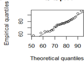
Q-Q plot
