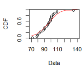
Empirical and theoretical CDF
