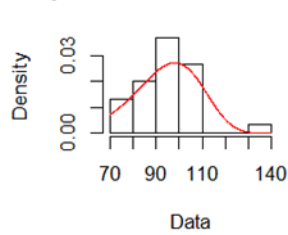
Empirical and theoretical de
