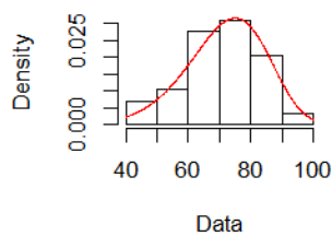
Empirical and theoretical de
