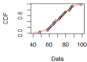
Empirical and theoretical CDF
