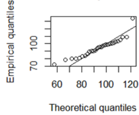
Q-Q plot
