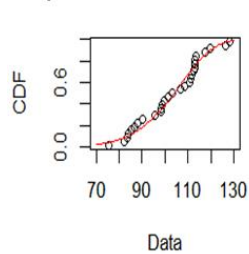
Empirical and theoretical CDF
