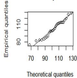
Q-Q plot
