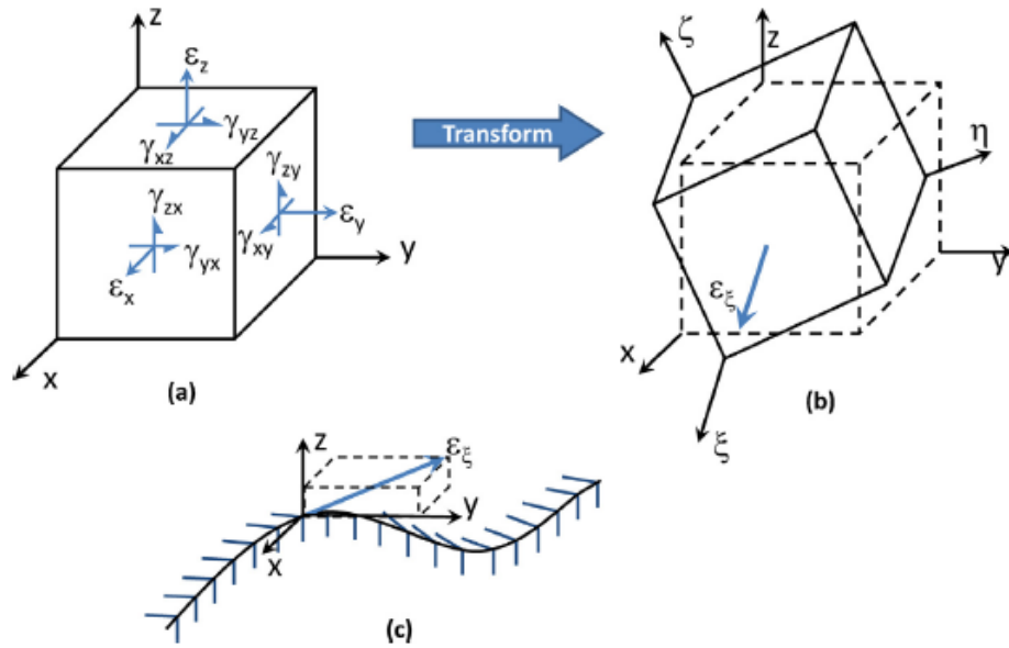
Figure 6.10. Transformation of the Cartesian strains, (\epsilon_x, \epsilon_y, \epsilon_z, \gamma_{xy}, \gamma_{yz}, \gamma_{zx}) , to a strain component, \epsilon_\xi , along the ceramic/filler interface edge.
