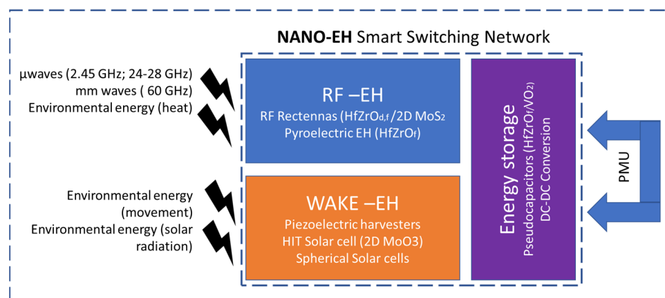
Figure 1. Conceptual schematic of the NANO-EH energy supply platform and included modules.
