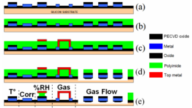
Figure 1: Multisensor fabrication process. From left to right: temperature sensor, corrosion sensor, humidity sensor, gas sensor, gas flow velocity sensor.
