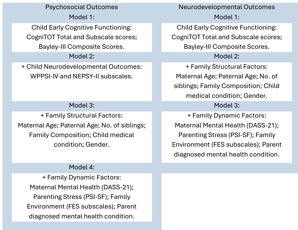
Figure 2 Hierarchical Multiple Regression Models for Psychosocial and Neurodevelopmental Outcomes
