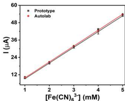
Fig. 8. Mean and standard deviation values for both the prototype and Autolab - Same potential with different concentrations.
