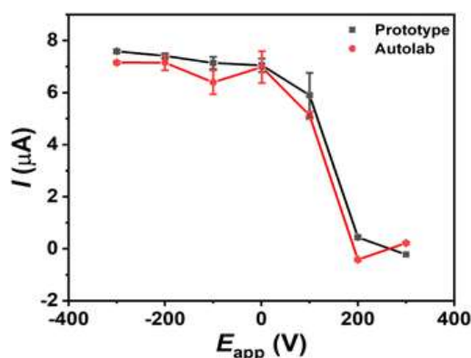
Fig. 7. Mean and standard deviation values for both the prototype and Autolab - Different potentials with the same concentration.
