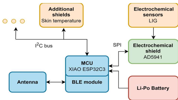
Fig. 1. Block diagram of the proposed device.
