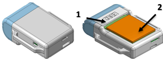
Fig. 4. Measurement platform outlook: enclosure, biochemical sensor (1), microfluidic interface (2).
