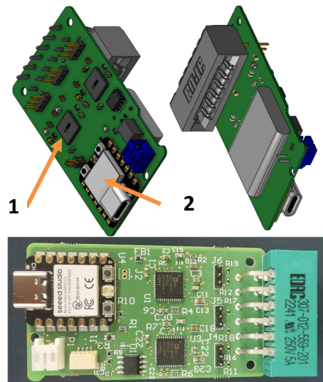
Fig. 2. Electrochemical shield (1), IoT base board XIAOESP32C3 (2).
