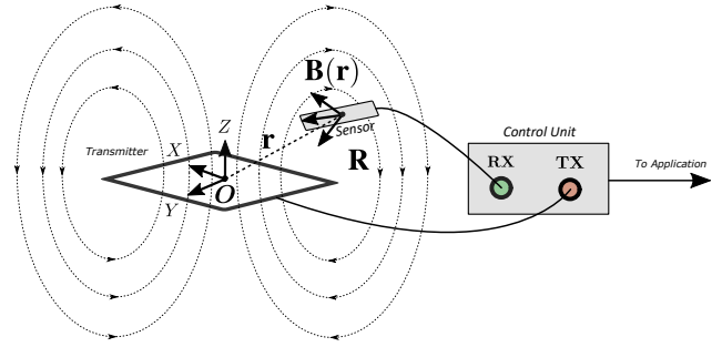
Figure 1. An electromagnetic tracking system.
