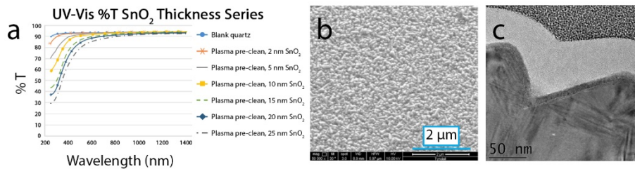
Figure 4: (a) % Transmission spectra (b) Plan view SEM showing surface morphology of 20 nm ALD- \text{SnO}_2 pre-treated with \text{O}_2 plasma (c) TEM of 10 nm ALD- \text{SnO}_2 pre-treated with \text{O}_2 plasma.
