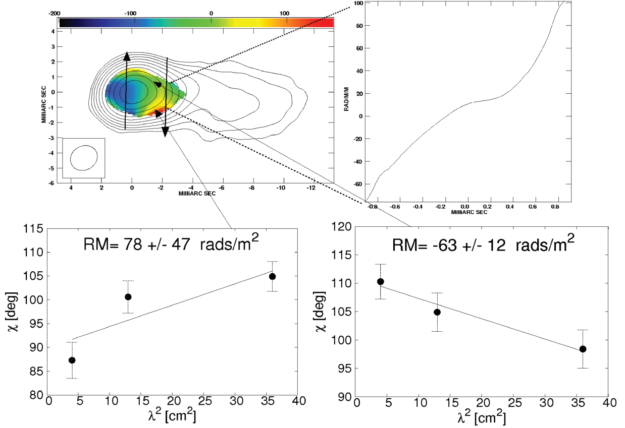
Figure 4. RM map of B1803+784 observed on 1997 April 6. The range of RM values shown in the colour bar is in units of \text{rad m}^{-2} . The I contours are those for 8.4 GHz. The peak flux ( \text{Jy beam}^{-1} ) is 1.9 \text{ Jy beam}^{-1} and the lowest contour is 2.0 \text{ mJy beam}^{-1} . The accompanying panels show a slice of the RM distribution across the jet, and plots of the polarization angle \chi versus \lambda^2 for the indicated 3 \times 3 pixel regions near the top and bottom of the jet. The errors shown are 1\sigma .
