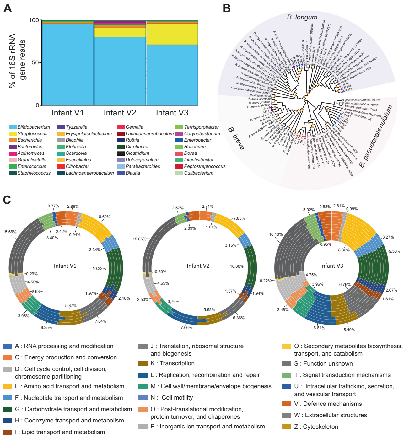
Fig. 1 a Faecal bacterial community profiles of three healthy, full-term infants as determined by 16S rRNA gene sequencing. Paired-end reads were generated using the MiSeq Illumina platform, all data sets were normalised and relative abundance of each bacterial taxa is represented in percentages of number of total reads for the top ten most prevalent genus in each infant. Bar colours represent different genus taxa, and bar lengths signify the relative abundance of each taxon. 16S rRNA bacterial profiles are named according to the sample used for bifidobacteria isolation. V1 at 102 days of age, V2 at 174 days of age, and V3 at 159 days of age. The number of reads obtained by 16S rRNA gene sequencing data for each sample can be found in Table S2.
