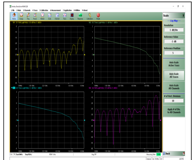
Fig. 2. Screen-shot of VNA measurements of 50 \Omega transmission line.
