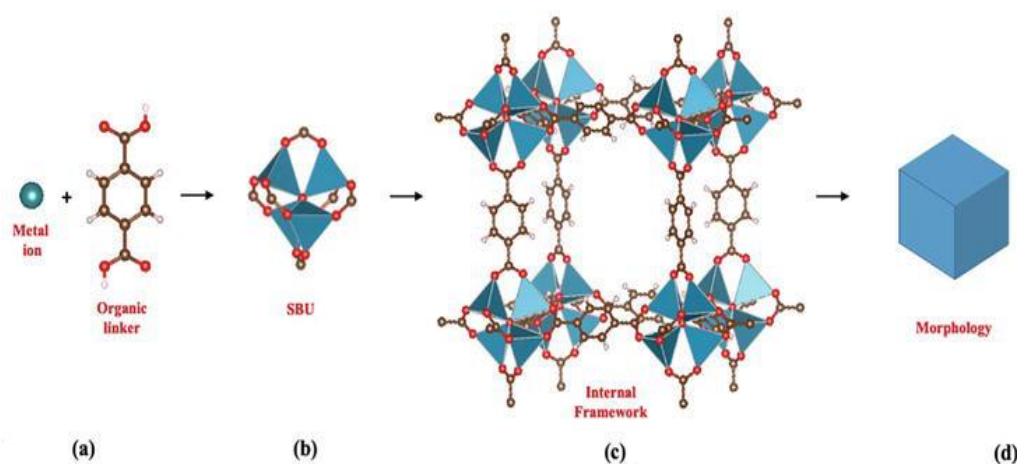
Figure 1.5: MOF-5 structure representation a) metal ion (Zn) and organic linker (Terephthalic acid) b) Secondary Building Unit (SBU) c) MOF- framework formed by coordination of SBUs to organic linker d) Final morphology of MOF-5. Adapted from Inoue, M.; Suzuki, T.; Nakada, M. Asymmetric Catalysis of Nozaki-Hiyama Allylation and Methallylation with a New Tridentate Bis(Oxazolinyl)Carbazole Ligand. J Am Chem Soc 2003 , 125 (5), 1140–1141. 74
