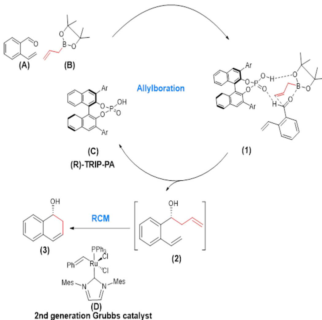
Figure 5.2: Mechanism of the asymmetric allylboration and Ring-Closing Metathesis (RCM)
