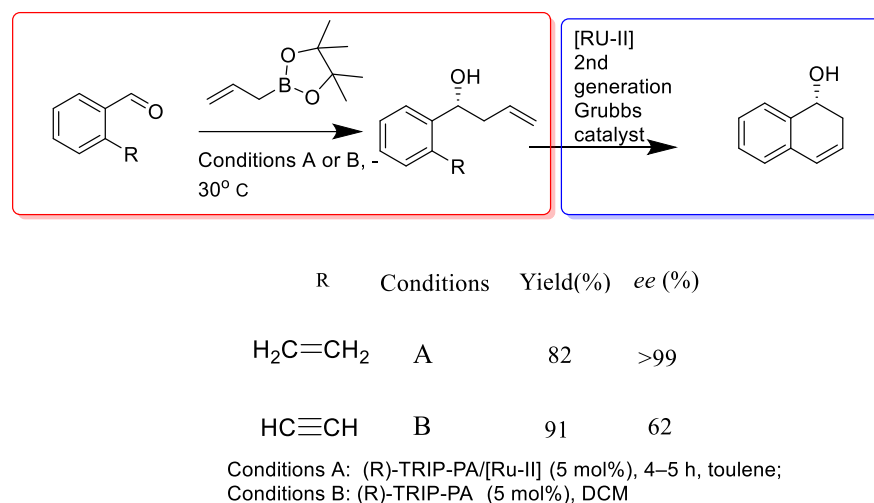
Figure 5.1: Allylboration of alkenes and alkynes catalyzed by BINOL phosphoric acid
