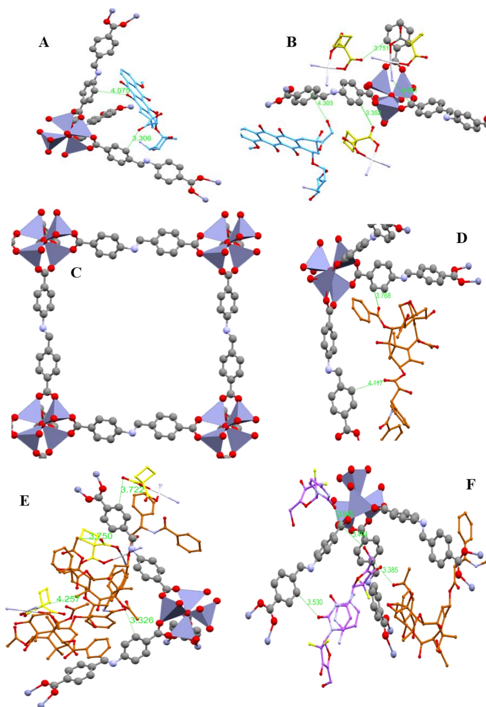
Figure 4.1: Images showing the site of adsorption in NUIG-4. A) DOX; B) DOX-CAR; C) NUIG-4 framework; D) PAL; E) PAL+CAR; F) PAL+GEM. The NUIG-4 atoms are in grey its metal cluster is represented as a blue-coloured polyhedron. DOX, PAL, CAR, and GEM are in the ball and stick representation
