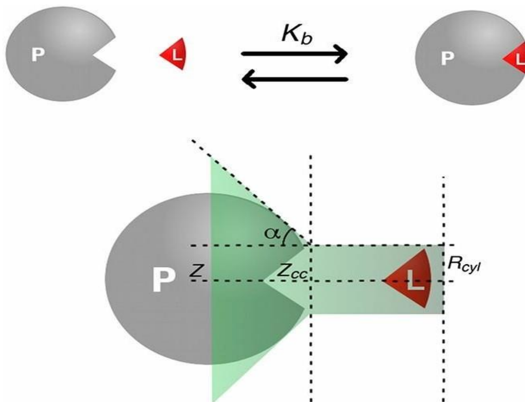
Figure 1.4: Schematic diagram showing the ligand binding to protein and the funnel restraint potential used in funnel metadynamic. Z in the figure is the axis of the binding path of the ligand. z_{cc} represents the distance where the restraint potential changes from cone to cylinder. \alpha -angle represents the cone amplitude and R_{cyl} is the radius of the cylindrical section. The funnel's shape is adjusted by the parameters mentioned above. Adapted from Kou, L. F.; Huang, H. E.; Lin, X. L.; Jiang, X. Y.; Wang, Y.; Luo, Q. H.; Sun, J.; Yao, Q.; Ganapathy, V.; Chen, R. J. Endocytosis of ATB(0,+)(SLC6A14)-Targeted Liposomes for Drug Delivery and Its Therapeutic Application for Pancreatic Cancer. Expert Opin Drug Deliv 2020 , 17 (3), 395–405. 31
