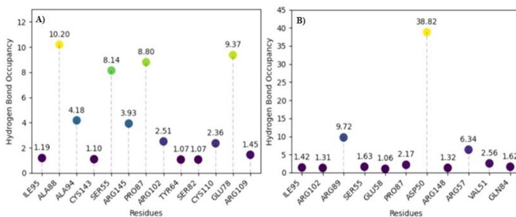
Figure 3.5: Hydrogen bond occupancy percentage calculated during 500 ns molecular dynamics simulation of A) Verbascoside and B) Salvanoic acid protein complexes
