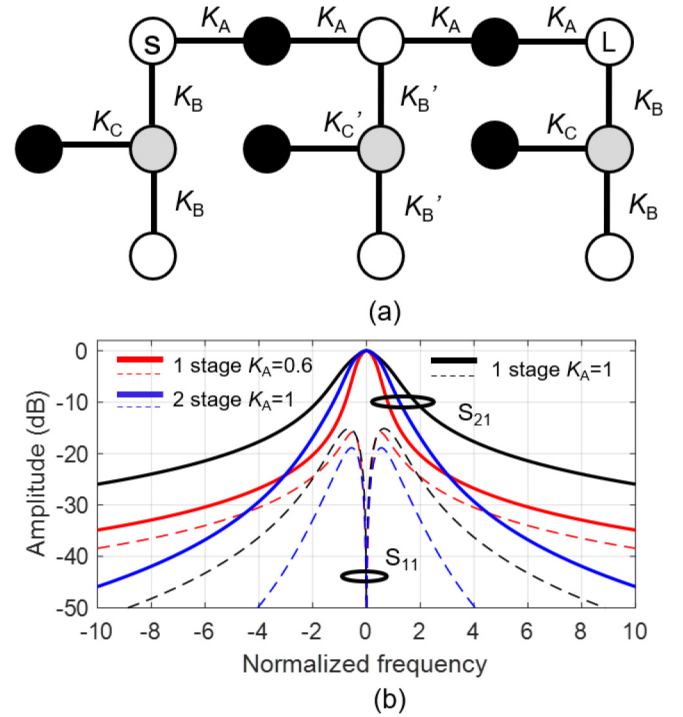
Fig. 2. (a) Normalized CRD of the two-stage quasi-reflectionless BPF. (b) Synthesized power transmission ( S_{21} ) and reflection ( S_{11} ) responses of the one- and two-stage BPFs.
