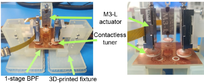
Fig. 5. RF testing setup for the one-stage prototype. A 3D printed fixture was manufactured to assemble the tuners on the BPF.
