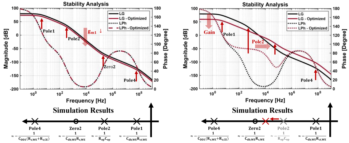
Figure 3.18. The stability analysis for current-mirror based potentiostat.
