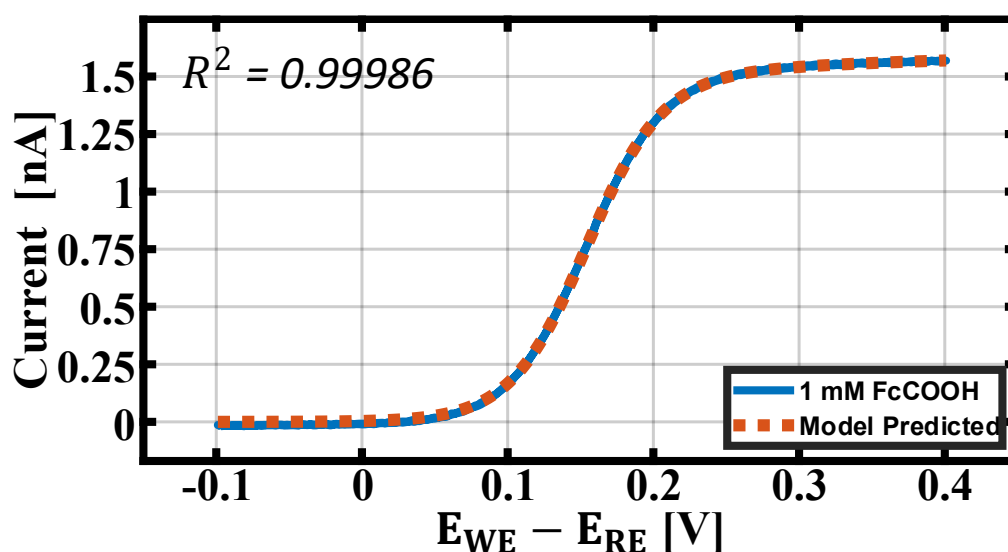
Figure 4.3. The measurement results of CV for one cycle with an UMB electrode sensor in 1 mM FcCOOH dissolved in 10 mM PBS at 25° C, SR = 0.001 V/s, and the Model predicted data.
