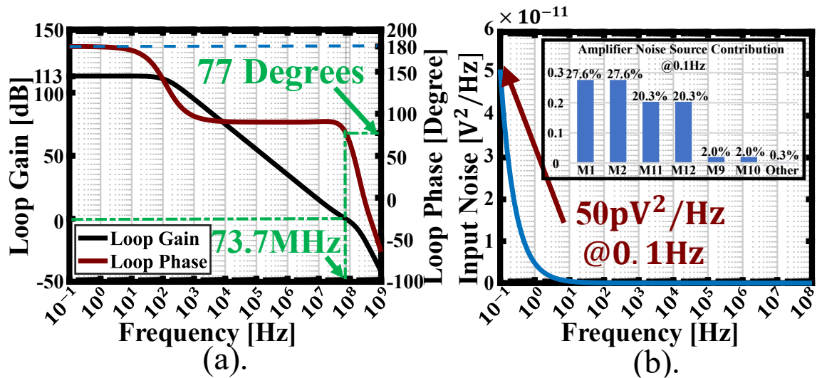
Figure 4.12. (a). Stability analysis, and (b). input-referred voltage noise density spectrum and the noise source contribution of the in-band integrated noise.
