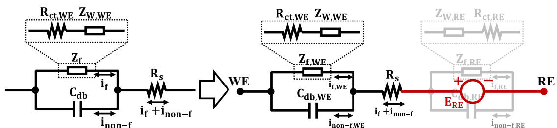
Figure 3.7 The approximated simplified small-signal model for a two-electrode system with tiny current.
