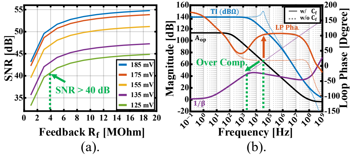
Figure 4.14. (a). The SNR analysis of TIA at a DC bias of 0.125 V, 0.135 V, 0.155 V, 0.175 V and 0.185 V. (b). The stability analysis of TIA with overcompensation. Note that the transimpedance has a unit of Ohm.
