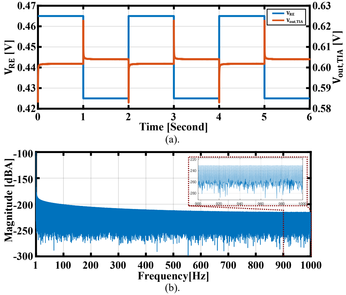
Figure 4.15. The noise analysis considering the FFT demodulation; (a). the simulated time-domain response of the Verilog-A model, with a DC potential ( V_{WE} - V_{RE} ) of 155 mV, and an AC amplitude of 40 mV, and (b). the FFT results of the current, by converting the TIA output with an R_f of 4 M \Omega .
