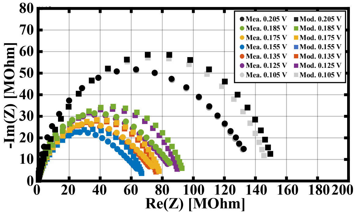
Figure 4.10. EIS measurement results with an amplitude of 10 mV over a frequency range of 0.1 Hz to 100 kHz, vs. Verilog-A model-predicted results from Cadence, on the DC biases of 0.105 V, 0.125 V, 0.135 V, 0.155 V, 0.175 V, 0.185 V and 0.205 V over the same frequency range.
