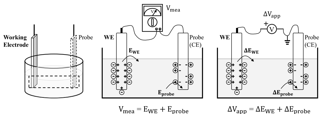
Figure 2.4. The single-electrode system: sensing or applying an electrode potential, where a probe of an instrument serving as a CE.
