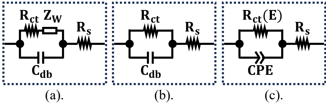
Figure 4.9. Models of electrochemical sensor electrode-electrolyte interfaces: (a). Randle's Model. (b). Randle's Model with Warburg Impedance omitted. (c). Model with CPE, where R_{ct} is dynamic.
