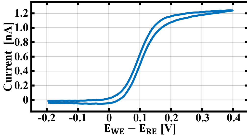
Figure 4.4. The CV measurement result under experimental conditions of 1 mM FcCOOH dissolved in 10 mM PBS at 25° C, with a SR of 50 mV/s.
