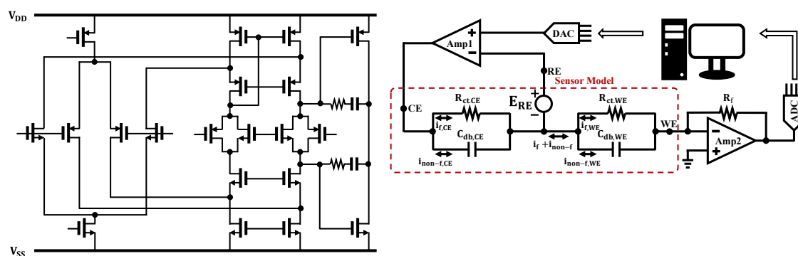
Figure 3.13. The rail-to-rail folded-cascode with floating class AB controlled output stage [78]
