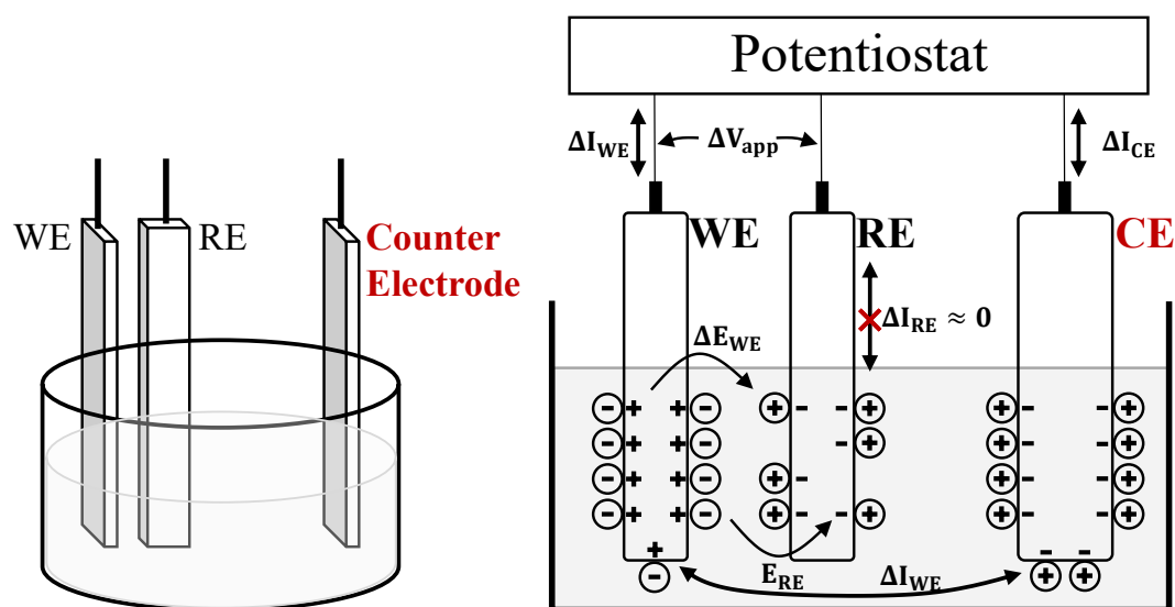
Figure. 2.6. The three-electrode sensor system, with a CE for conducting the current.
