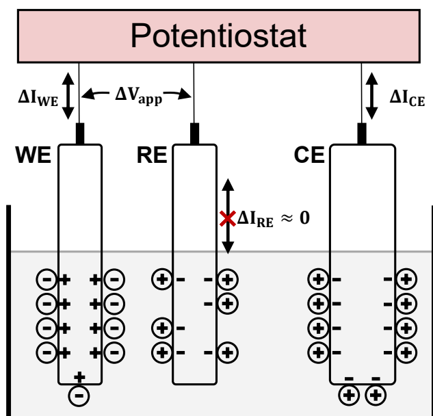
Figure 3.10. The diagram of a three-electrode electrochemical system.
