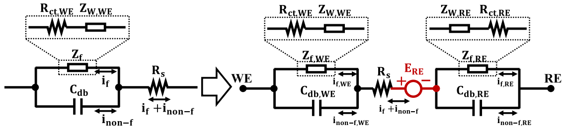
Figure 3.6. The model of the two-electrode sensor system, with a DC voltage source representing the reference electrode potential.
