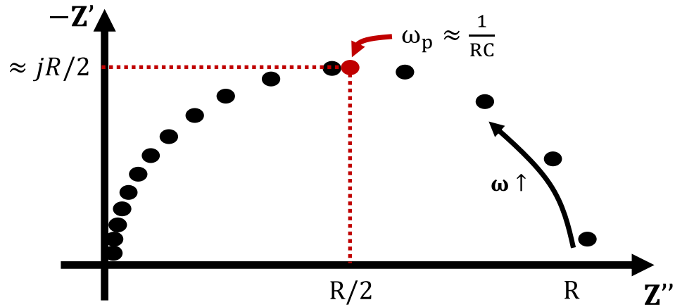
Figure 2.9. The Nyquist diagram of a RC complex impedance.
