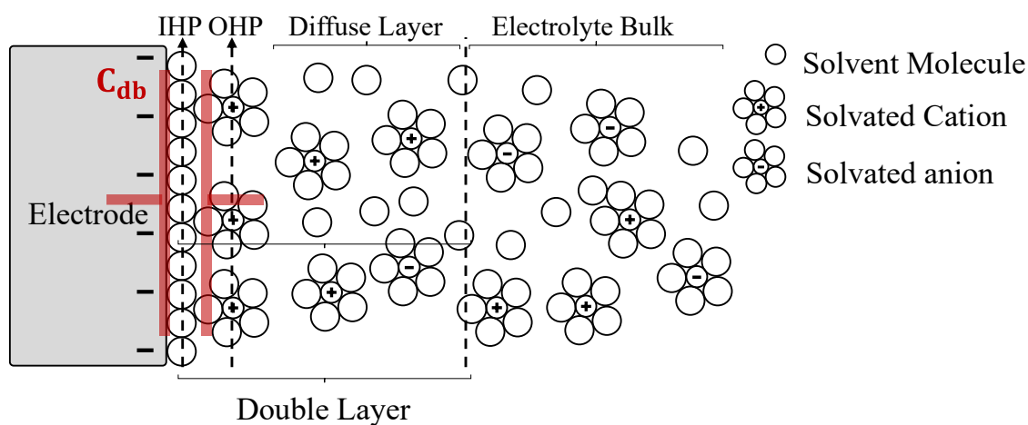
Figure 3.3 The equivalent double-layer capacitor model at the electrode-electrolyte interface.
