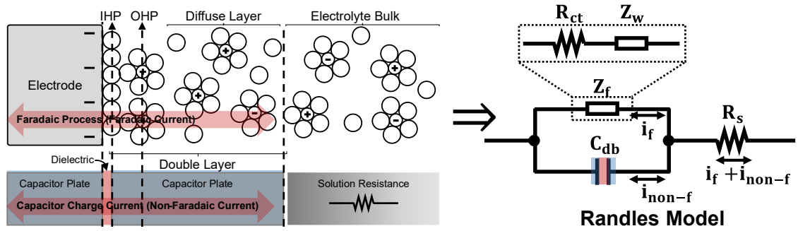
Figure. 3.5. Equivalent Small-signal Models for Single Electrode – Randles Model
