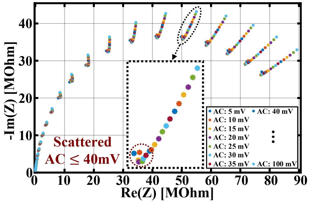
Figure 4.6. EIS results of UMB electrode with AC amplitude increasing from 5 mV to 100 mV, with an incremental step of 5 mV at 0.1 V DC potential.
