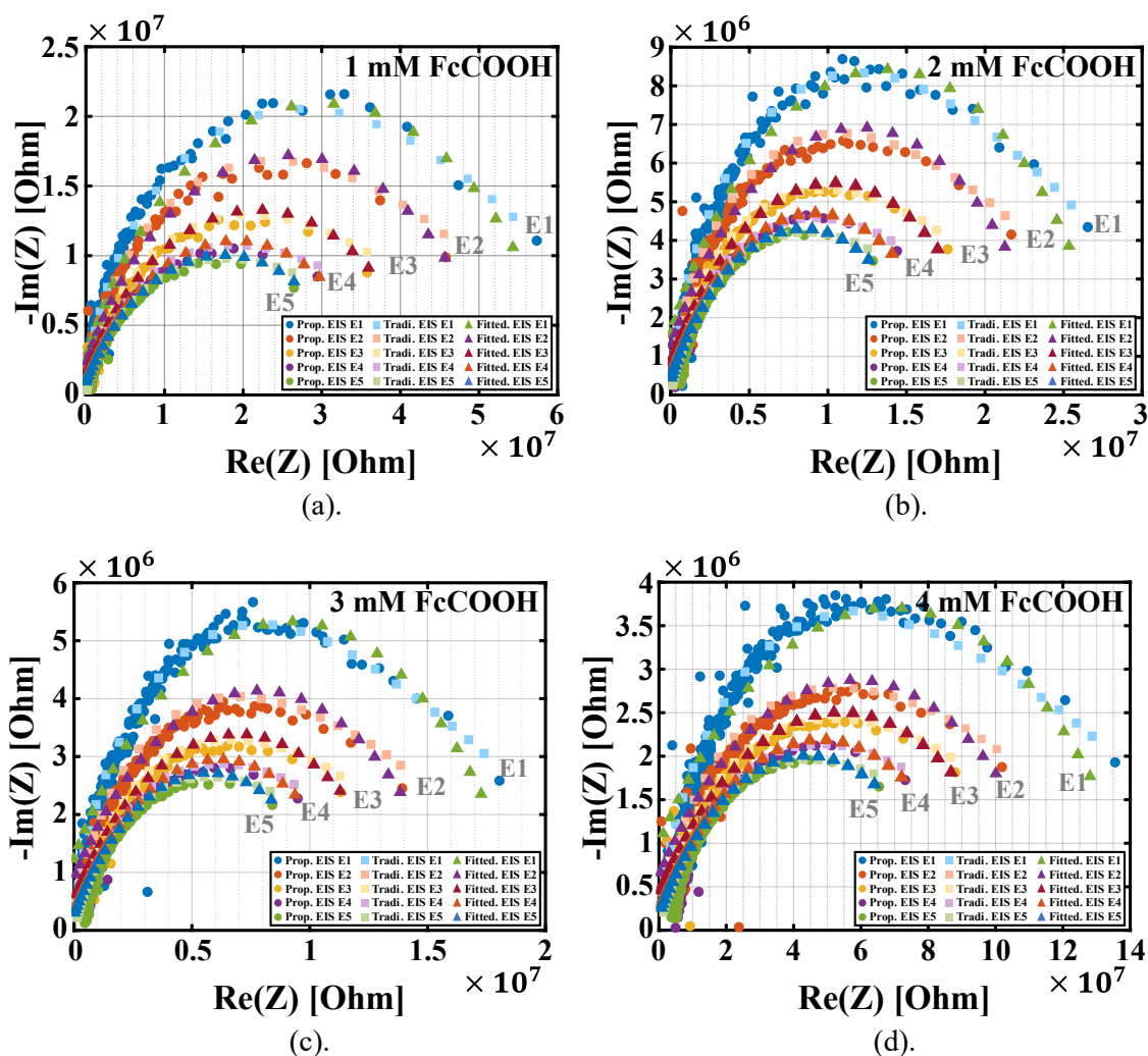
Figure 4.29. The comparison of EIS results of the square wave EIS, the traditional EIS performed by AutoLab, and the EIS optimized fitted model. The square wave EIS and the traditional EIS employ the same AC and DC conditions as indicated in Figure 4.26.
