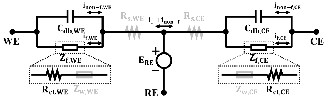
Figure. 3.9 The AC impedance model of UMB three-electrode sensor system for electrochemical sensor interface design.
