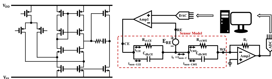
Figure 3.12 A two-stage folded-cascode amplifier [72]
