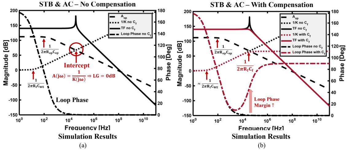
Figure 3.15 The stability analysis for TIA
