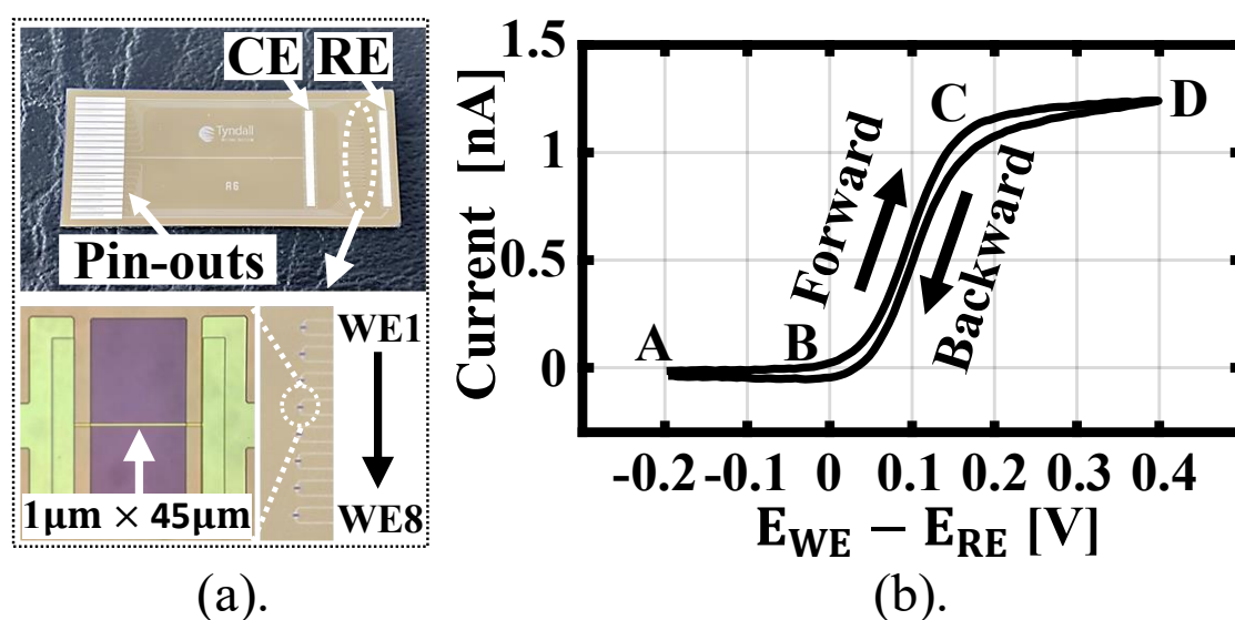
Figure 4.2. (a). A silicon wafer substrate with eight individual UMB electrodes. (b). The measurement results of CV with an UMB electrode sensor in 1 mM FcCOOH dissolved in 10 mM PBS at 25° C, SR = 50 mV/s.
