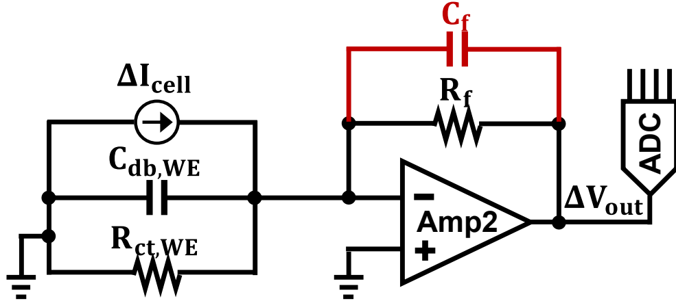
Figure. 3.14. The equivalent model for stability analysis of a TIA
