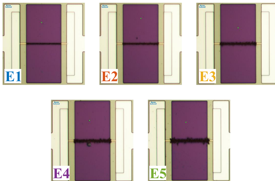
Figure 4.21. Microscopic images of five electrodes with different deposited thicknesses of gold.
