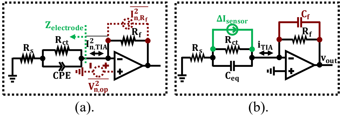
Figure 4.13. The equivalent models for TIA design. (a). The simplified equivalent model with noise source contributions, and (b). the equivalent model for analyzing stability and bandwidth.
