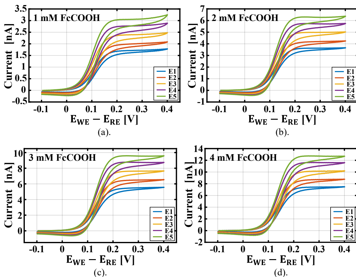
Figure 4.22. The CV results performed by AutoLab in (a). 1 mM FcCOOH, (b). 2 mM FcCOOH, (c). 3 mM FcCOOH, and (d). 4 mM FcCOOH, in a 10 mM PBS supporting electrolyte at 25°, with a SR of 50 mV/s from -0.1 V to 0.4 V, showing different electrode characteristics for the electrochemical validation.
