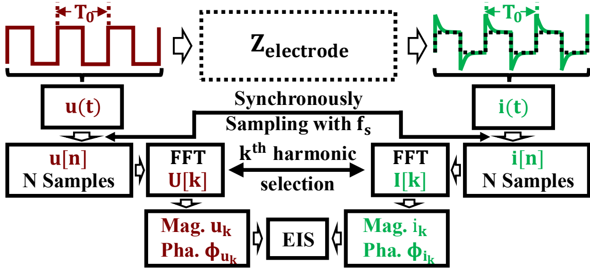
Figure 4.7. The system level diagram of the proposed square-wave EIS.
