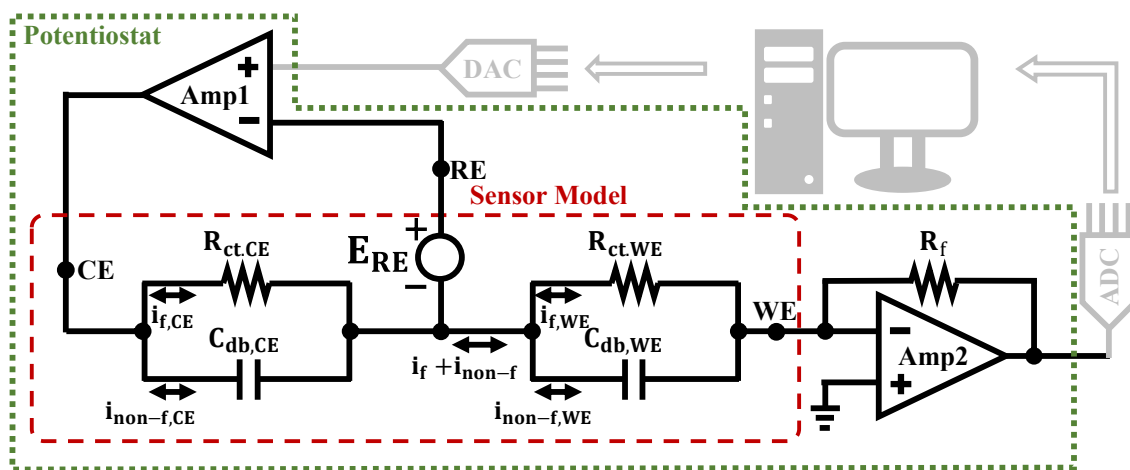
Figure. 3.11. Op-amp and TIA-based potentiostat
