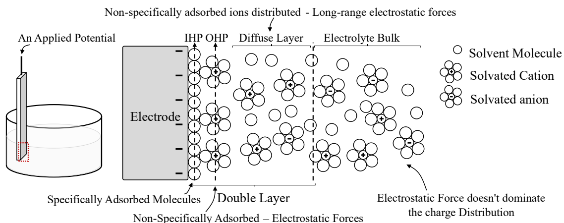
Figure 3.1. The electrode-electrolyte interface for a single electrode.
