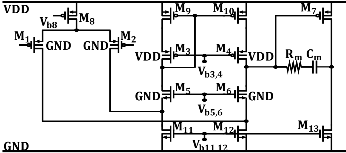
Figure 4.11. PMOS-input folded-cascode amplifier topology, complemented by a CS output stage with Miller compensation.
