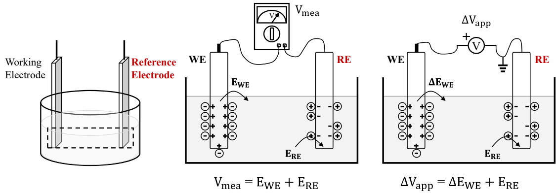
Figure 2.5. The two-electrode system: sensing or applying an electrode potential, where the probe is replaced with an RE, providing a constant reference electrode potential.
