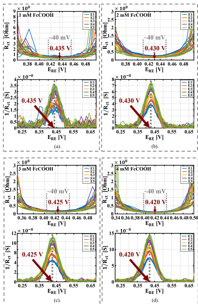
Figure 4.26. The determination of AC and DC conditions for square-wave EIS across a). 1 mM FcCOOH, b). 2 mM FcCOOH, c). 3 mM FcCOOH, and d). 4 mM FcCOOH, in a 10 mM PBS supporting electrolyte at 25°. The DC bias of the sensor is chosen where the conductance of the sensor reaches minimum, namely, the half potential, and the AC amplitude is chosen to be 40 mV as mentioned in Section 4.2.3, where the sensor working in a linear region.
