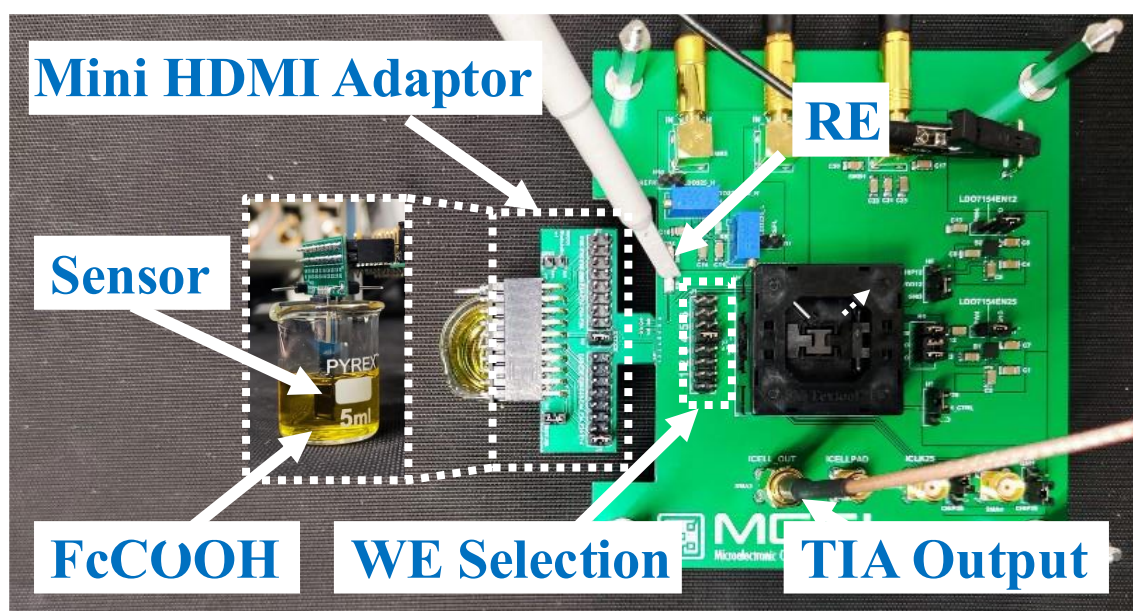
Figure 4.24 The PCB setup for chemistry test with deposited UMB electrodes.
