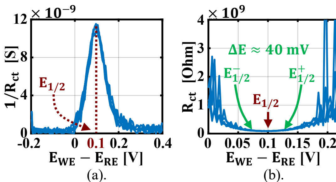
Figure 4.5. The determination of the conditions where R_{ct} is an LTI component. (a). The conductance of the UMB electrode sensor is potential-dependent. (b). Determination of the practical time-invariant linear region.
