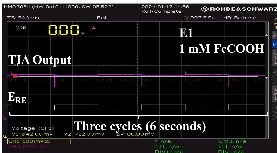
Figure 4.27. The time-domain results of the sensor input and TIA output for E1.
