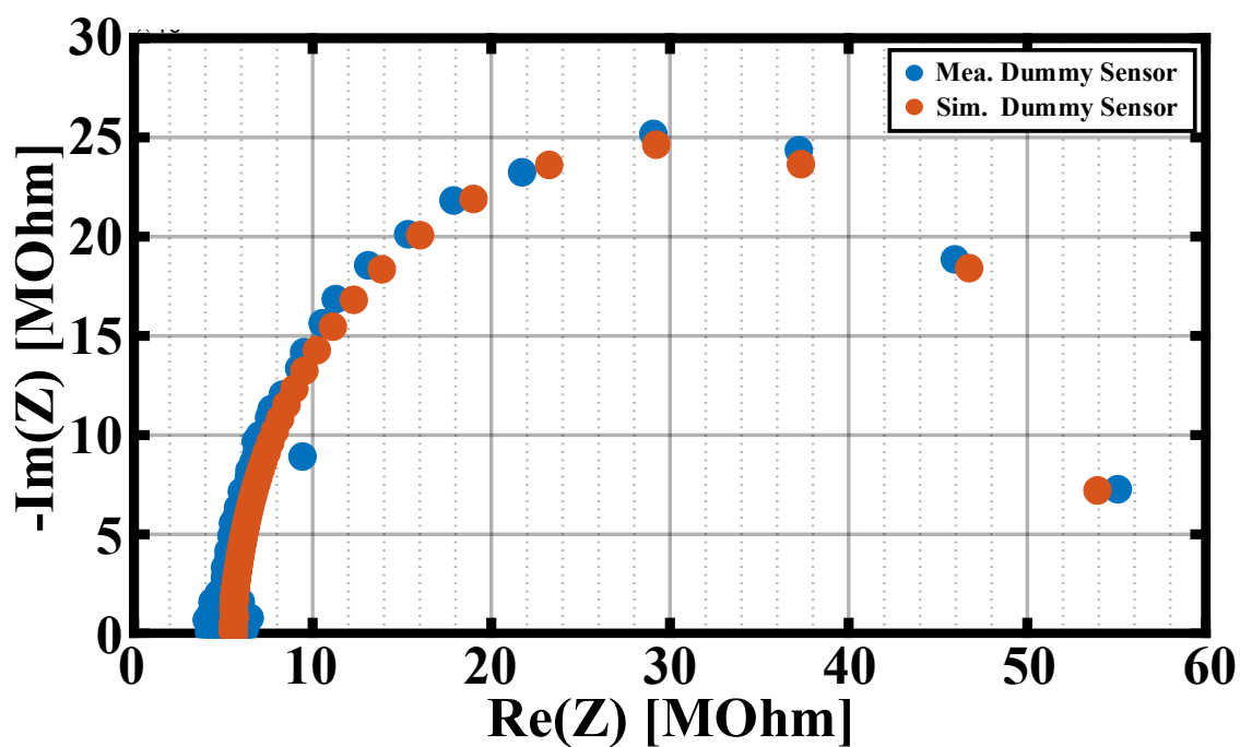
Figure 4.20. The chip-tested results of square-wave EIS and simulated results of a dummy sensor, with an R_{ct} = 50 MOhm, and a C_{eq} = 1 nF.
