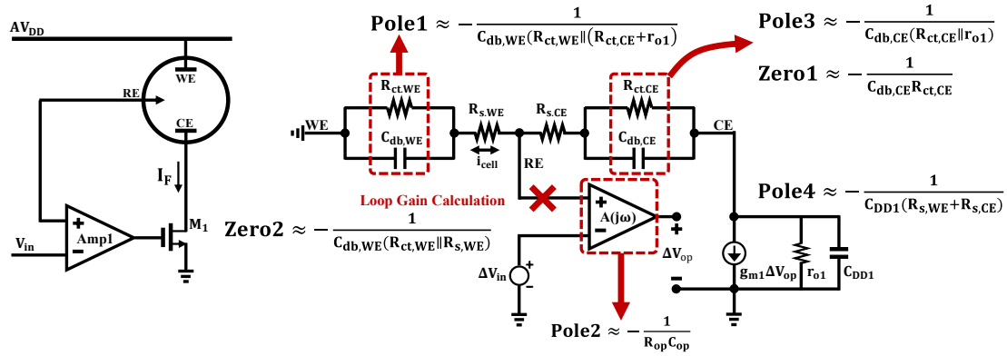
Figure 3.17. The equivalent small-signal model for stability analysis [83].
