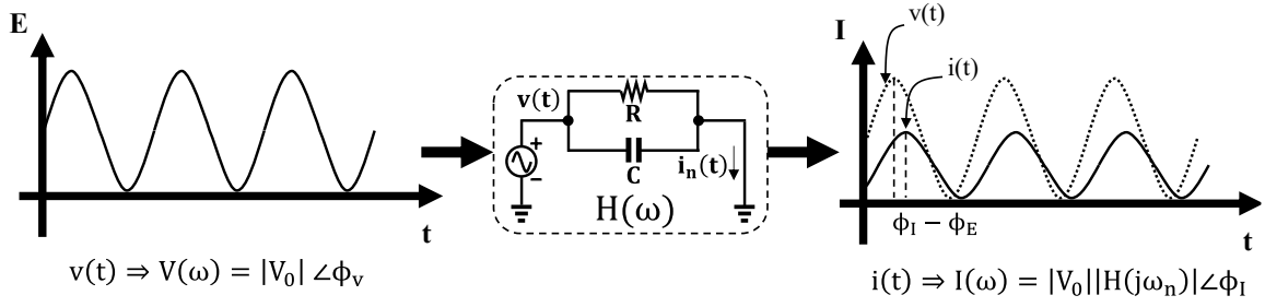
Figure. 2.8. The EIS for an RC complex impedance.
