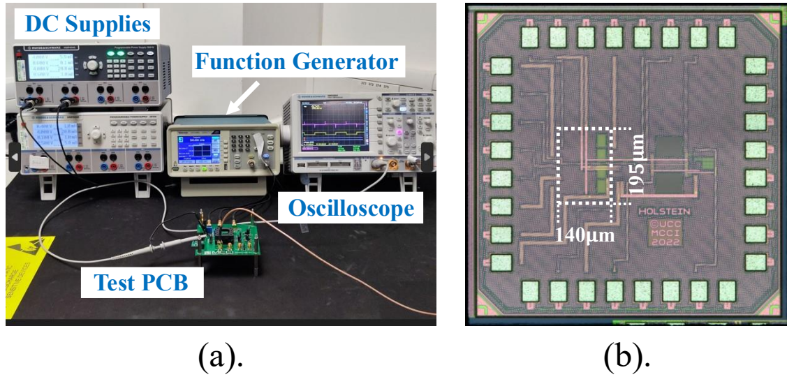
Figure 4.16. The measurement setup and the die micrograph: (a). The test setup, and (b). the die micrograph.
