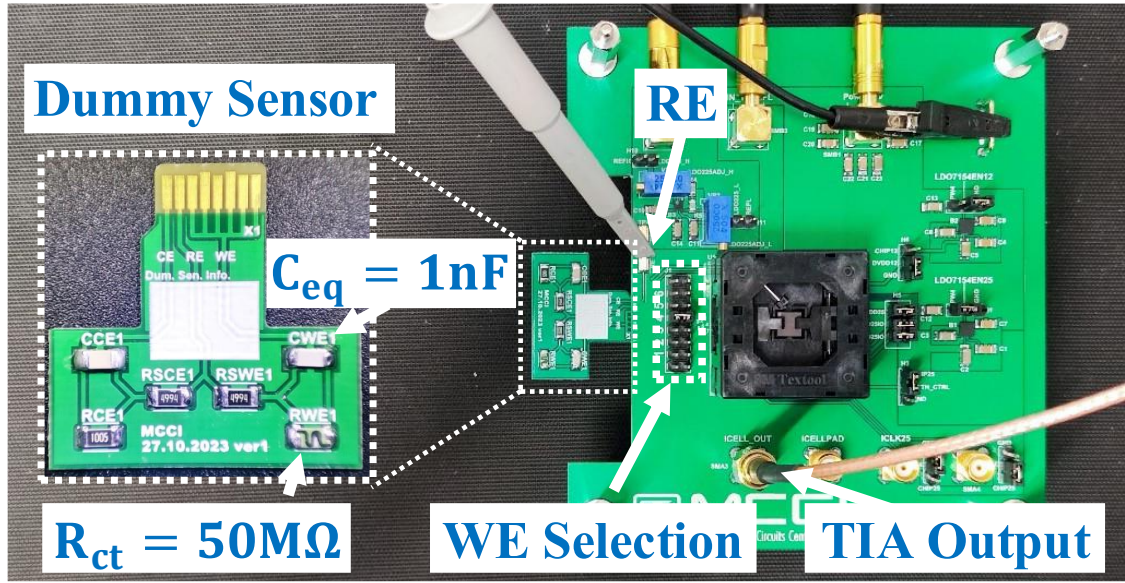
Figure 4.17. The PCB setup for electrical validation, with an R_{ct} = 50 \text{ MOhm} , and a C_{eq} = 1 \text{ nF} .
