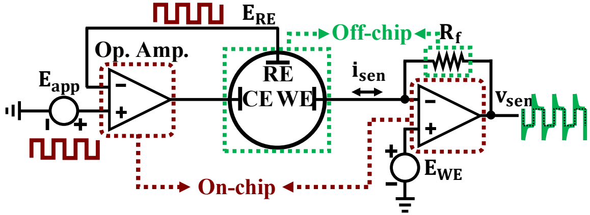
Figure 4.8. The block diagram of the circuit for the proposed square-wave EIS.
