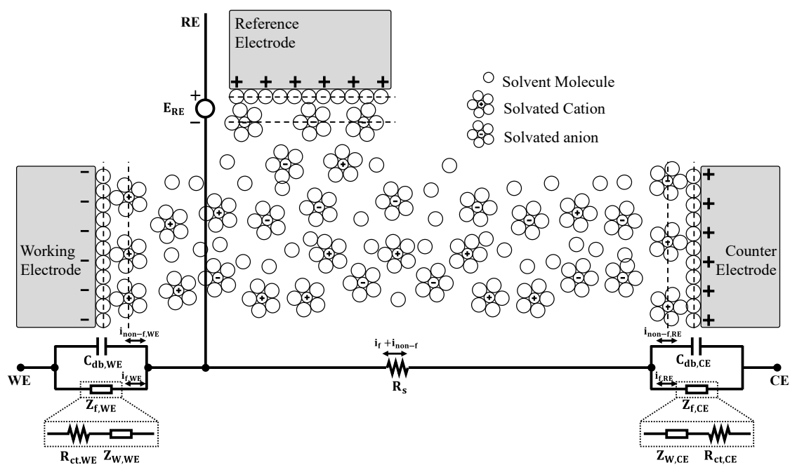
Figure 3.8. The equivalent small-signal model of a three-electrode electrochemical sensor, with the comparison of sensor electrode-electrolyte interface of each electrode.
