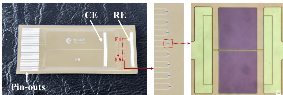
Figure 2.3. The UMB electrode electrochemical sensor with Counter Electrode (CE), Reference Electrode (RE), Mini HDMI compatible pin-outs, and the microscopic photo of the working electrode.
