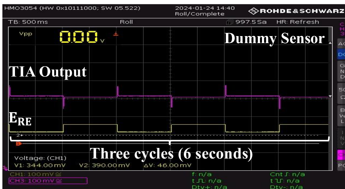
Figure 4.18. The time-domain results of the sensor input and TIA output for a dummy sensor, with an R_{ct} = 50 \text{ MOhm} , and a C_{eq} = 1 \text{ nF} .
