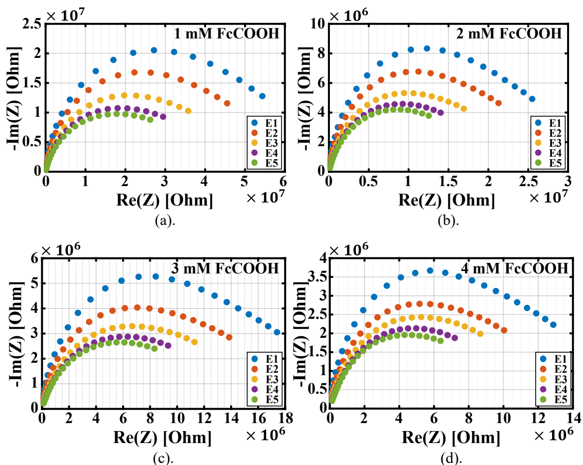
Figure 4.23. The EIS results performed by AutoLab in (a). 1 mM FcCOOH, (b). 2 mM FcCOOH, (c). 3 mM FcCOOH, and (d). 4 mM FcCOOH, in a 10 mM PBS supporting
