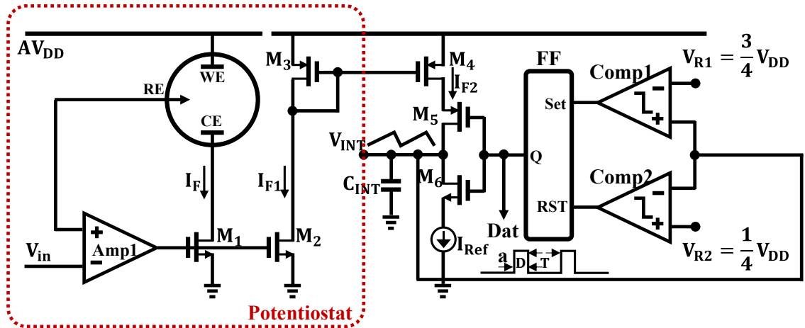
Figure 3.16 The current mirror-based potentiostat and current-to-frequency converter
