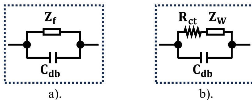
Figure 3.4. The equivalent model of an electrode-electrolyte interface: (a) an equivalent model with a capacitor and faradaic impedance in parallel; (b) equivalent with faradaic impedance represented by a charge-transfer resistance and the WI.
