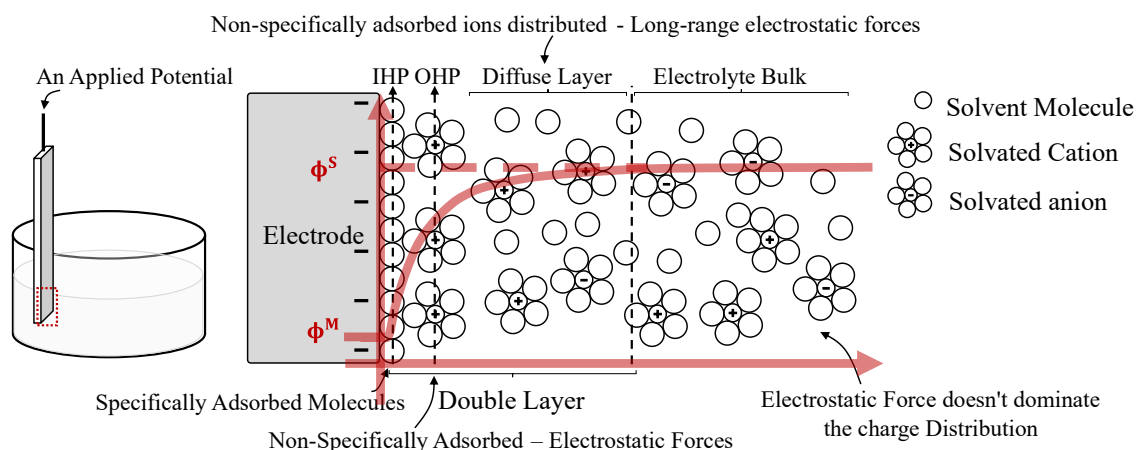
Figure 3.2. The electrode-electrolyte interface and the electrode potential.
