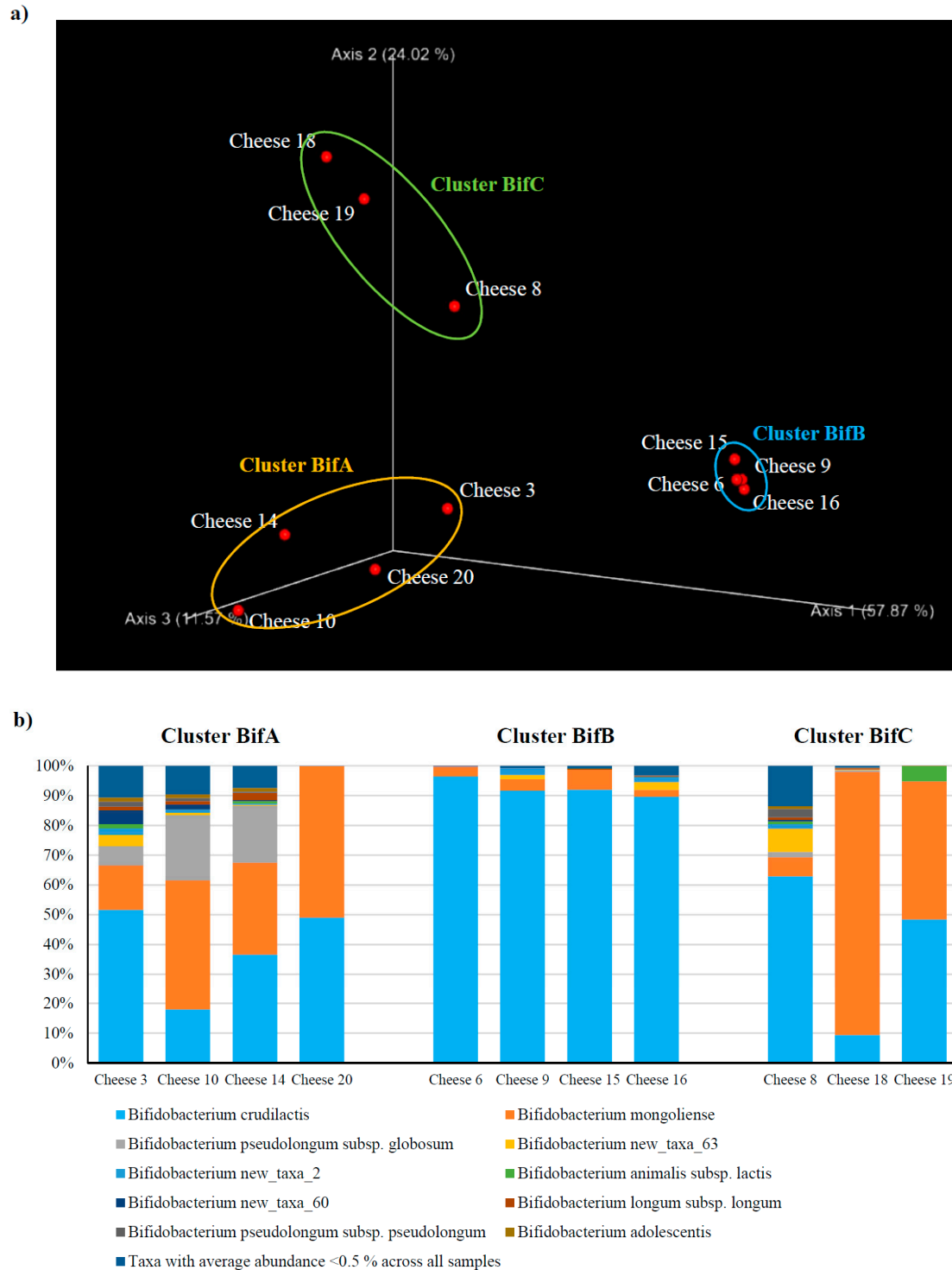
Figure 2. Taxonomic dissection of the bifidobacterial population harbored by raw cheese. (a) shows a PCoA representation of the beta-diversity analysis performed for bifidobacterial ITS data at species level using the Bray–Curtis index. (b) displays a bar plot representation of the bifidobacterial population at the species level observed in 11 ‘raw’ cheese samples (i.e., those for which we could obtain data). Only taxa with an average abundance >0.5% are shown.
