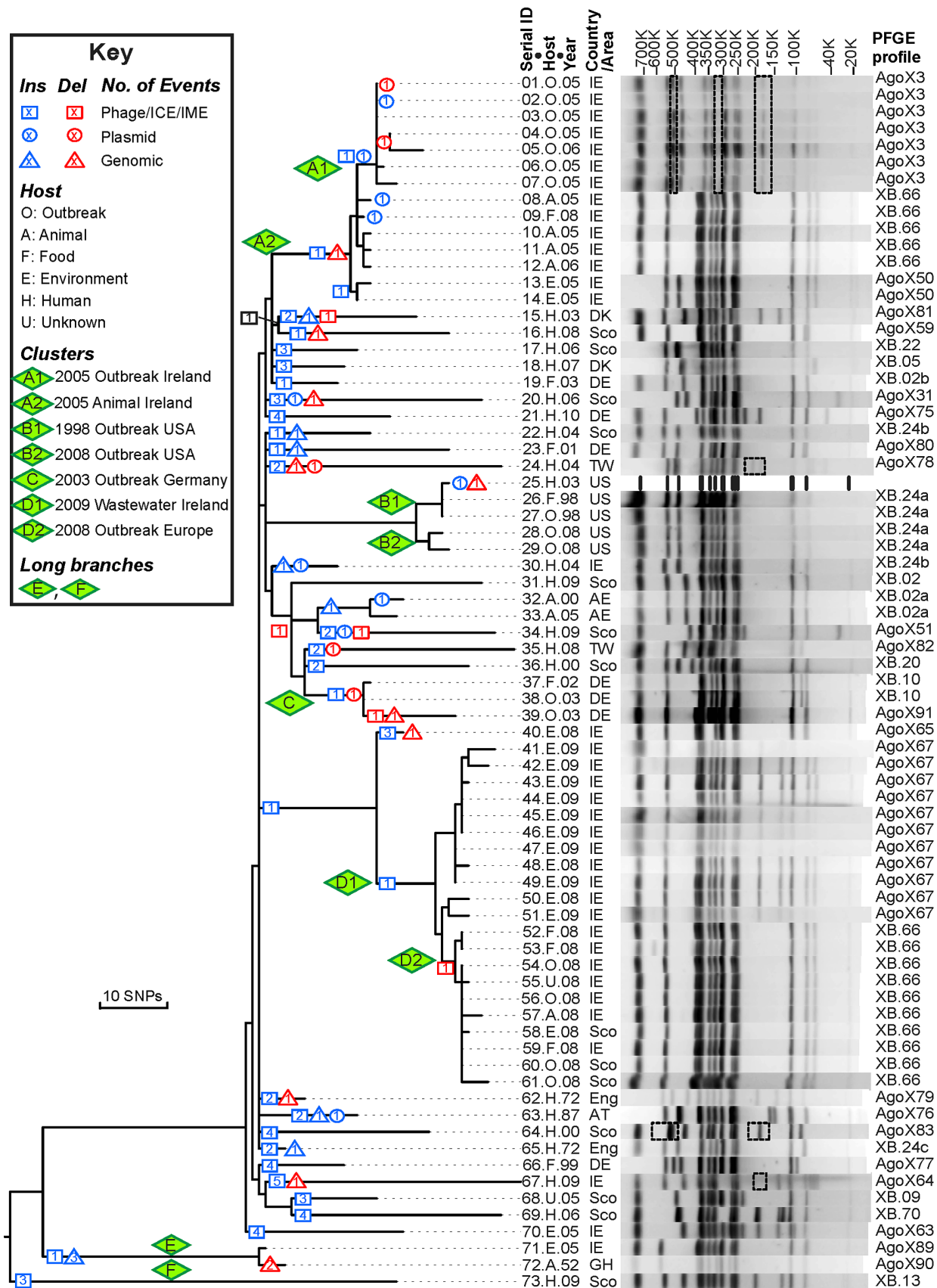
Figure 1. Genealogy of 73 Agona genomes based on SNPs and indels versus PFGE patterns. Left: Maximum parsimony genealogy inferred from 846 non-homoplasic, non-recombinant, non-mobile, non-repetitive core SNPs. The numbers of independent insertions or deletions of mobile
