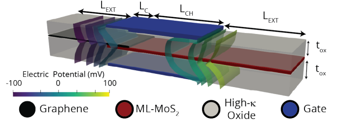
Fig. 1. Schematic of the double-gate device geometry studied. Top and bottom oxides are high- \kappa ( \epsilon_r = 25 ) with thickness t_{ox} = 3 nm. Source and drain extensions of length L_{EXT} = 15 nm are explicitly included in the self-consistent simulation loop. Top and bottom gates span the length of the ML-MoS 2 channel L_{CH} = 15 nm, and the length of the vertical contact L_C = 5 nm. Periodic boundary conditions are applied along the width direction. Overlaid contour surfaces correspond to electric potential for V_{GS} \approx V_{Th} .
