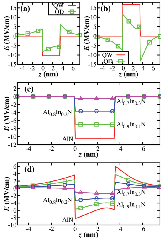
FIG. 3. (Color online) Built-in field along the c axis for (a) GaN/AlN and (b) GaN/InN QD and QW. (c) Built-in field along the c axis for GaN/ \text{Al}_x\text{In}_{1-x}\text{N} QW and (d) QD, as the barrier composition is varied from x = 1 to x = 0.7 . QW and QD of typical dimensions (well: height h = 3.5 nm; truncated-cone dot: base radius R_b = 8 nm, top radius R_t = 2 nm and height h = 3.5 nm).
