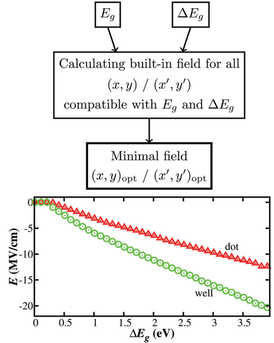
FIG. 6. (Color online) (top) Flux diagram explaining how, for a certain combination of E_g and \Delta E_g at room temperature, the compositions of the \text{Al}_x\text{In}_y\text{Ga}_{1-x-y}\text{N}/\text{Al}_{x'}\text{In}_{y'}\text{Ga}_{1-x'-y'}\text{N} system that minimize the built-in field are obtained and (bottom) smallest built-in field that can be obtained for a QW and a QD system where E_g = 2.25 eV as the bandgap difference \Delta E_g between the barrier and well (or dot) increases.
