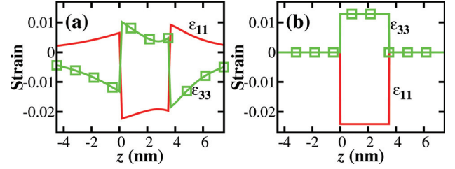
FIG. 2. (Color online) (a) Strain components \varepsilon_{11} and \varepsilon_{33} (open squares) through the center of a QD along the z direction (parallel to c -axis) for a GaN/AlN truncated-cone shaped dot with height h = 3.5 nm, base radius R_b = 8 nm (located at z = 0 ) and top radius R_t = 2 nm (located at z = h ) and (b) for a QW of the same height and composition.
