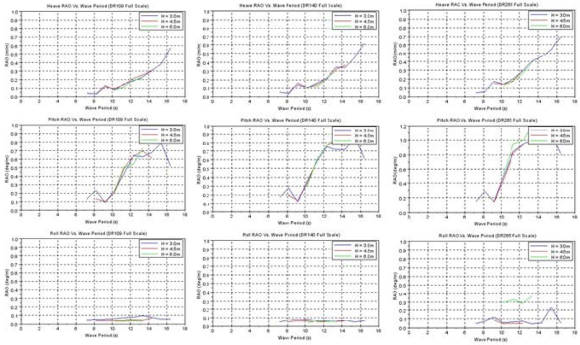
Figure B.7: Primary motion characteristics, heave, pitch and roll, for the OWC array platform for DR109, DR140 and DR265
