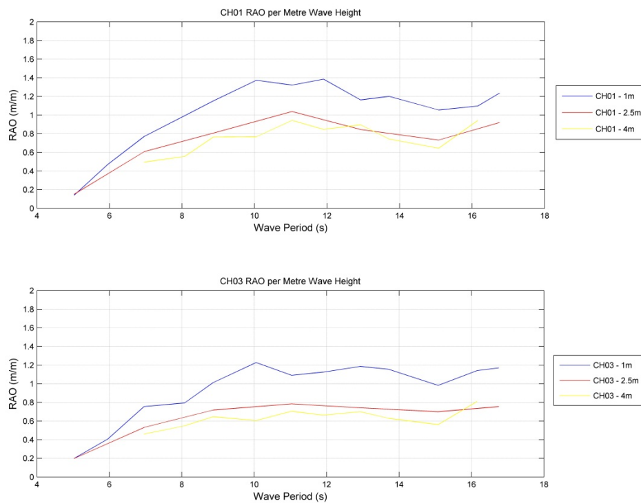
Figure D.17: Chamber 1&amp;3 Water Surface Elevation RAOs
