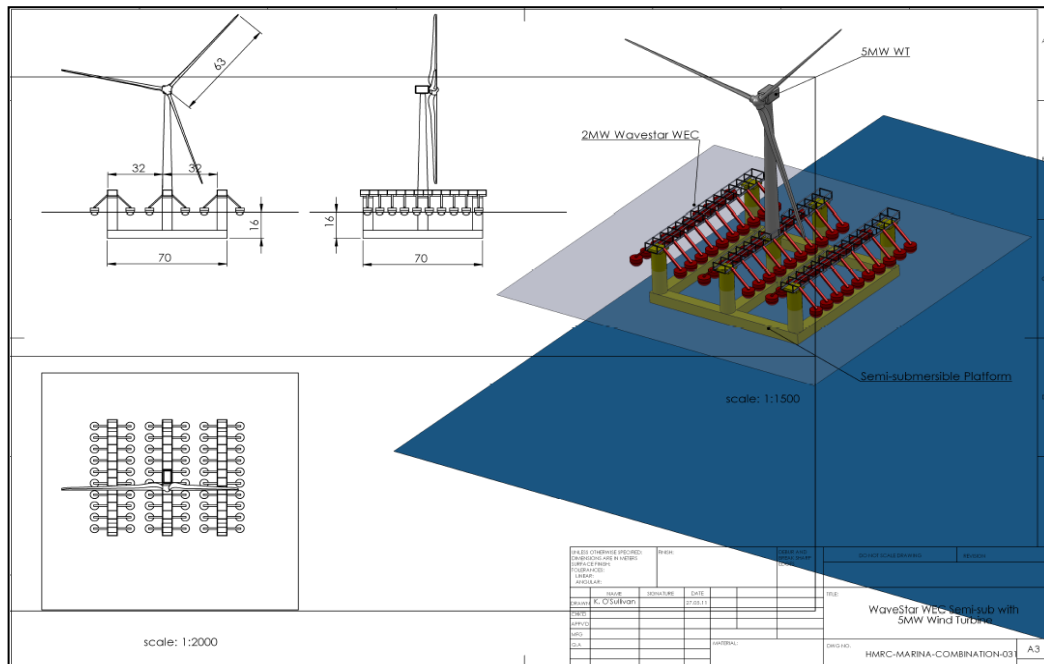
Figure 4-19: Combined Floating Wind/Wave Energy Platform analysed
