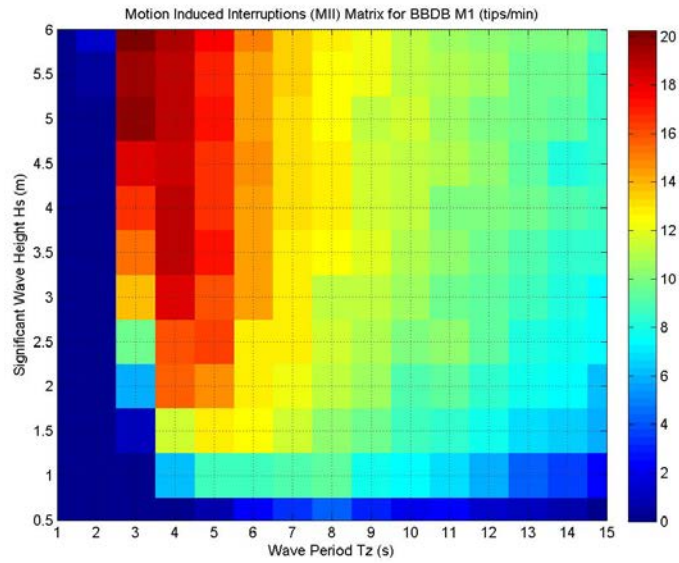
Figure 3-63: MII Events for the BBDB M1 Device
