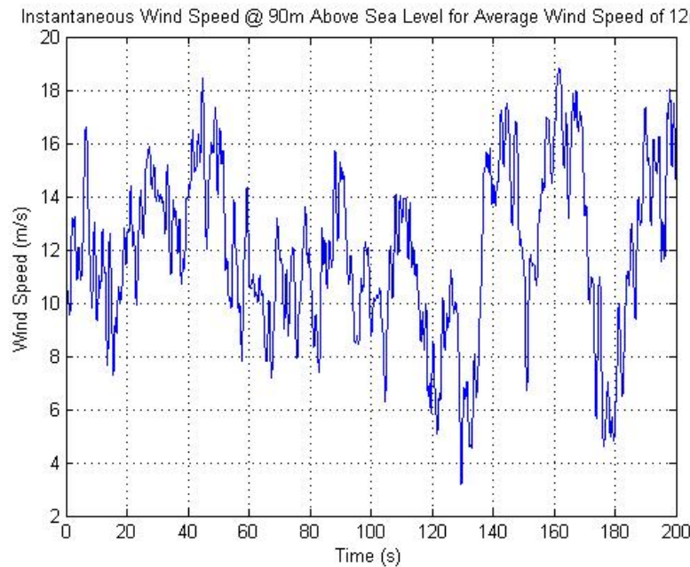
Figure 3-6: Sample Instantaneous Wind Speed at Hub Height of the Turbine
