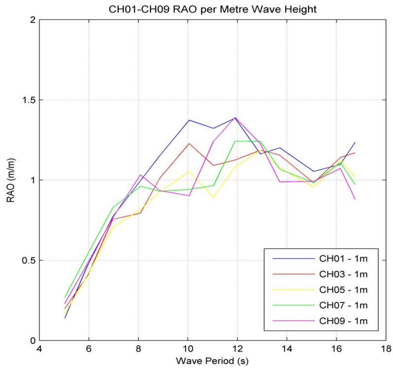
Figure 5-42: Delta OWC Array Chambers 01-09 RAO
