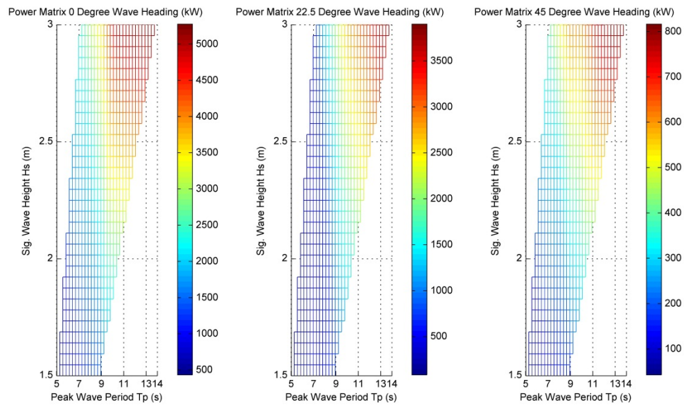
Figure D.26: Prototype Absorbed Power Matrices for the Delta OWC Array Platform for Varying Incident Wave Direction in Panchromatic Waves
