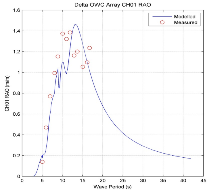
Figure 5-48: Delta OWC Array Chamber 01 RAO Measured Vs Modelled
