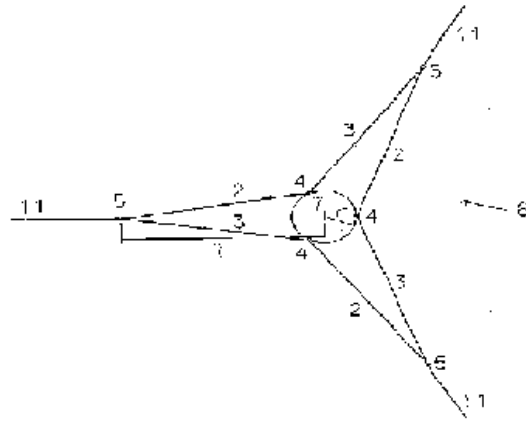
Figure 2-53: The Spar Floating Wind Turbine and Delta Mooring Line Concept ([76], [77])
