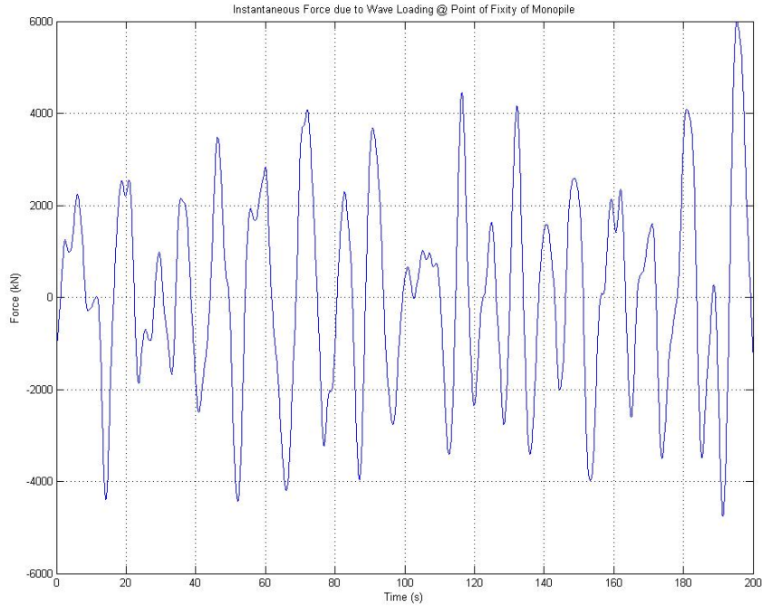
Figure 3-4: Sample Instantaneous Lateral Force at the Point of Fixity of the Monopile from Wave Loading
