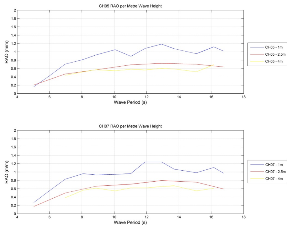
Figure D.18: Chamber 5&amp;7 Water Surface Elevation RAOs
