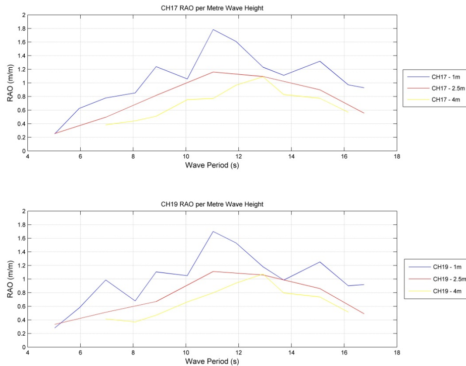
Figure D.20: Chamber 13&15 Water Surface Elevation RAOs
