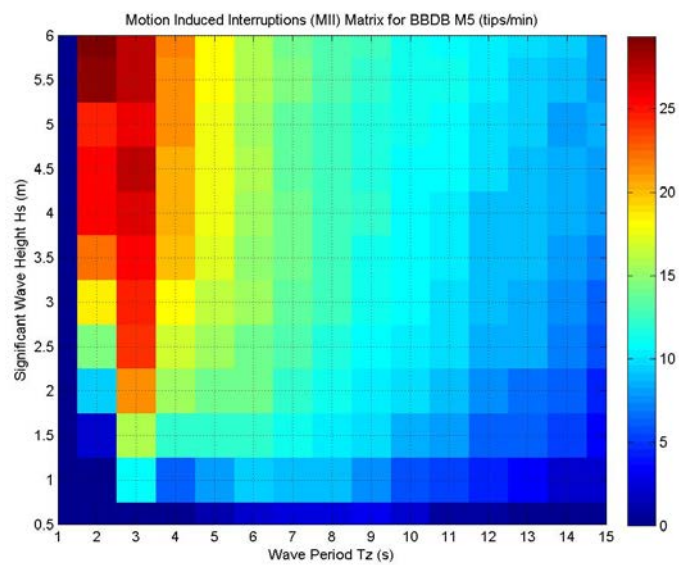
Figure 3-64: MII Events for the BBDB M5 Device
