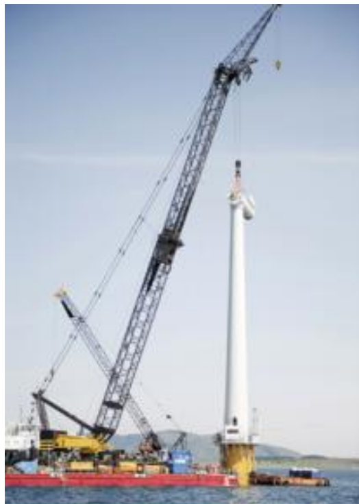
Figure 2-56: Hywind foundation during wind turbine installation
