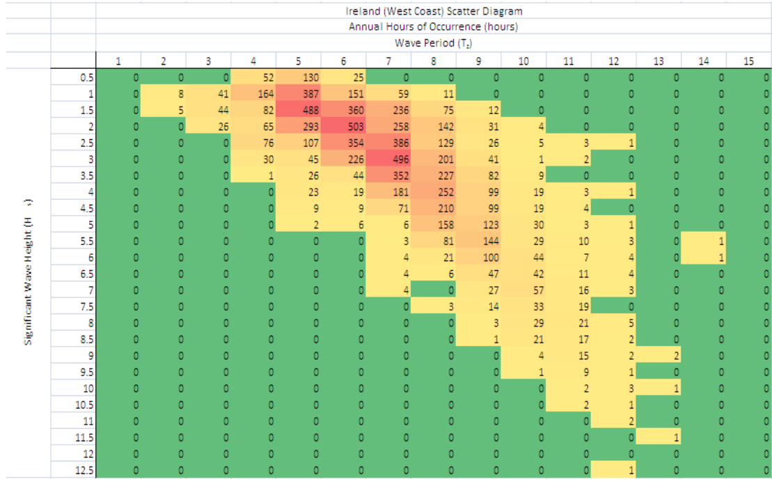
Figure 4-18: Measured Scatter Diagram for the West Coast of Ireland
