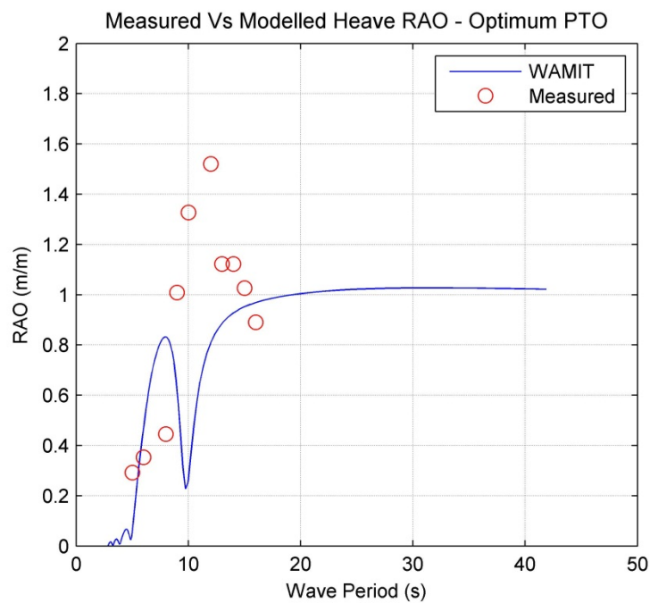
Figure 3-43: Heave RAO for BBDB M1 Numerical and Physical Modelling Comparison
