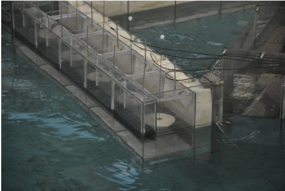
Figure D.7: Float, guides and Qualysis marker arrangement in the chamber
