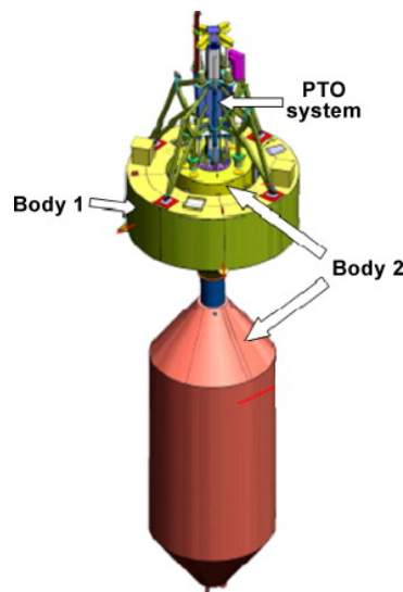
Figure 2-21: Wavebob Concept Configuration
