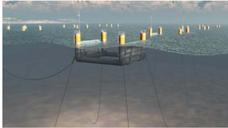
Figure 2-38: Initial Langlee Device
