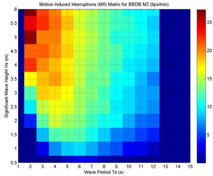
Figure 3-65: MII Events for the BBDB M2 Device
