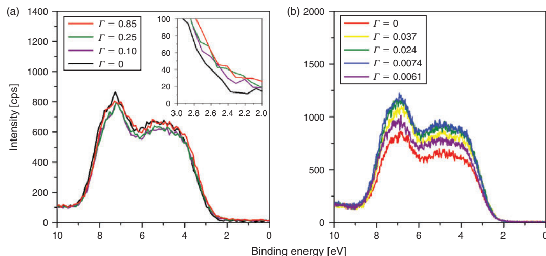
Fig. 4. Valence-band X-Ray photoelectron spectroscopy (XPS) spectra for \text{FeO}_x(I)/\text{TiO}_2 (a) and \text{SnO}_2(I)/\text{TiO}_2 (b).
