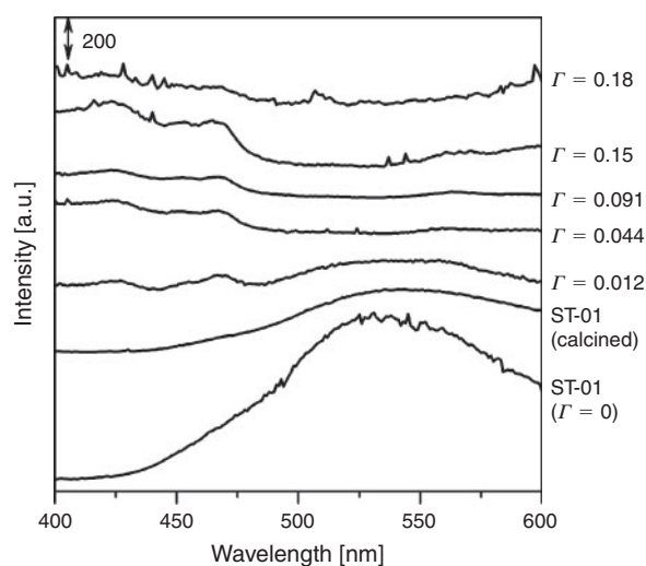
Fig. 5. Photoluminescence spectra of \text{FeO}_x(I)/\text{TiO}_2 at 77 K: excitation wavelength = 320 nm.
