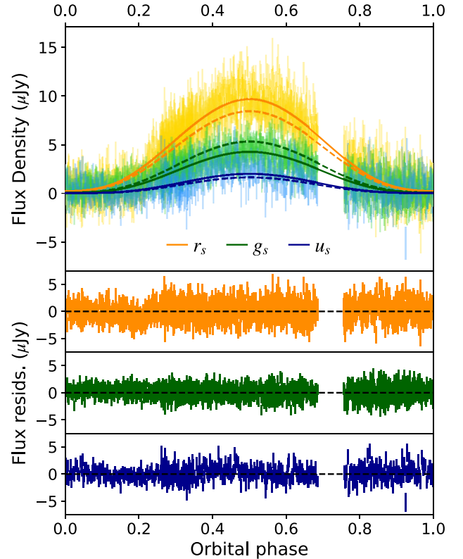
Figure 3. Optical light curves (points), Icarus model fits (solid lines) and residuals (bottom panels) for PSR J1346–2610 from ULTRACAM data.
