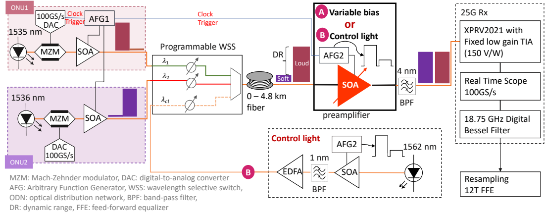
Figure 4.5: Experimental setup for high-speed burst-mode traffic analysis with SOA preamplified receiver performing optical equalisation using two schemes, (A) variable bias, and (B) control light injection.
