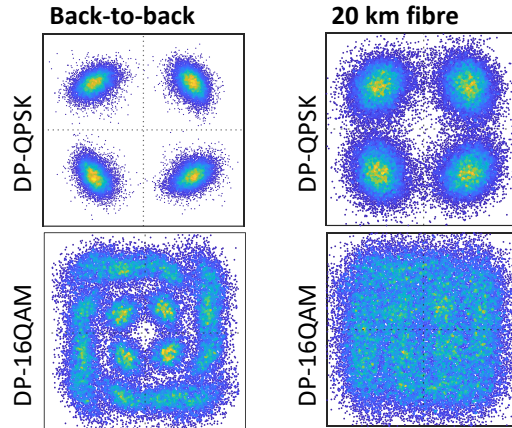
Figure 5.8: Constellation diagrams for both modulation formats measured at an SOA input power of 0 dBm and an LO power of -3 dBm, comparing the back-to-back configuration with 20 km fibre transmission.
