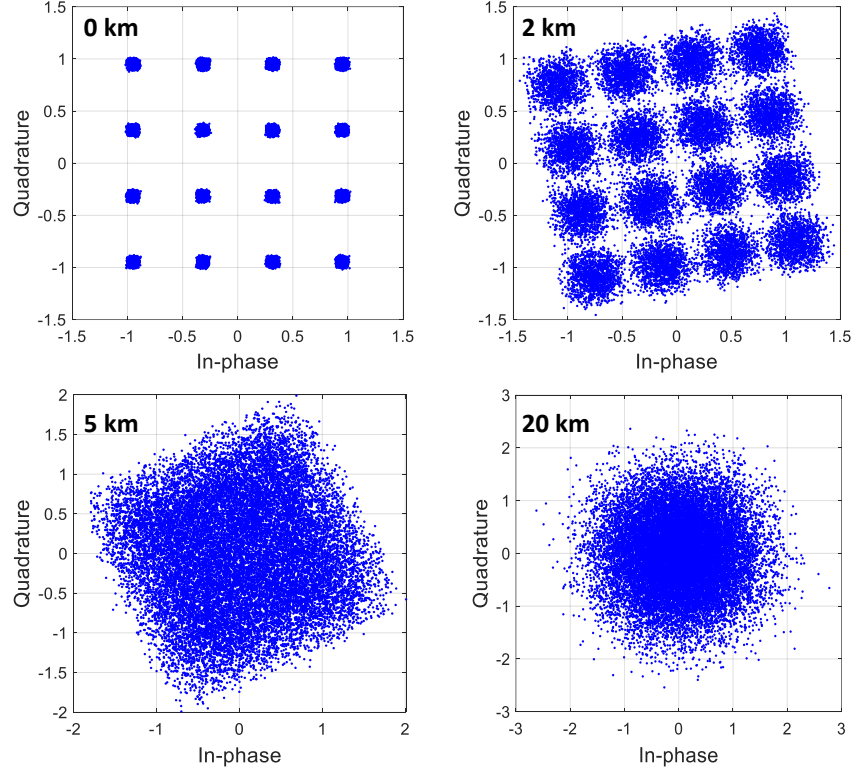
Figure 2.18: Simulated constellations for 50 Gbaud 16QAM using the coherent transmission setup in Figure 2.11.(b), for different lengths of C-band SMF.
