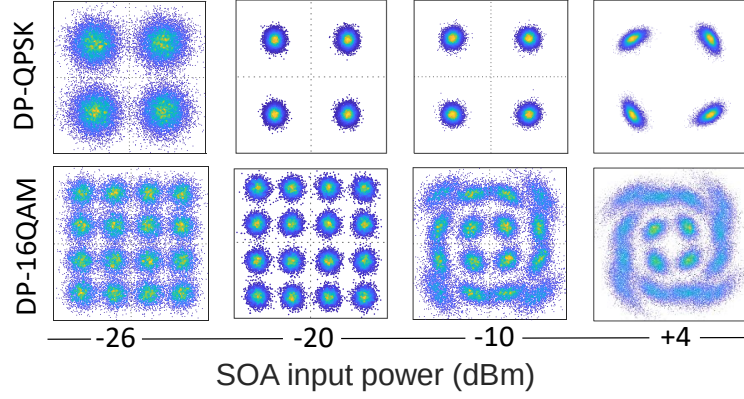
Figure 3.8: Experimental constellation diagrams showing the impact of CIP-SOA-S amplification on DP-QPSK and DP-16QAM signals at increasing input power levels.
