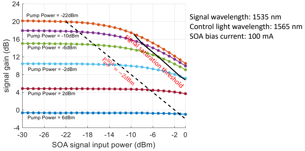
Figure 3.12: Experimentally measured SOA signal gain as a function of increasing input power for multiple control light power levels. Solid black line is gain versus signal saturation input power levels and the dashed black line shows the required signal gain to fix the output power at -2 dBm by increasing the input power.
