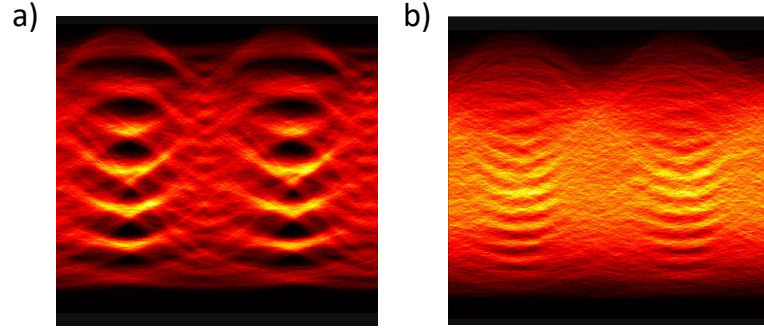
Figure 2.17: Eye diagrams from simulation of 50 Gbaud transmission over 5 km (dispersion D \approx 17 ps/(nm · km)): (a) PAM4 and (b) PAM8.
