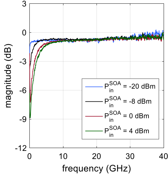
Figure 3.4: Experimental frequency response measurements of CIP-SOA-S at varying input power levels. The SOA is biased at 100 mA for all input power levels.
