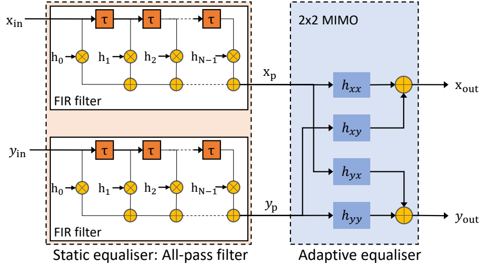
Figure 2.22: Functionality of the digital filtering stage. For linear filtering, the order of the two sub-blocks may of course be reversed.
