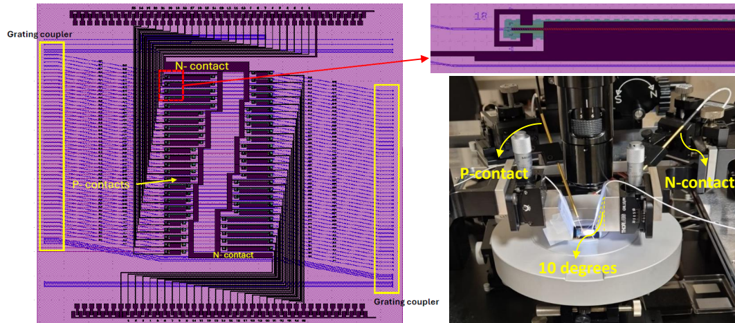
Figure 4.9: TP-SOA chip layout and probe station connection.
