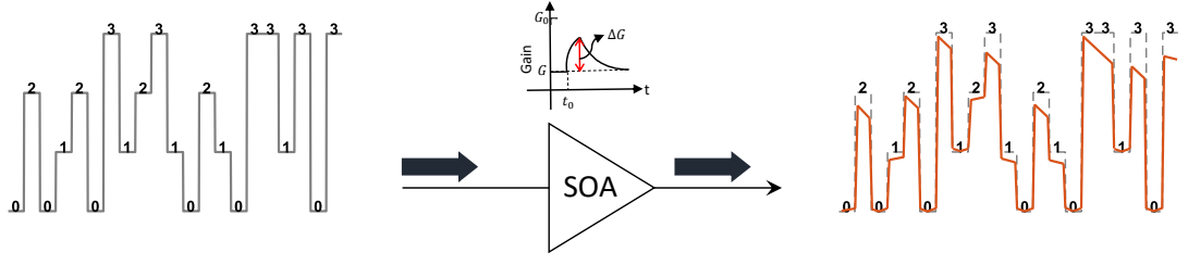
Figure 2.19: SOA gain compression effect on a PAM4 pulse
