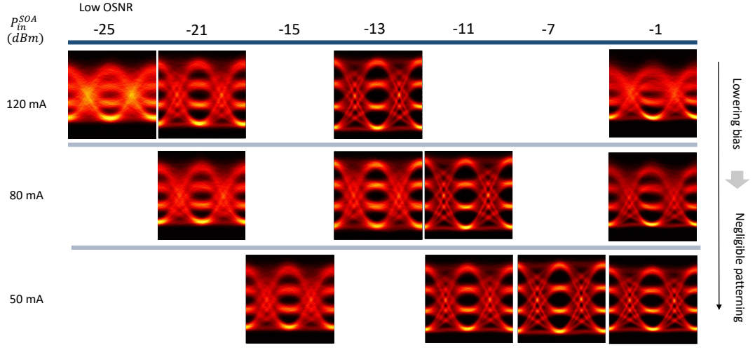
Figure 4.13: Eye diagrams at increasing input powers for multiple bias currents.
