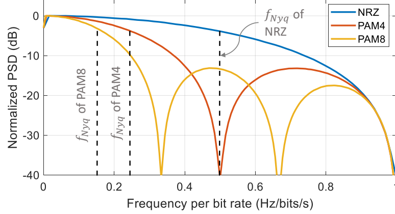
Figure 2.4: Power spectral density envelope for randomly-generated NRZ, PAM4, and PAM8 signal.
