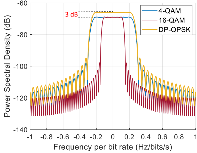
Figure 2.9: PSD of randomly generated 4QAM (QPSK), 16QAM, and DP-QPSK at the same bit rate.
