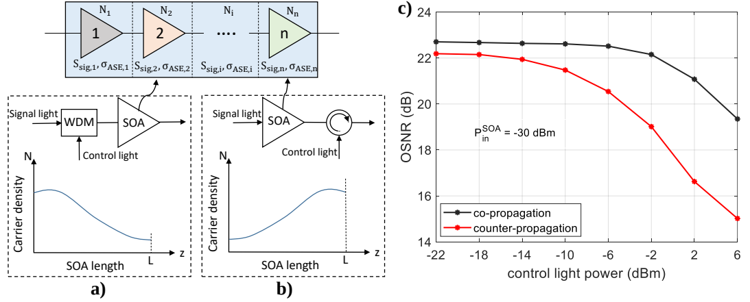
Figure 3.11: (a) Co-propagation injection scheme, (b) counter-propagation injection scheme. The SOA is longitudinally divided into n sections of equal length, and the carrier density graphs correspond to the case where the control light power is much higher than the input power. (c) Experimentally measured OSNR comparison of the two propagation schemes as a function of control light power at an SOA input power of -30 dBm. The loss of the WDM is not taken into account in this measurement.
