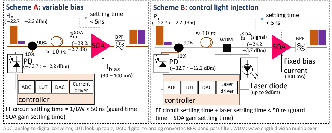
Figure 3.15: The SOA gain controller structure for the two proposed equalisation methods: (A) variable bias, and (B) control light injection.
