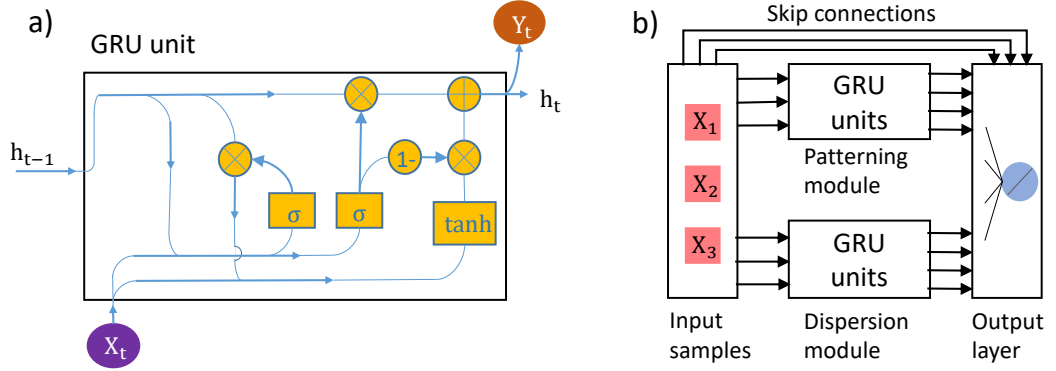
Figure 2.21: (a) Schematic of a GRU unit, and (b) the concept of combining modular GRUs for addressing multiple impairments is shown, where each "module" is exposed to a single isolated impairment during training.
