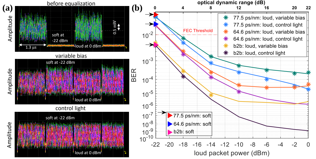
Figure 4.7: (a) Signal traces of burst signals before and after equalisation with two techniques, captured after the SOA preamplifier. (b) BER measurements for 100 Gb/s burst-mode PAM4 transmission using SOA-based equalisation at various dispersion levels. Markers indicate counting errors, and solid lines represent stochastic errors.
