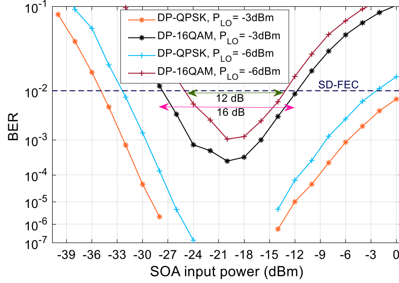
Figure 5.7: Experimental results of 50 Gbaud DP-QPSK and DP-16QAM signals in continuous mode operation after 20 km transmission, measured at different LO power levels using an SOA preamplifier biased at 120 mA and a variable analogue-gain receiver.
