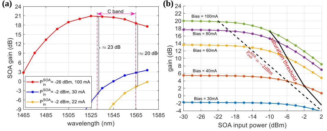
Figure 3.9: Experimentally measured (a) CIP-SOA-S gain spectrum highlighting the effect of bias current on gain change, and (b) gain measurement as a function of increasing input power at multiple bias currents, solid black line is gain versus saturation input power levels and dashed black line shows the required gain to fix the output power at -2 dBm by increasing the input power.
