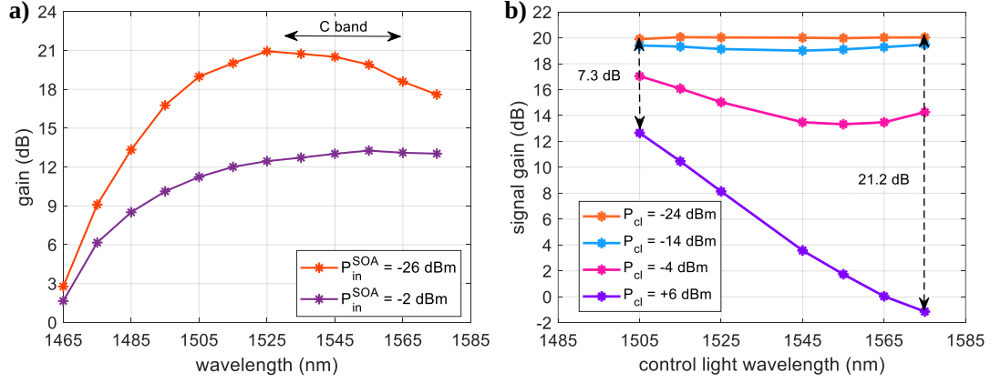
Figure 3.10: Experimental measurement of (a) CIP-SOA-S gain spectrum highlighting the peak gain wavelength shift at high input powers, (b) signal gain at -30 dBm input power to the SOA for a signal placed at 1535 nm, measured for various control light power levels at different control light wavelengths.
