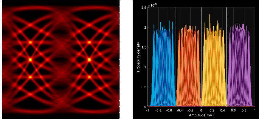
Figure 2.14: Eye diagram and histogram of a simulated 100 Gb/s PAM4 transmission after applying 18.75 GHz Bessel filter.
