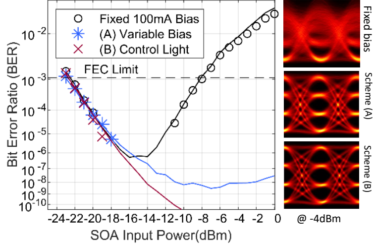
Figure 4.2: BER performance versus SOA input power for the three modes of SOA operation: fixed SOA bias with no power equalisation and the two SOA gain control schemes to maintain a constant output power of -2 dBm.
