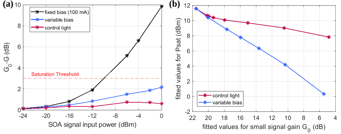
Figure 3.13: Experimental measurement of (a) SOA signal gain reduction compared to the small-signal gain, with a 3 dB drop defined as the saturation threshold across different operating modes, and (b) Fitted values of saturation power versus small signal gain.
