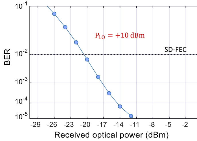
Figure 5.4: Experimentally measured BER versus input optical power for a continuous-mode 50 Gbaud DP-16QAM back-to-back transmission using the integrated coherent receiver, without optical amplification and with an LO power of +10 dBm.
