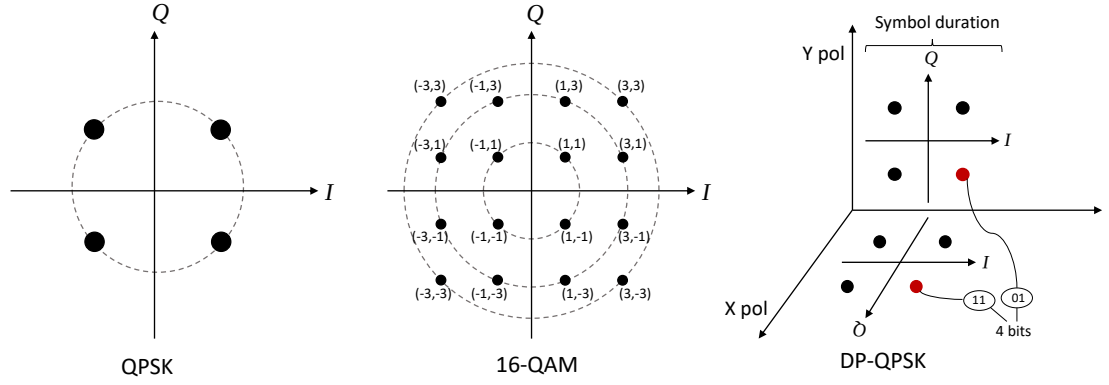
Figure 2.8: Constellations of the inphase and quadrature phases of lightwave carrier under modulation formats QPSK, 16QAM with three rings, and dual polarisation QPSK.
