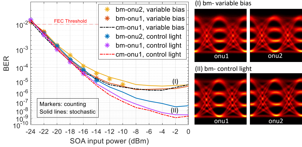
Figure 4.6: Burst-mode (loud (ONU1), and soft (ONU2)) and continuous mode (ONU1) BER measurements using SOA-based equalisation techniques in a 100 Gb/s back-to-back PAM4 transmission. Eye patterns are provided for both ONU1 and ONU2 at an input power of -2 dBm to the SOA.
