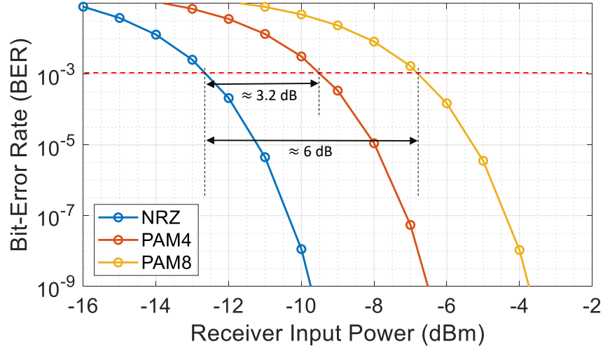
Figure 2.7: Modulation level impact on receiver sensitivity.
