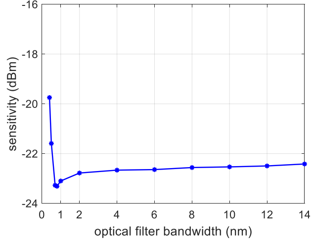
Figure 3.5: The impact of optical filter bandwidth on the receiver sensitivity in an experimental 100 Gb/s PAM4 transmission at \text{BER} = 10^{-2} .
