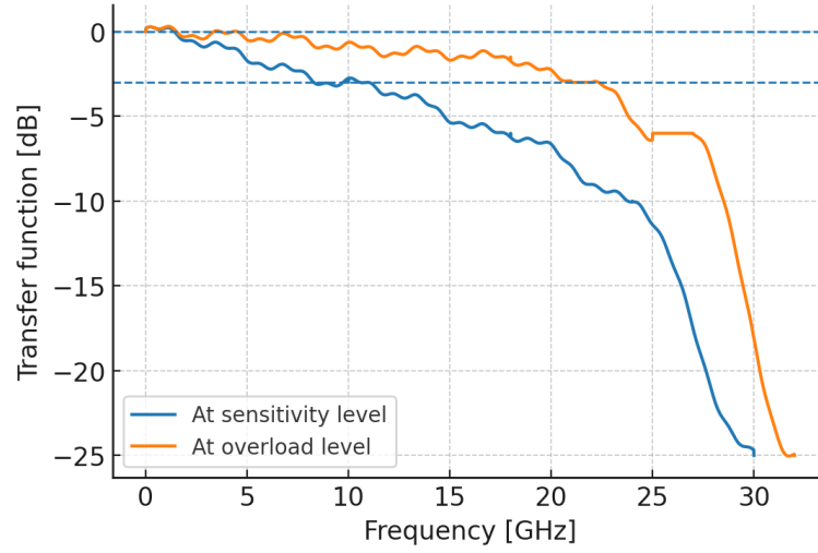
Figure 2.13: Frequency response of the entire transmission system using BM-TIA at sensitivity and overload levels (redrawn based on [49]).
