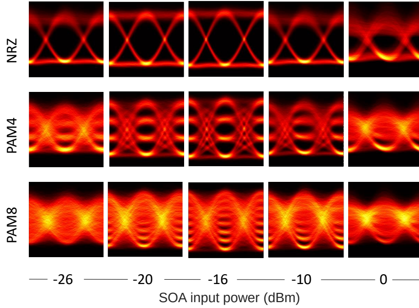
Figure 3.7: Experimental evaluation of the impact of reduced OSNR and gain saturation in CIP-SOA-S on 50 Gbaud M-PAM transmission.
