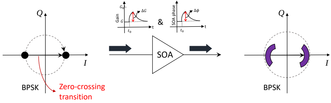
Figure 2.20: Schematic illustration of SOA saturation effects for a BPSK signal.
