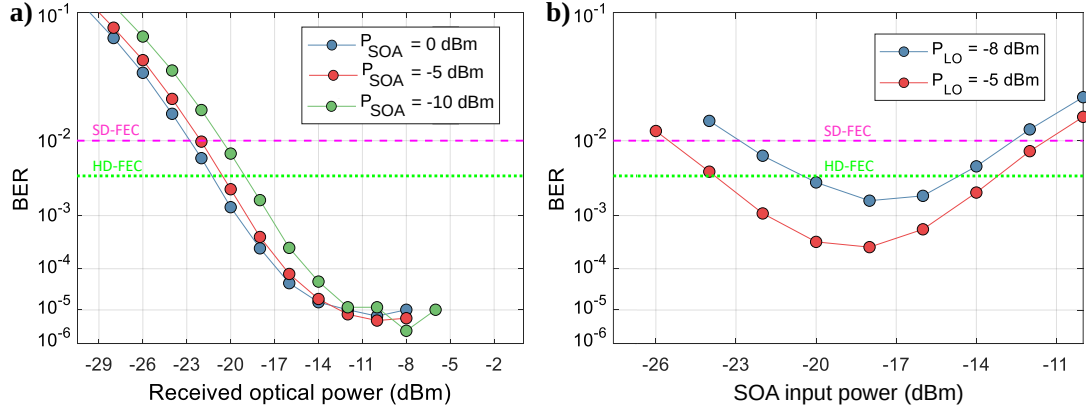
Figure 5.5: BER measurements for a 400 Gb/s DP-16QAM continuous-mode signal, where the receiver analogue gain is adjusted for each input power, comparing two configurations: (a) an SOA in the LO path with a fixed bias and input powers of 0 dBm, -5 dBm, and -10 dBm, resulting in different LO power levels, and (b) an SOA used as a preamplifier with a fixed bias and two different LO powers.
