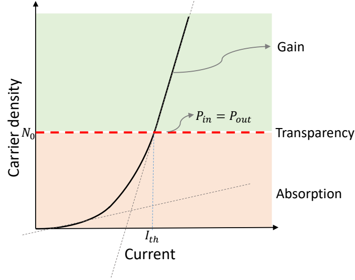
Figure 3.2: Relationship between carrier density and injection current in an SOA. N_0 and I_{th} are the number of carriers and bias current at transparency.
