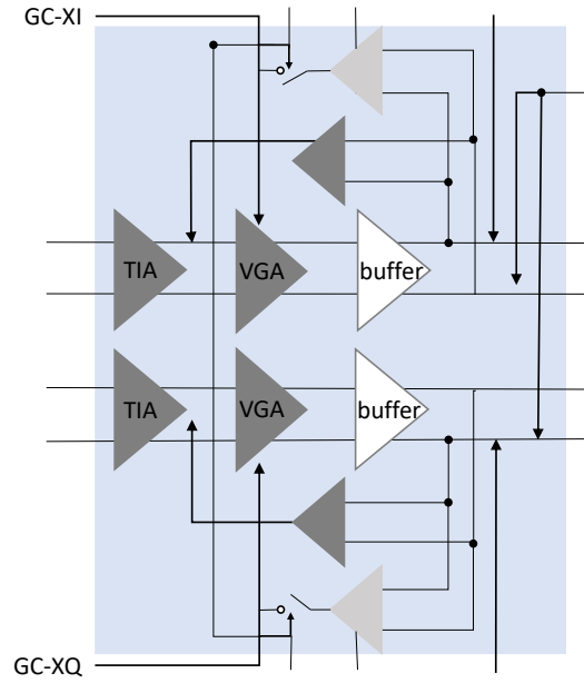
Figure 5.3: Dual-channel TIA-AGC architecture in automatic adjustable mode. This diagram represents X channel only. Y channel has the same diagram.
