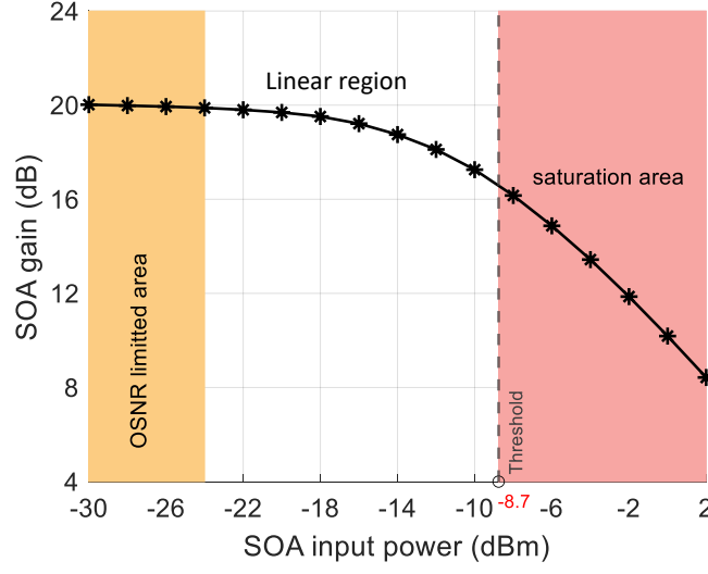
Figure 3.6: Experimental measurement of CIP-SOA-S gain variation with increasing input power in three regions: the OSNR-limited regime, the linear operation regime, and the nonlinear (saturation) regime.
