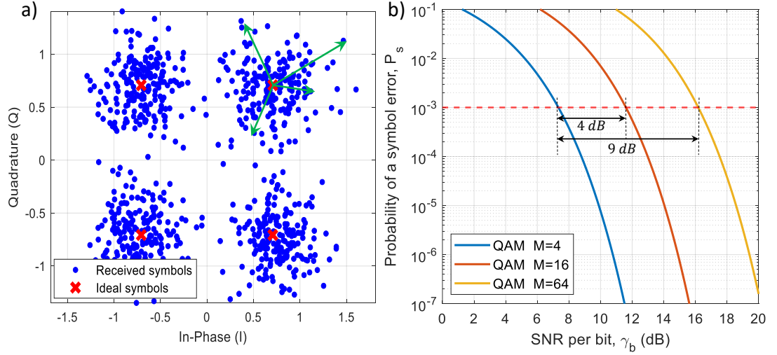
Figure 2.10: (a) Constellation diagram with error vectors (green). EVM is computed as the RMS distance normalised to the reference symbol power. (b) Symbol error probability for M -QAM, plotted using the expression in [41].
