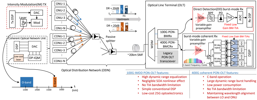
Figure 2.1: Upstream transmission scheme for future PONs, considering IM/DD and coherent technologies operating in the O- and C-bands, respectively.
