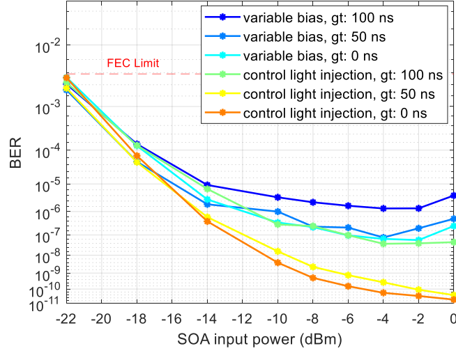
Figure 4.4: Effect of inserted inter-packet idle intervals (guard-time emulation) on the performance of a continuous-wave 100 Gb/s PAM4 transmission using the experimental setup shown in Figure 4.1. The receiver input power is fixed at -2 dBm using the equalisation techniques.
