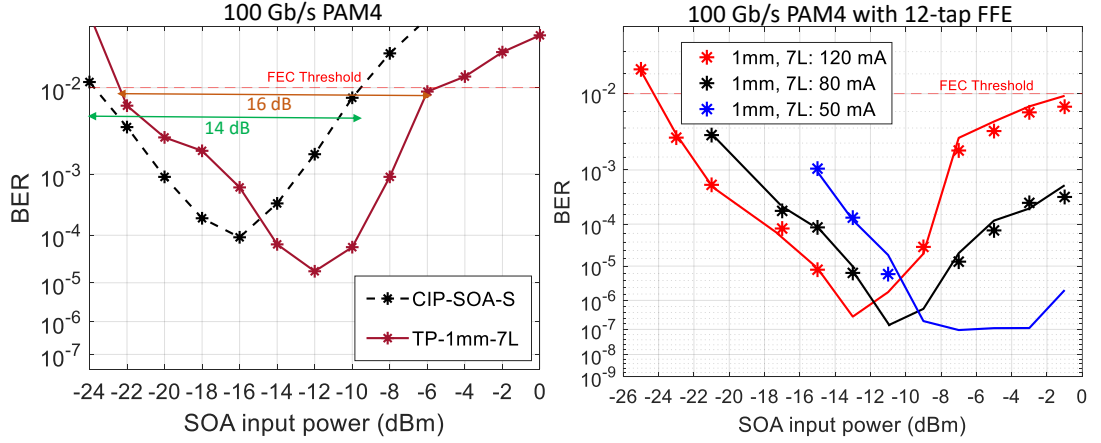
Figure 4.12: (a) BER comparison of TP-SOA and CIP-SOA-S at a fixed bias current of 100 mA for 100 Gb/s PAM4 transmission over a wide dynamic range, and (b) bias reduction impact on the BER performance improvement at high input powers.
