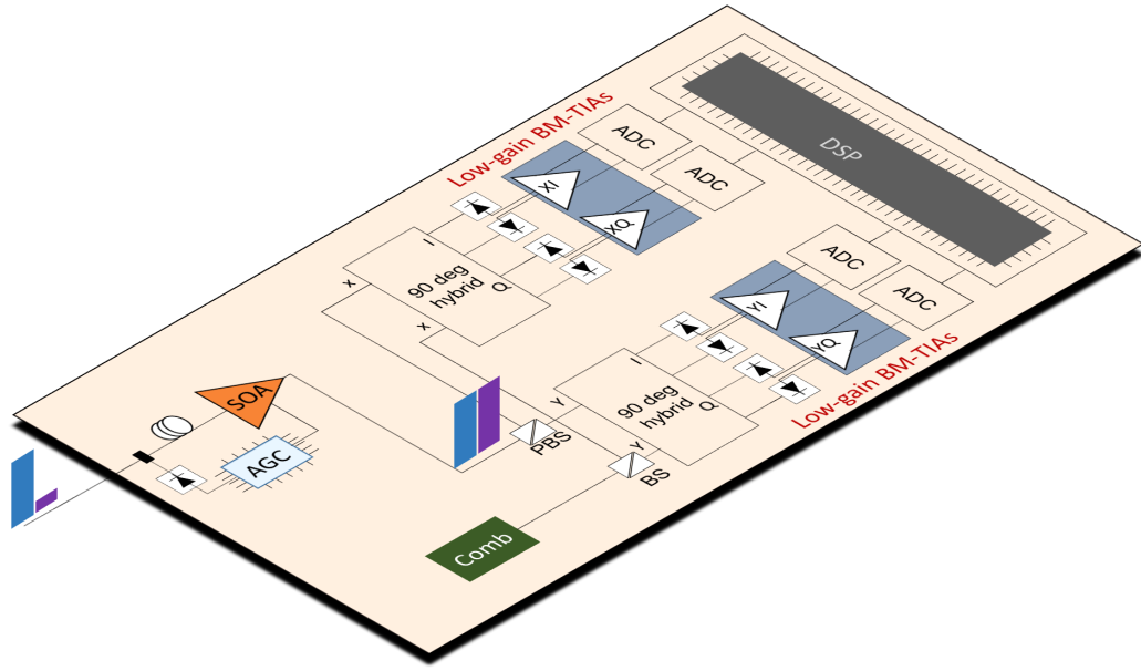
Figure 6.1: Schematic of an integrated optical equaliser in a coherent receiver employing an integrated comb source as the LO for future ultra-high-speed PONs.
