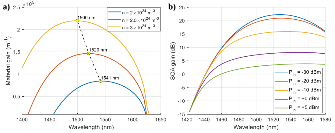
Figure 2.24: Simulation results showing (a) the SOA material gain coefficient spectra at different carrier densities and (b) the SOA gain spectra at different input powers.
