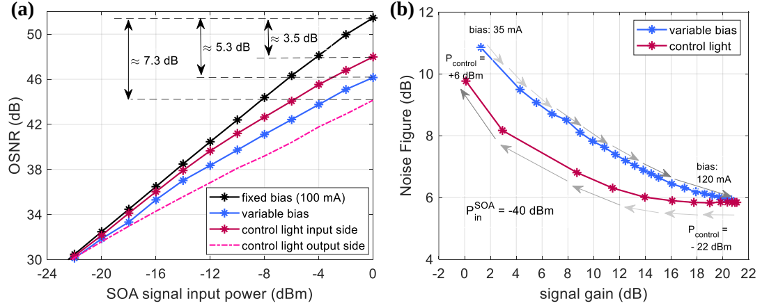
Figure 3.14: (a) Experimental OSNR measurement as a function of SOA signal input power before and after equalisation using the proposed schemes. The OSNR for control light injected from the SOA output is also included. (b) Experimental Noise figure measurement versus small signal gain after equalisation using the proposed techniques.
