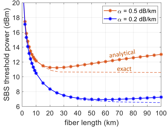
Figure 2.16: SBS threshold power in standard single-mode fibre. Solid lines show the analytical SBS threshold P_{th} evaluated using Equation (2.24). Dashed curves indicate representative reference values inferred from the exact noise-initiated theory reported in [54] and are included for qualitative comparison.
