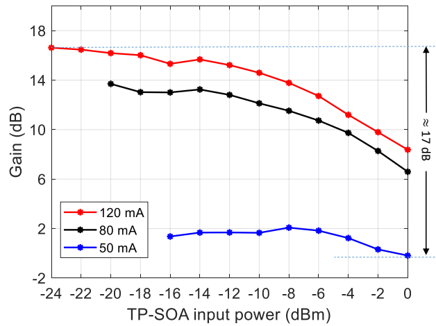
Figure 4.11: Measured TP-SOA gain as a function of input power for several bias currents, illustrating a gain variation of approximately 17 dB.
