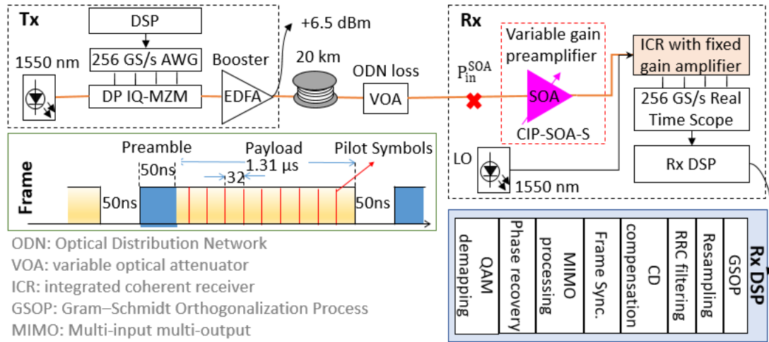
Figure 5.6: Experimental setup of a 20 km optical upstream link in a flexible coherent PON supporting a net data rate of up to 312 Gb/s. The packet frame structure is also shown.
