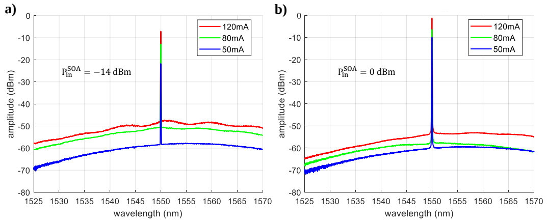
Figure 4.10: Measured spectra of the TP SOA at (a) low and (b) high input powers for multiple bias currents, used to assess potential parasitic lasing.
