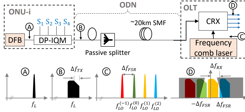
Figure 5.1: Simplified system model of the upstream transmission using a low-cost DFB laser at the ONU and a frequency-comb source at the OLT as the LO [60]. Power spectra at different stages are included.
