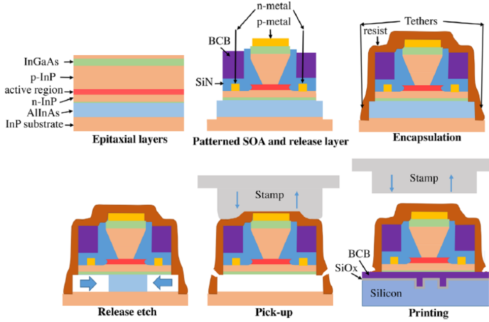
Figure 4.8: Overview of the micro transfer printing process for integrating pre-fabricated III–V devices onto silicon photonic circuits [30].
