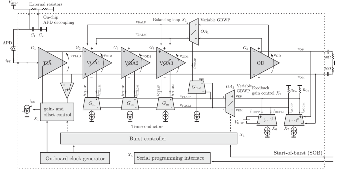
Figure 2.12: The latest state-of-the-art BM-TIA architecture [19]
