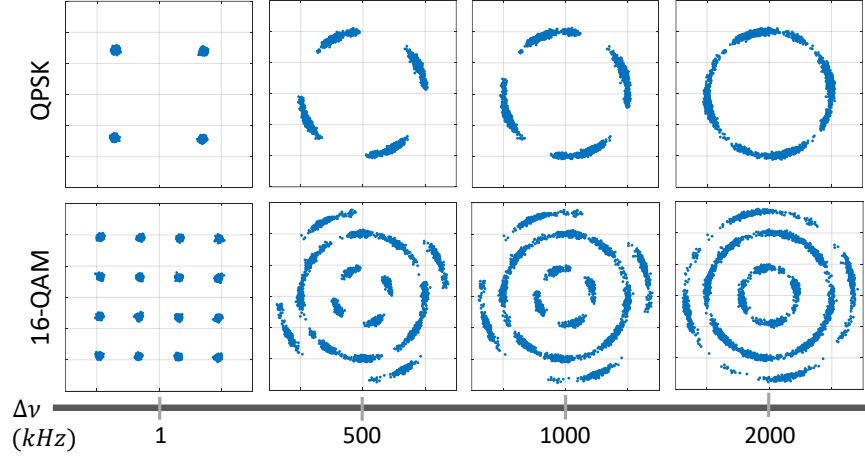
Figure 2.15: Simulated phase-noise-induced distortion of QPSK and 16QAM constellations at a symbol rate of 50 Gbaud for different transmitter and LO laser linewidths.
