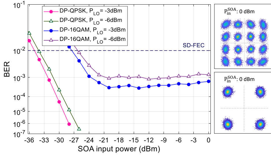
Figure 5.9: Experimental results of 50 Gbaud DP-QPSK and DP-16QAM continuous mode signals at different values of LO power in a 20 km transmission using variable gain SOA and fixed, low receiver analogue gain. Constellation diagrams are for -3 dBm LO power at SOA input power of 0 dBm.
