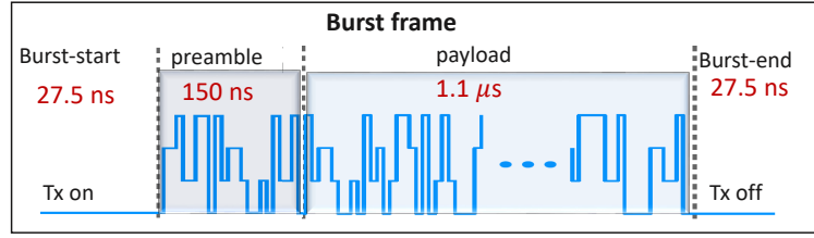
Figure 4.3: Logical structure of the burst frame.
