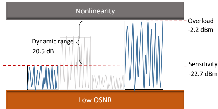
Figure 2.3: Dynamic range between "soft" and "loud" burst packets.
