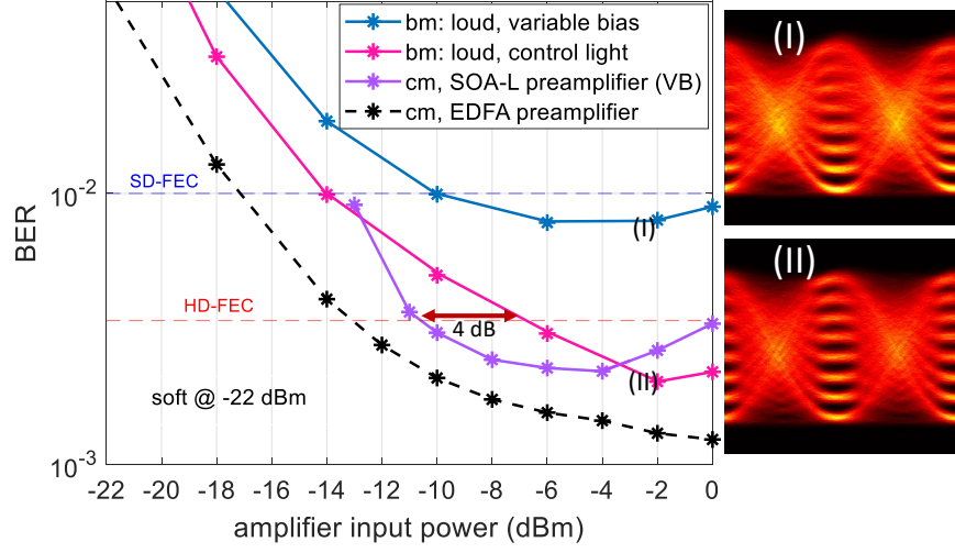
Figure 4.14: 150 Gb/s PAM8 burst-mode back-to-back transmission employing SOA-based power equalisation is analysed. Continuous-mode operation using a linear SOA is included for comparison, and EDFA preamplification serves as an ideal reference case.
