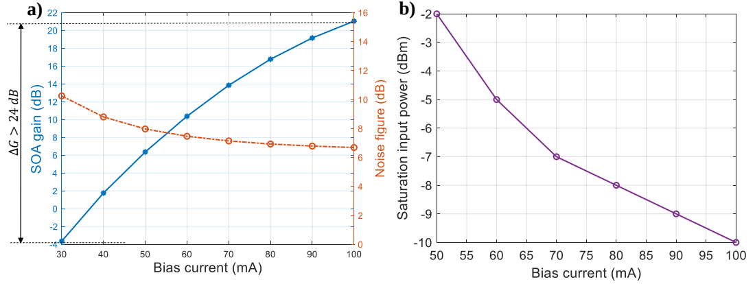
Figure 2.23: Simulation results showing the impact of SOA bias adjustment on (a) gain and noise figure, and (b) saturation input power.
