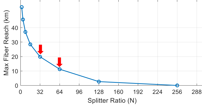
Figure 2.2: Maximum reach versus splitter ratio for given PON power budget of 29 dB.
