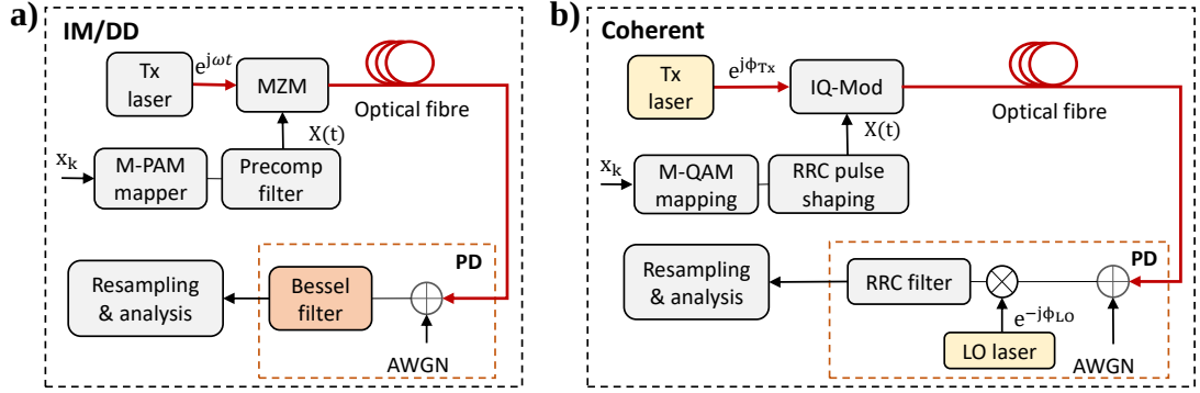
Figure 2.11: (a) IM/DD simulation setup for receiver bandwidth and chromatic dispersion analysis of M -PAM signals. (b) Baseband-equivalent coherent M -QAM simulation model for phase-noise and chromatic dispersion analysis.
