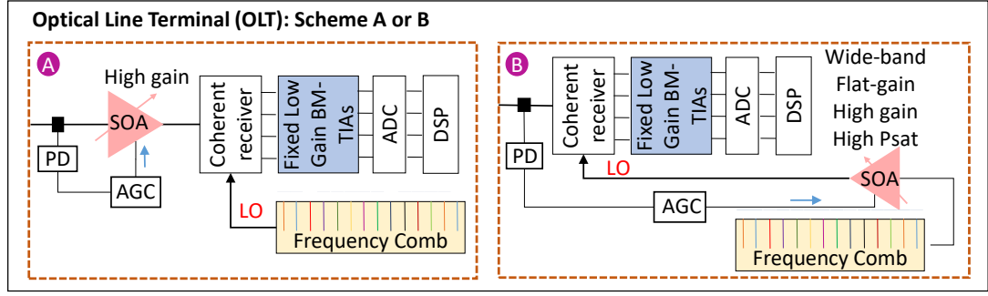
Figure 5.2: OLT receiver architecture showing two possible configurations when a frequency-comb source is used as the LO: (A) SOA-based signal pre-amplification and (B) SOA-based LO power boosting.
