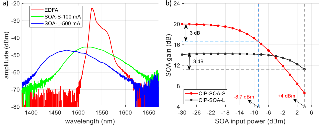
Figure 3.3: Experimentally measured (a) ASE spectra comparison of CIP-SOA-S and CIP-SOA-L with EDFA, (b) CIP-SOA-S (biased at 100 mA) and CIP-SOA-L (biased at 500 mA) gain at increasing input power. -8.7 dBm and +4 dBm are saturation input powers for SOA-S and SOA-L at 1535 nm, respectively.
