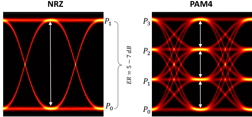
Figure 2.6: Eye diagrams of NRZ and PAM4 with normalised vertical full swing level. Arrows indicate the level-to-level amplitude differences in each eye diagram.
