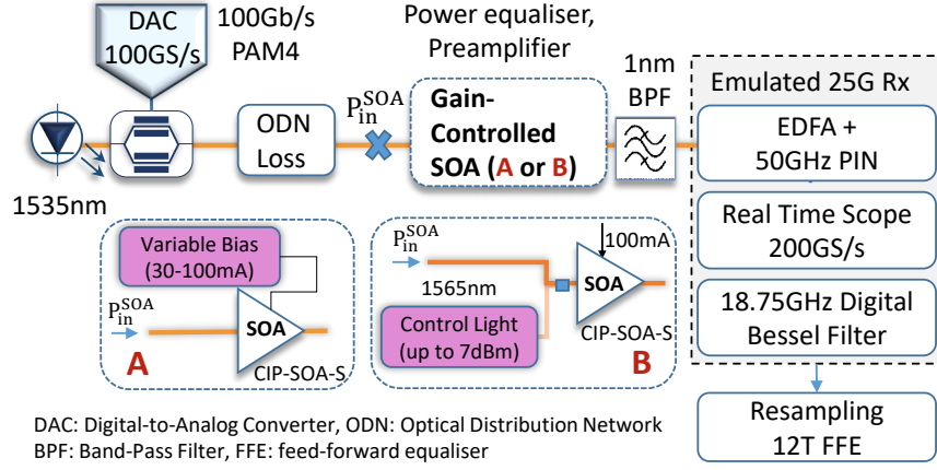
Figure 4.1: Experimental setup emulating PAM4 PON upstream back-to-back transmission using ideal transmitter and receiver to study the two SOA gain control schemes A and B.
