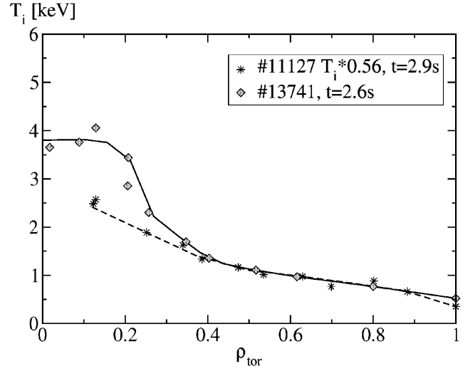
FIG. 2. The ion temperature profiles for #13741 at t = 2.6 s and for #11127 at t = 2.9 s scaled by a factor of 0.56 to be equal in the outer region of the plasma. The symbols represent the actual measured values.
