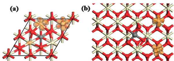
Fig. 6 Spin density plot for Mg adsorbed at the (a) (111) and (b) (110) surfaces of ceria. The spin density isosurfaces are orange and include spin densities up to 0.02 electrons/Å 3 .
