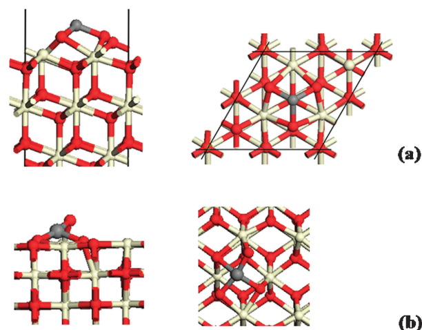
Fig. 5 Atomic structure of Mg adsorbed at the (a) (111) and (b) (110) surfaces of ceria. In the interest of space, only a portion of the (110) surface around the dopant site is shown. The dopant is the grey sphere.
