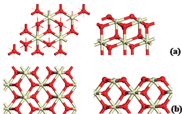
Fig. 4 Atomic structure of the bare CeO 2 surfaces. (a) (111) and (b) (110). In this and subsequent figures, Ce is coloured white and O is red.
