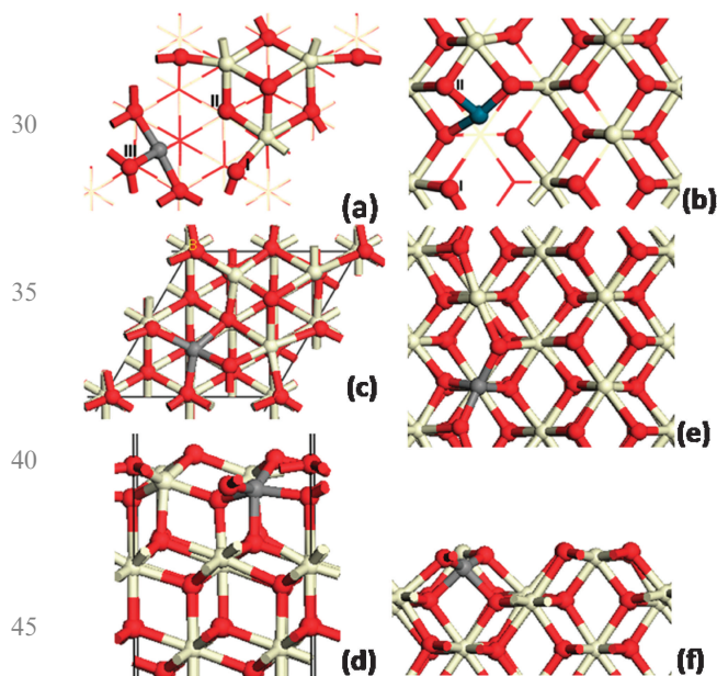
Fig. 10 Oxygen vacancy sites considered for formation of an active oxygen vacancy in Mg doped CeO 2 surfaces; (a): (111) and (b): (110). (c) and (d) show the relaxed structures of the most stable active oxygen vacancy site in the (111) surface and (e) and (f) show the relaxed structure of the most stable active oxygen vacancy site in the (110) surface.
