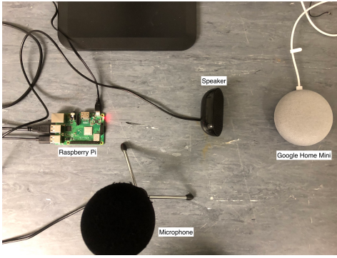
Fig. 3: Experiment Setup.
