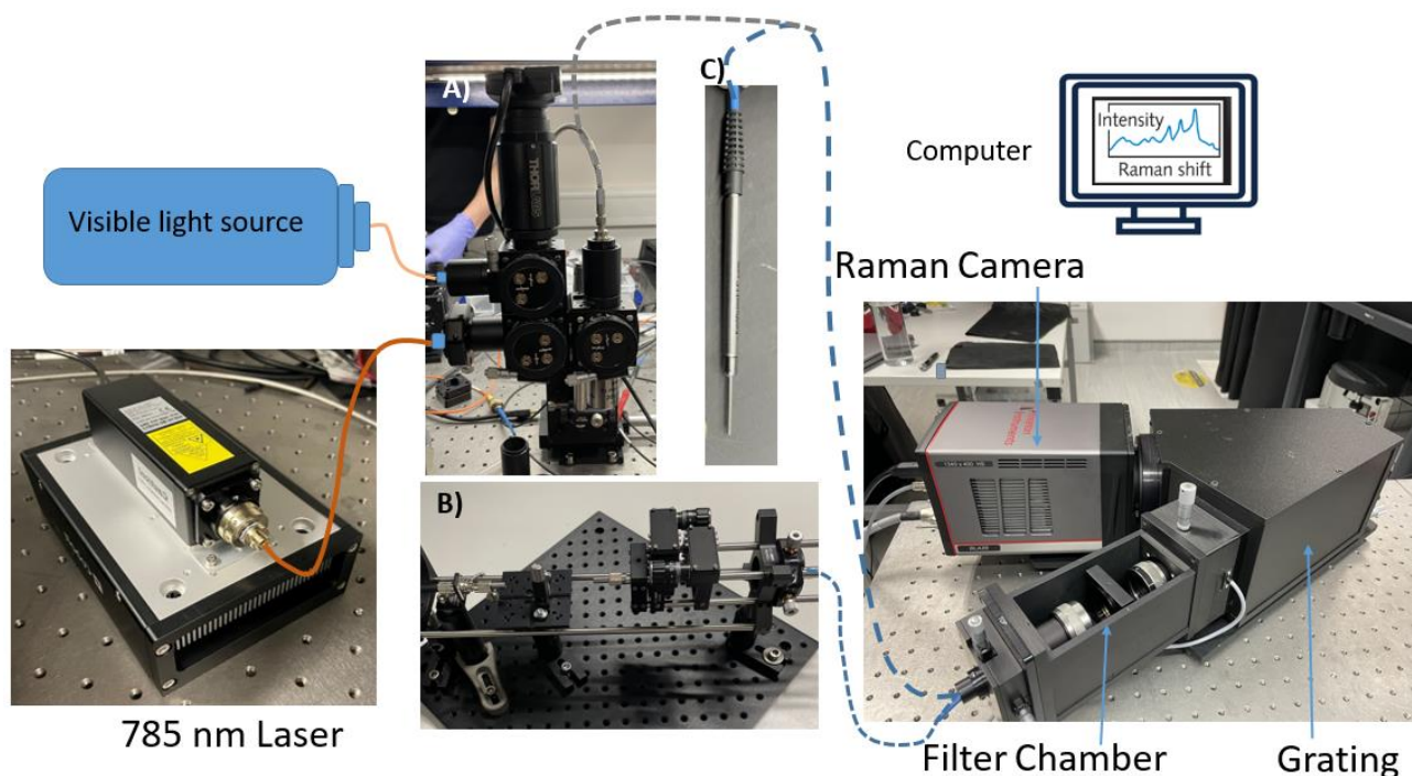
Figure 1. Home built multi-configuration Raman system
