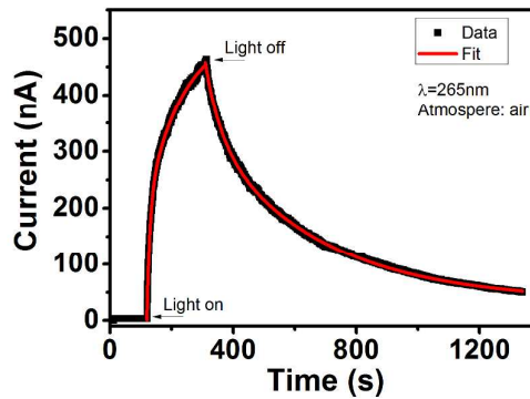
Figure S4. Photoresponse of ZnO nanowire in air device during 200s exposition to UV light (265 nm). Red lines are the bi-exponential growth and decay fitting to the corresponding data.
