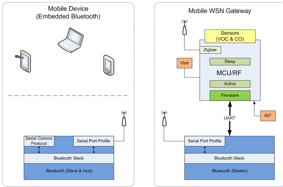
Fig. 2. Schematic of the Mobile Gateway.
