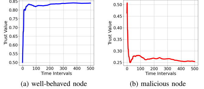
Fig. 1: Trust values over time intervals (a) well-behaved node and (b) malicious node
