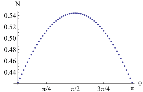
FIG. 7. (Color online) Entanglement between x and y position of the walker in the alternate quantum walk, with the initial conditions of the coin as in Eq. (24), \phi = \pi/2 , and after a number of steps t = 10 .
