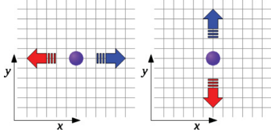
FIG. 1. (Color online) Sketch of the alternate quantum walk: the walker is allowed to move alternately in two orthogonal directions of a two-dimensional lattice; a coin operation is performed before each movement.
