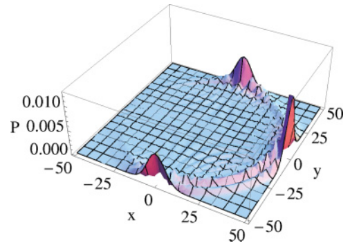
FIG. 4. (Color online) Spatial probability distribution after t = 50 time steps of the alternate quantum walk with the initial state of the coin as in Eq. (26).
