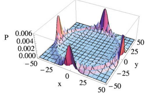
FIG. 2. (Color online) Spatial probability distribution after t = 50 time steps of the two-dimensional Grover walk with the initial state of the coin as in Eq. (5). Only the sites with even x and y are shown, as the probability is zero for all odd sites.
