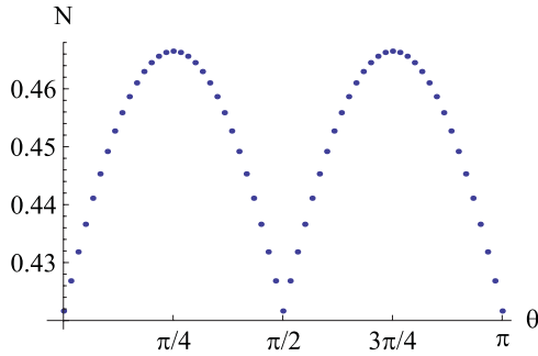
FIG. 5. (Color online) Entanglement between x and y position of the walker in the alternate quantum walk, with the initial conditions of the coin as in Eq. (24), \phi = 0 , and after a number of steps t = 10 .
