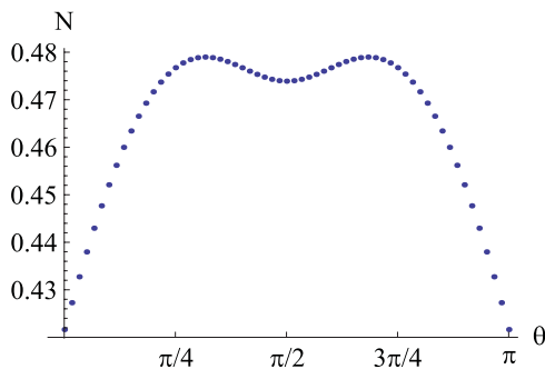
FIG. 6. (Color online) Entanglement between x and y position of the walker in the alternate quantum walk, with the initial conditions of the coin as in Eq. (24), \phi = \pi/8 , and after a number of steps t = 10 .
