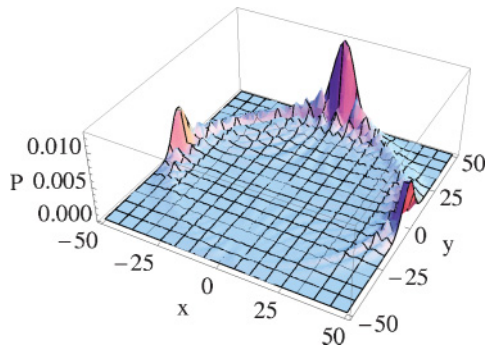
FIG. 3. (Color online) Spatial probability distribution after t = 50 time steps of the alternate quantum walk with the initial state of the coin as in Eq. (25).
