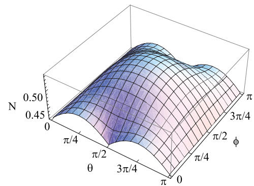
FIG. 8. (Color online) Entanglement between x and y position of the walker in the alternate quantum walk against both \theta and \phi , with the initial conditions of the coin as in Eq. (24) and after a number of steps t = 10 .
