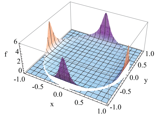
FIG. 9. (Color online) Limit density function f(x, y) for the alternate quantum walk with \gamma = \pi/4 and |\psi_0(0, 0)\rangle = {}^T[1/\sqrt{2}, i/\sqrt{2}] .
