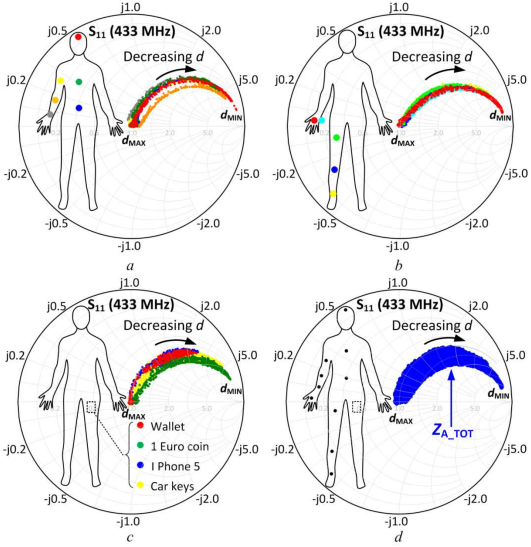
Fig. 2. Summary of on-body AUT impedance measurements
