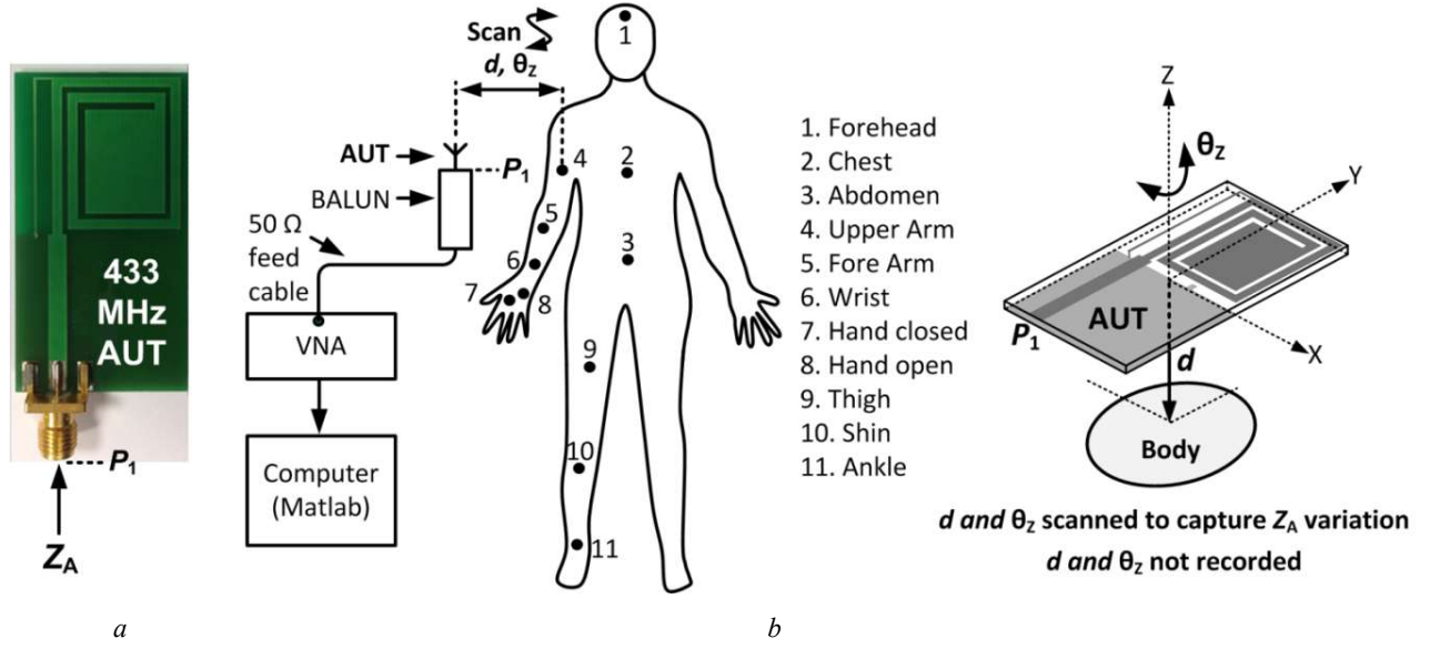
Fig. 1. Details of AUT and on-body antenna measurement setup using a human test subject a. Photograph of 433 MHz AUT b. Overview of measurement setup for on-body AUT characterization
