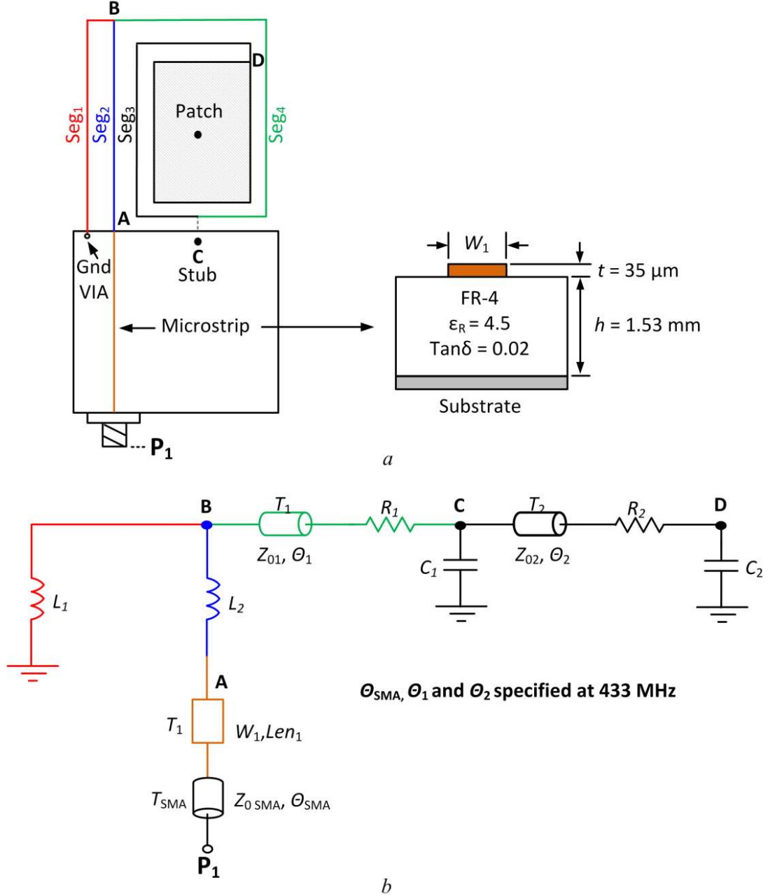
Fig. 3. Transmission line model of 433 MHz AUT
