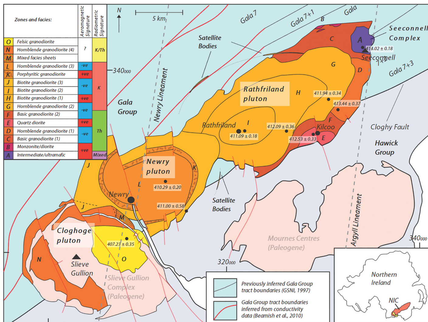
Figure 1. Geology of the Newry igneous complex (NIC) and its host rocks, including age determinations (in Ma) for the Newry igneous complex and recognized aeromagnetic/radiometric anomalies within the complex derived by Cooper et al. (2016); a newly mapped zonation of the Newry igneous complex (defined by zones A–O) derived by Anderson et al. (2016); and a simplification of the local host-rock structure, highlighting the modified Gala Group tract boundaries inferred by Beamish et al. (2010). The zonation includes the satellite bodies, which consist of fine-grained biotite/hornblende granodiorite. The positions of major grid lines (corresponding to sample grid references within Appendix 2 [see text footnote 1]) and the locations of key geographical features are also shown. Irish grid coordinate system.
