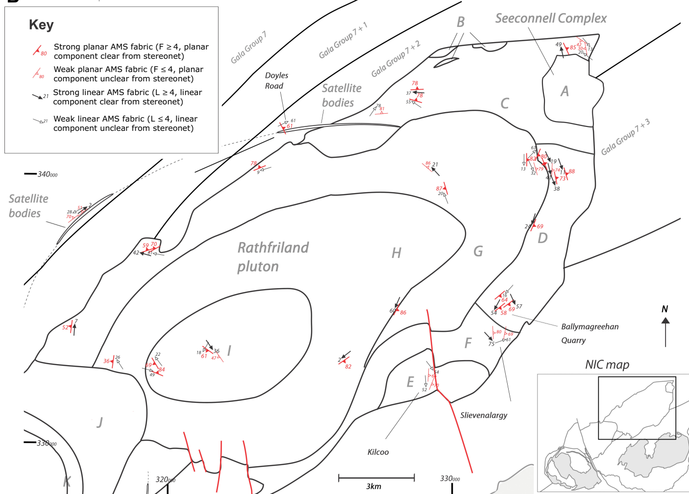
Figure 4 (continued). (B) Derived planar and linear AMS fabrics for the Rathfriland pluton and adjacent satellite bodies.
