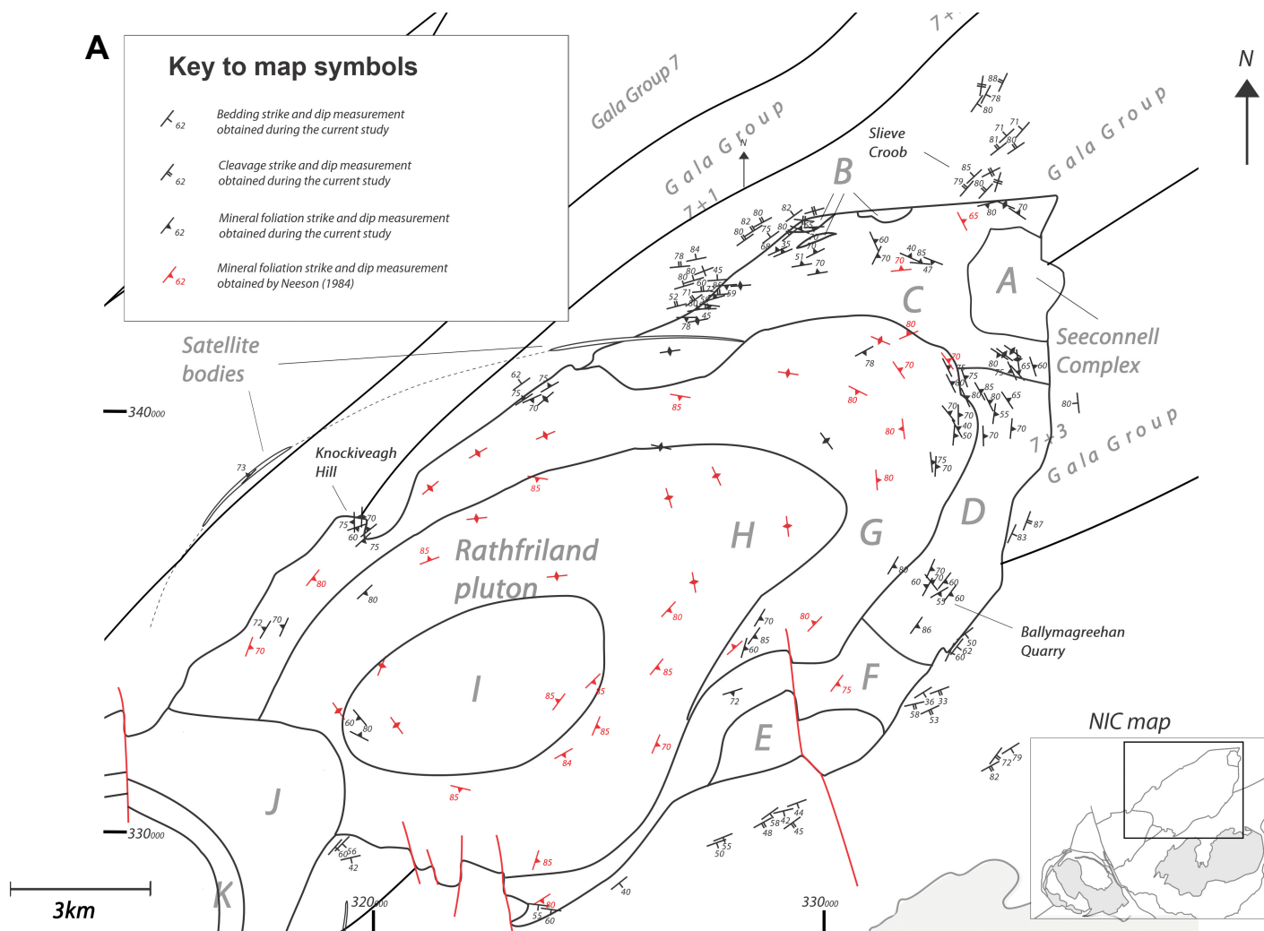
Figure 3 (on this and following page). Field structural data collected from the Newry igneous complex (NIC), satellite bodies, and host rocks. All data were collected during the current study, excluding the highlighted mineral foliations collected by Neeson (1984). (A) Data collected from the Rathfriland pluton and adjacent host rocks/satellite bodies.
