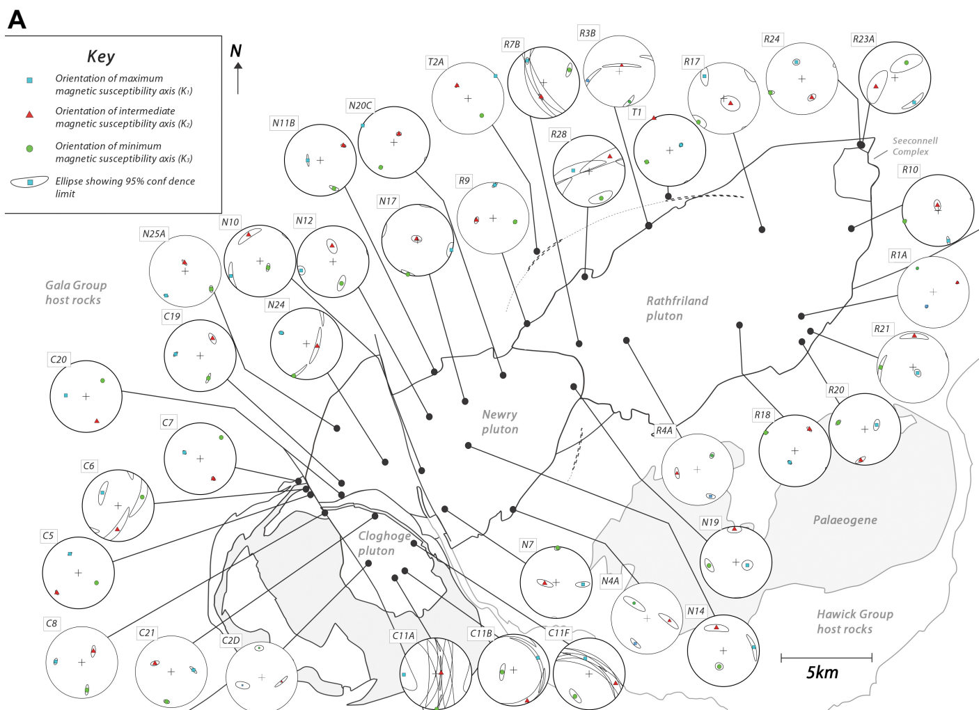
Figure 4 (on this and following two pages). (A) Stereographically plotted anisotropy of magnetic susceptibility (AMS) results for selected samples from the Newry igneous complex (NIC) and satellite bodies.
