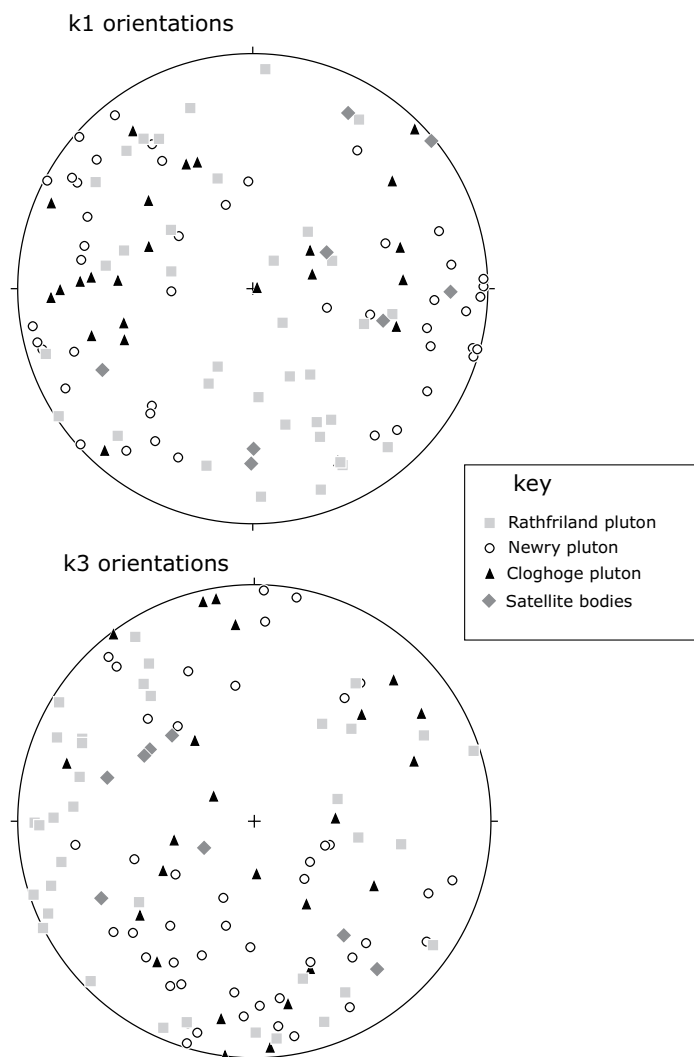
Figure 5. Stereographically projected orientations of K_1 (upper stereonet) and K_3 (lower stereonet) values obtained from anisotropy of magnetic susceptibility (AMS) analysis. Results from the three plutons of the Newry igneous complex and the satellite bodies are distinguished.
