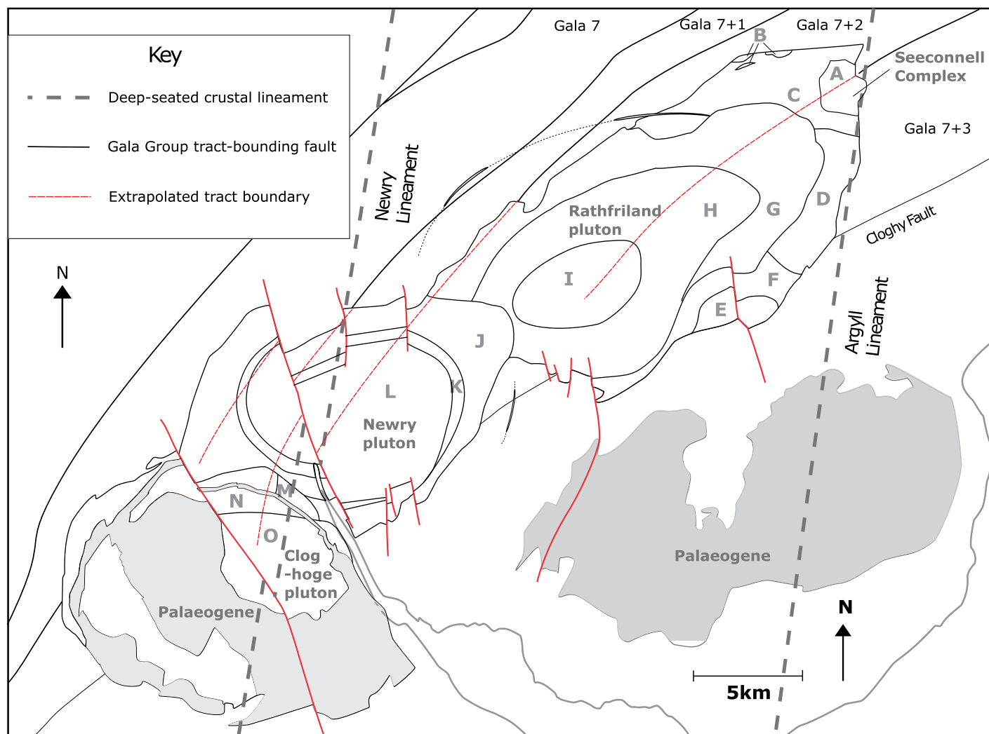
Figure 9. Gala Group tract boundaries and deep-seated crustal lineaments in the vicinity of the Newry igneous complex. Tract boundaries are extrapolated through the Newry igneous complex (after Beamish et al., 2010; Cooper et al., 2013). See Figure 1 for zones and facies.
