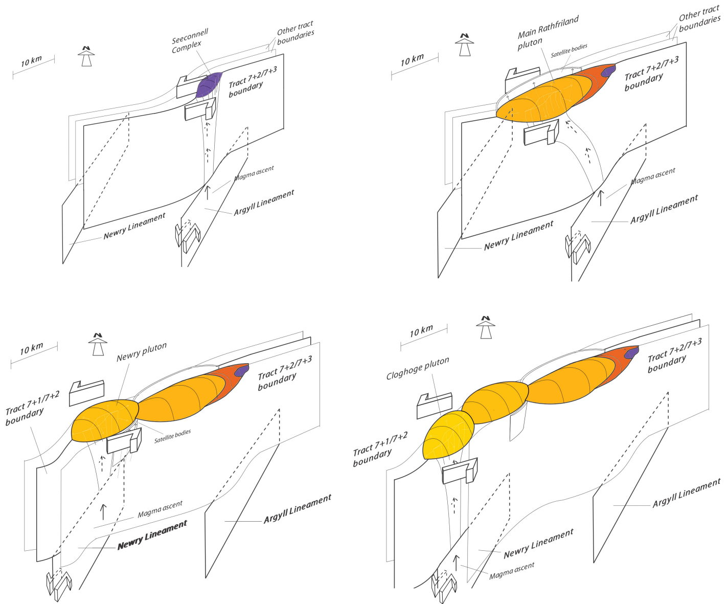
Figure 10. Schematic emplacement history of the Newry igneous complex and its satellite bodies, showing the interaction between deep-seated lineaments and Gala Group tract boundaries within the crust.
