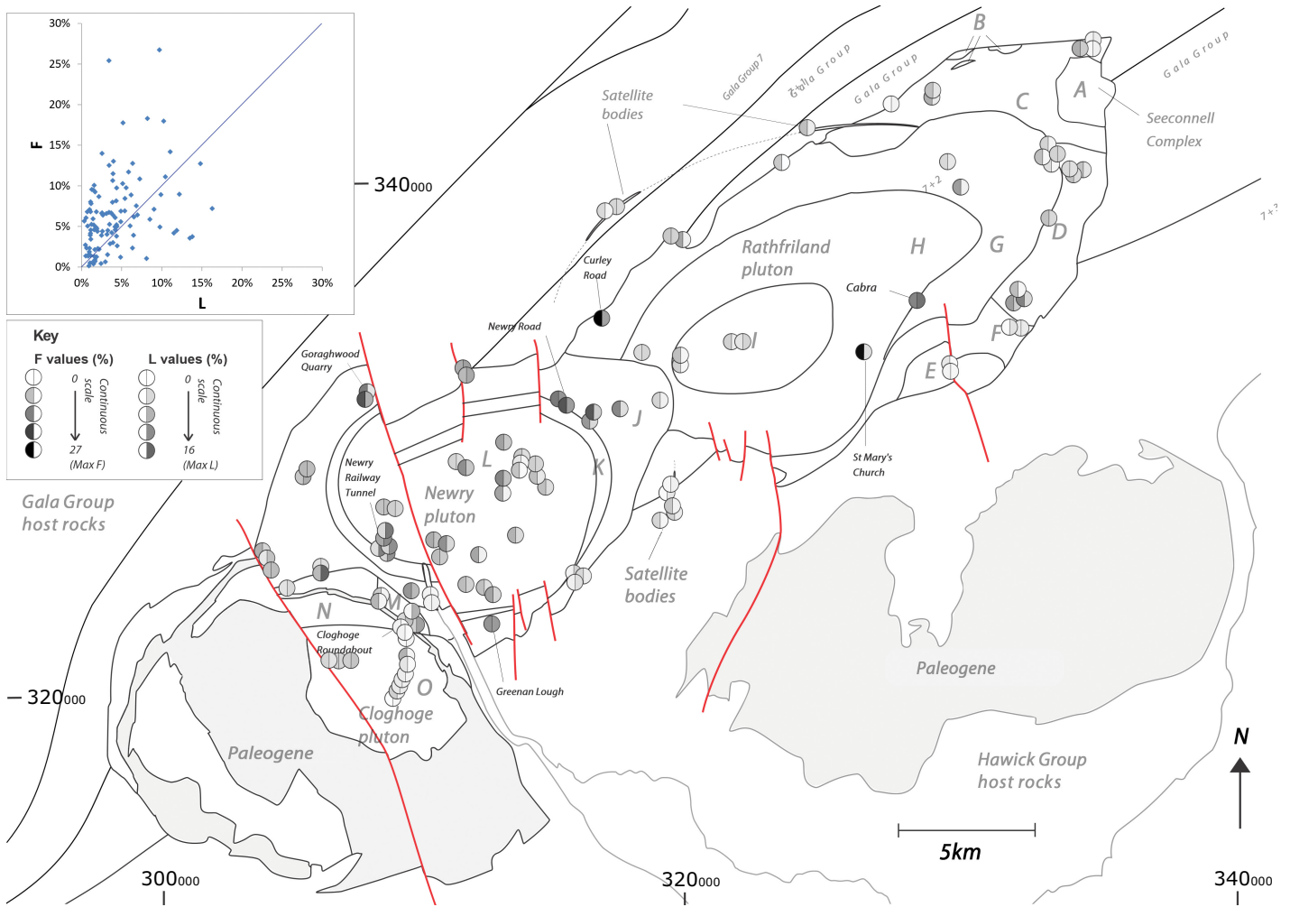
Figure 6. Anisotropy of magnetic susceptibility (AMS) fabric strengths (planar = F , linear = L ) within the Newry igneous complex and satellite bodies. F and L are mapped as well as plotted against each other in the inset graph. See Figure 1 for zones and facies. Irish grid coordinate system.
