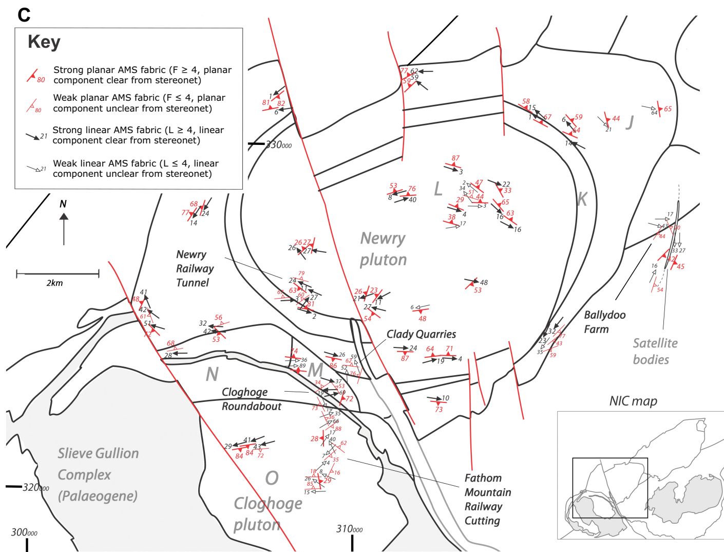
Figure 4 (continued). (C) Derived planar and linear AMS fabrics for the Newry and Cloghoge plutons and adjacent satellite bodies. See Figure 1 for zones and facies. Irish grid coordinate system.
