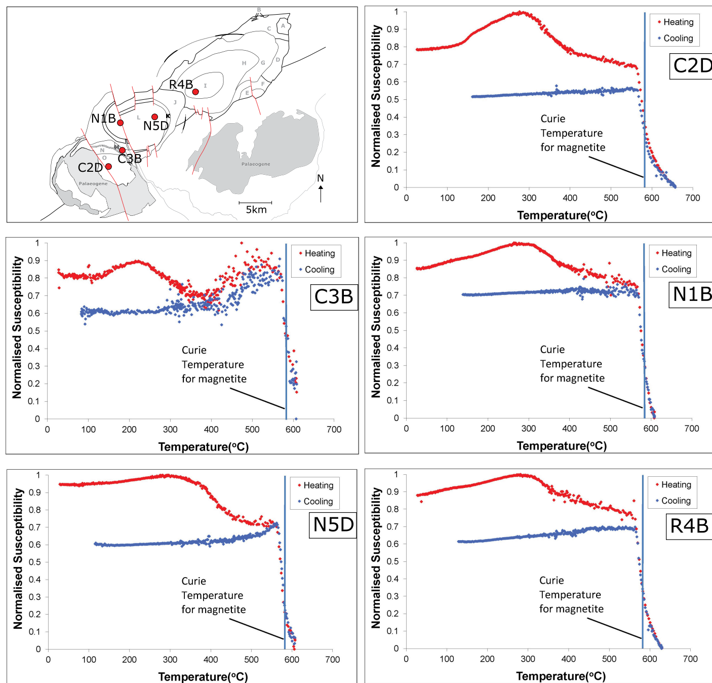
Figure 8. Thermomagnetic results, showing changes in magnetic susceptibility during heating and subsequent cooling for five samples from the Newry igneous complex. Sample locations are shown on the inset map (see Fig. 1 for zones and facies). Irish grid coordinate system.
