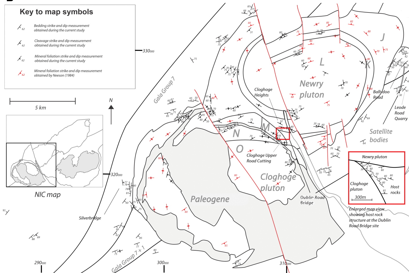
Figure 3 (continued). (B) Data collected from the Newry and Cloghoge plutons and adjacent host rocks/satellite bodies, and inset showing an enlarged map relating to the area of host rock between the southern Newry and Cloghoge pluton boundaries. See Figure 1 for zones and facies. Irish grid coordinate system.
