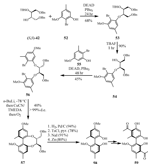
Scheme 10.
