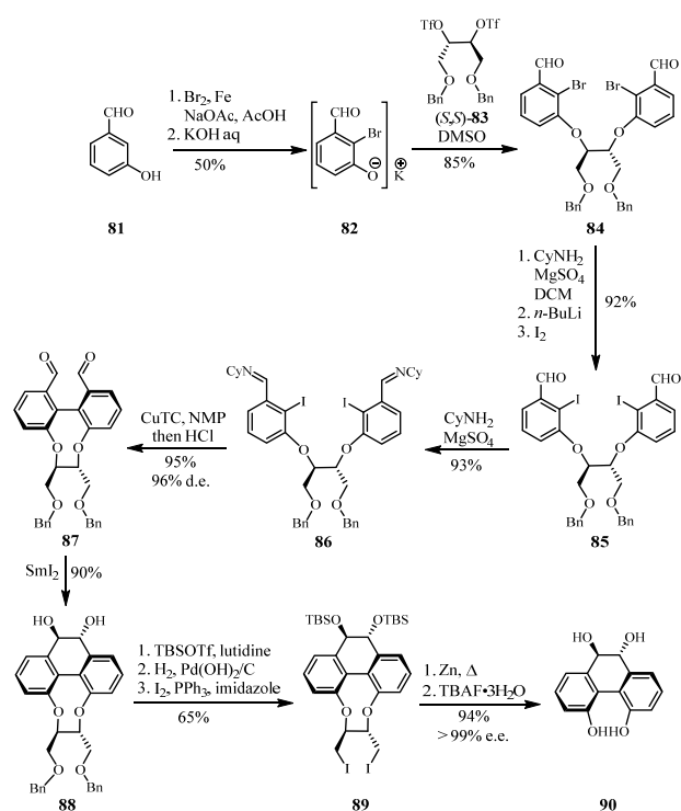
Scheme 15.
