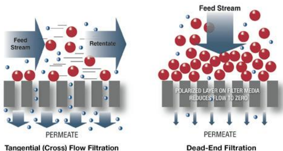
Figure 13. Comparison between Tangential Flow Filtration (TFF) and Dead-End Filtration
