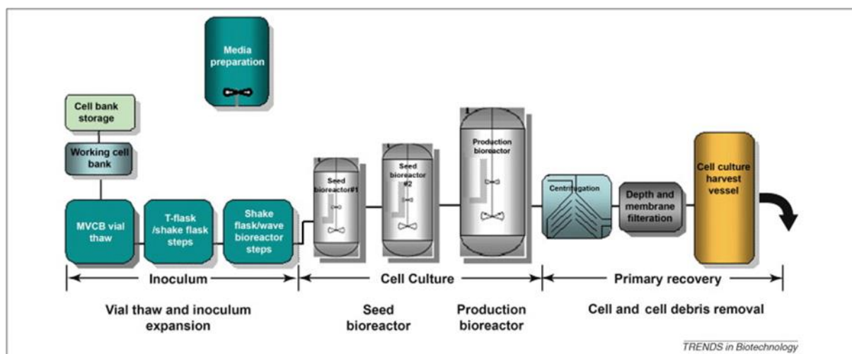
Figure 9. Monoclonal Antibody Upstream production process (Shukla and Thömmes, 2010)
