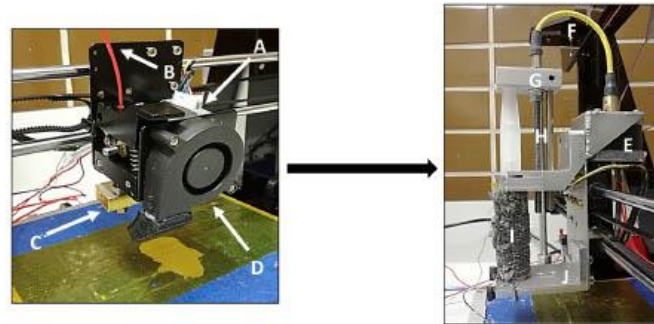
Fig. 1. A - Stepper Motor, B - Polylactic Acid (PLA) Filament, C - Hotend, D - Hotend Fan, E - Stepper Motor, F - Flexible Drive Shaft, G - Plunger Housing, H - Helical Screw, I - Syringe Barrel with Insulation, J - Syringe mount.
