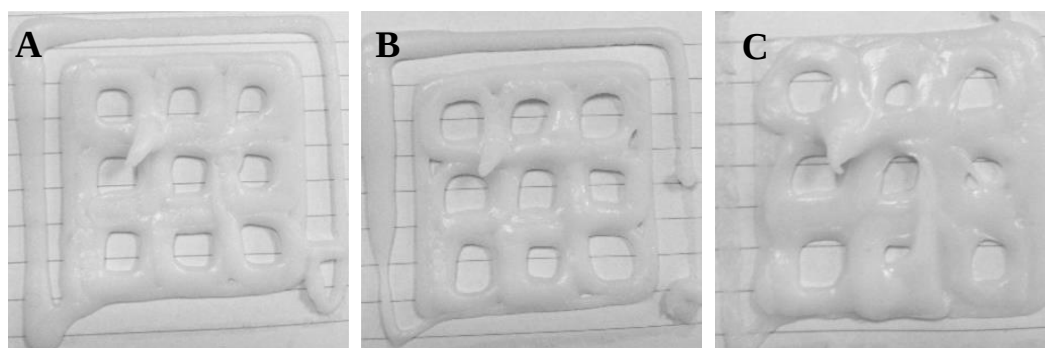
Fig. 3.8 (A-C). 3D-printed 40 mm 2 grid, A (Recipe A: pH 5.4), B (Recipe B: pH 5.6), and C (Recipe C: pH 5.8).
