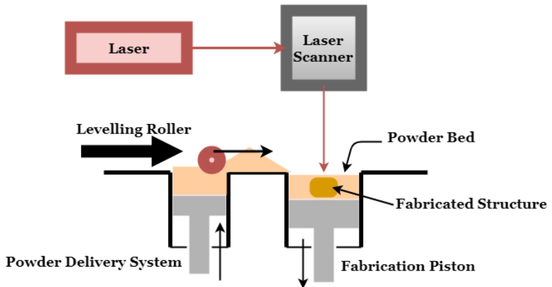
Fig. 1.3. Principle of a laser sintering: a laser melts the fine layer of powdered material to cause it to fuse together into a solid structure. The levelling roller scrapes each layer to provide an even surface for the subsequent lasering.
