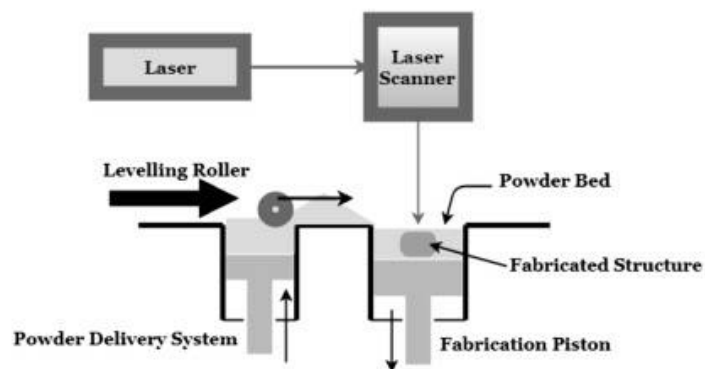
FIGURE 7.3 Principle of a laser sintering: a laser melts the fine layer of powdered material to cause it to fuse together into a solid structure. The levelling roller scrapes each layer to provide an even surface for the subsequent lasering.
