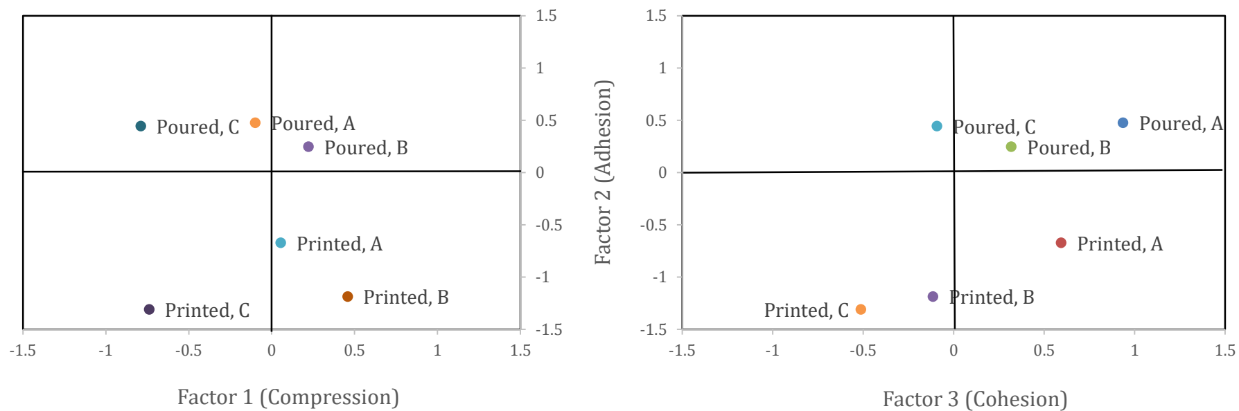
Fig. 3.9. Quality chart with the factor scores of the samples (averages of 3 independent repeat measurements) of the pH dataset (Recipes A-C)
