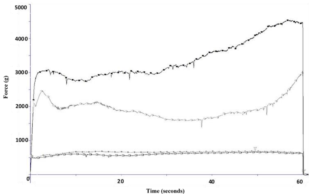
Fig. 2.15. Texture Profile Analysis graph showing force required to extrude Cream cheese (18°C) (■), Cream cheese (30°C) (○), Ketchup (18°C) (●) and Ketchup (30°C) (□) from a syringe
