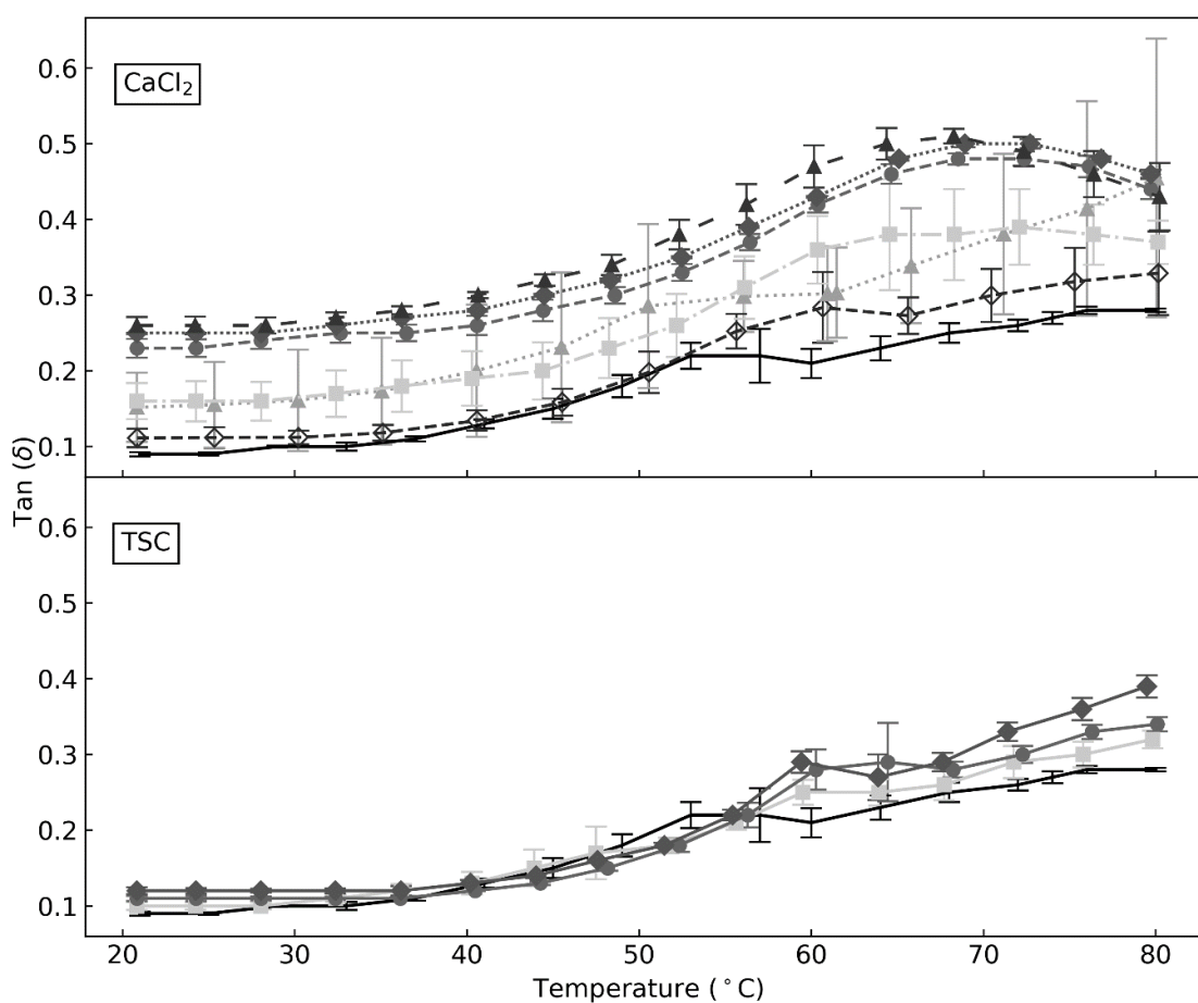
Fig. 4.4. Comparison of melting profiles of 3D-printed MCC samples. (Note: Control and TSC samples (unbroken lines) and \text{CaCl}_2 samples (broken lines)). Control (—), 1 mM \text{CaCl}_2 (—◇—), 2.5 mM \text{CaCl}_2 (—▲—), 5 mM \text{CaCl}_2 (—■—), 10 mM \text{CaCl}_2 (—●—), 15 mM \text{CaCl}_2 (—◆—), 20 mM \text{CaCl}_2 (—▲—), 5 mM TSC (—■—), 10 mM TSC (—●—) and 15 mM TSC (—◆—).
