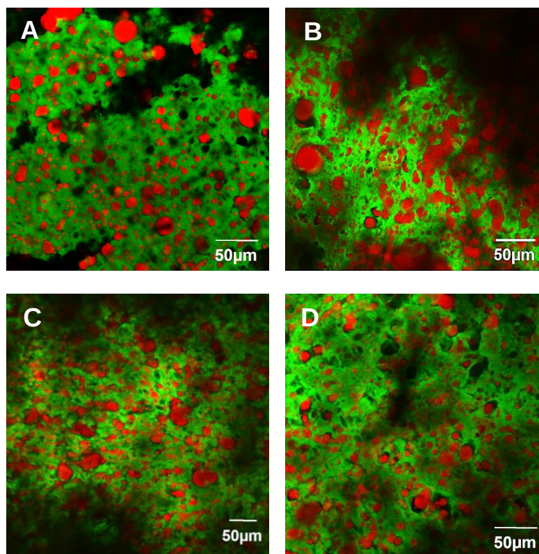
Fig. 3.6. CSLM Micrographs - A = Poured recipe A, B = Poured recipe F, C = Printed recipe A, and D = Printed recipe F (Images were taken using a 40x objective) (Red (Nile red stain) = Lipids, Green (Fast Green FCF) = Protein)
