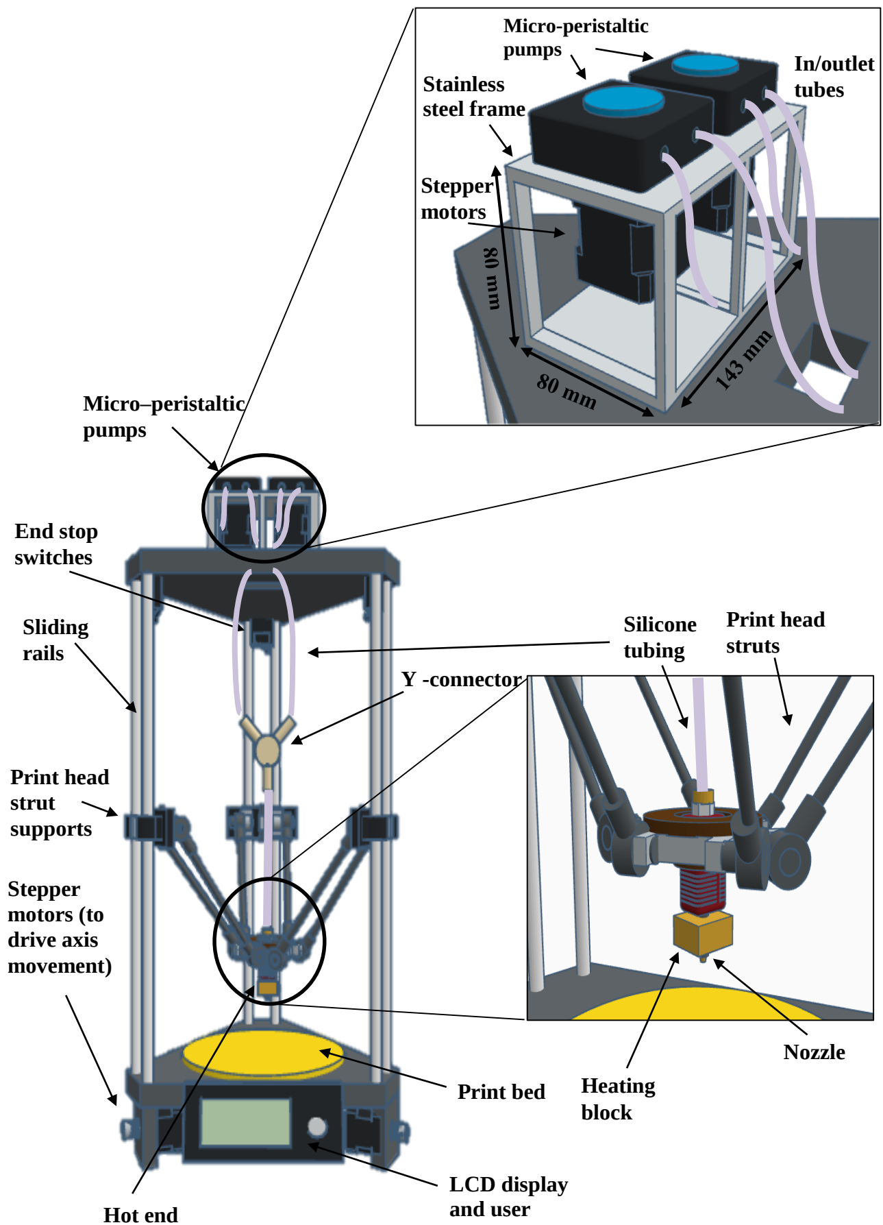
Fig. 2.3. Diagram of Delta 3D printer post-modification. (A) Close-up of micro-peristaltic pumps, stainless steel holder and silicone in/outlet tubes and (B) Close-up of modified print head
