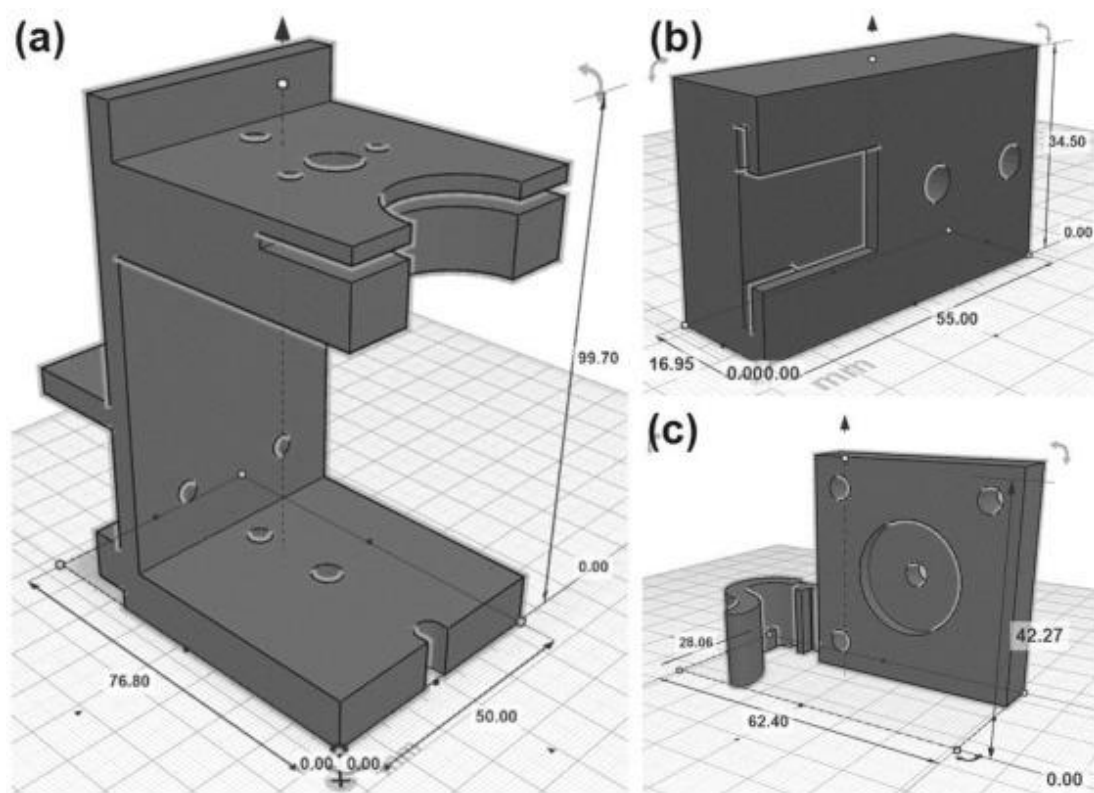
Fig. 2.7. Original design inspiration for modifications made to the Cartesian 3D printer. Computer aided design (CAD) drawings of the extrusion system elements: (a) syringe mount, (b) syringe plunger holder and (c) extrusion motor mount (Obtained with permission from Le Tohic et al. , 2018).
