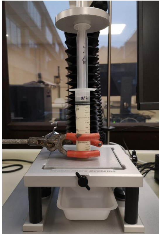
Fig. 2.13. Layout of modified syringe rig using Texture Profile Analysis (TPA) equipment
