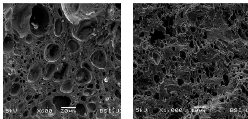
Fig. S3.7. SEM Micrographs of (Left – Recipe E poured samples contain mostly large spherical fat globules interspersed between a reasonably dense protein network, Right – Recipe E printed samples appear to have a lipid fraction which are irregular in shape and are much smaller in size than those appearing in poured samples)
