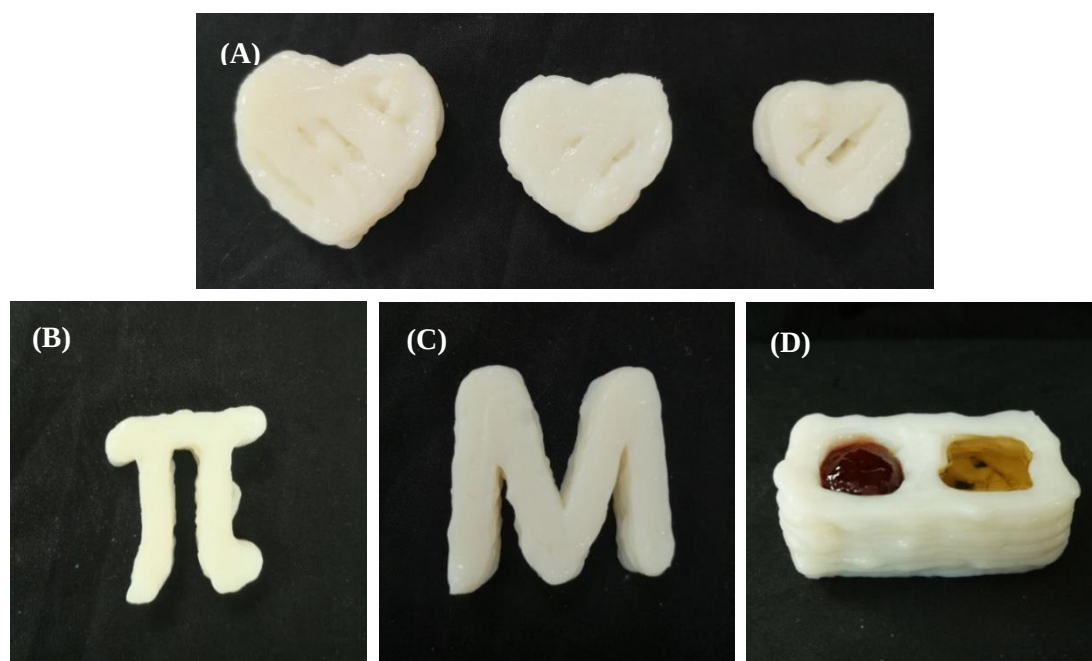
Fig. 4.9. Examples of various printable structures using MCC. (A) – (C) 3D-printed MCC shapes, symbol and letter; (D) fillable structure contains strawberry jam and honey in separate compartments to demonstrate that separate fillings could be utilised simultaneously in the same product.
