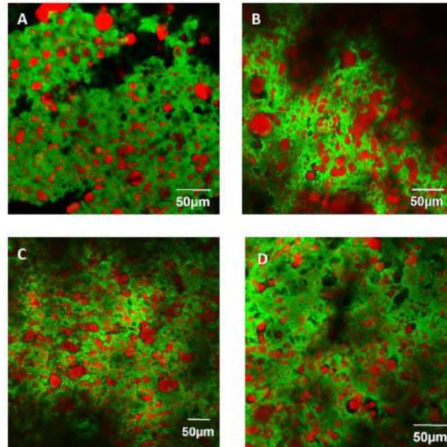
Fig. 6. CSLM Micrographs - A = Poured recipe A, B = Poured recipe F, C = Printed recipe A, and D = Printed recipe F (Images were taken using a 40× objective) (Red (Nile red stain) = Lipids, Green (Fast Green FCF) = Protein).
