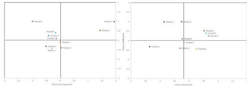
Fig. 10. Quality chart with the factor scores of the samples (averages of 3 independent repeat measurements) of the structural protein content dataset (Recipes D–H).
