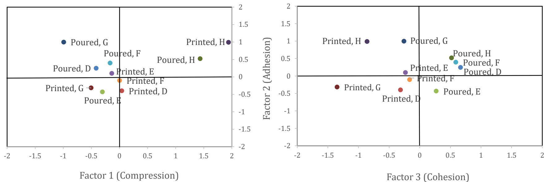
Fig. 3.10. Quality chart with the factor scores of the samples (averages of 3 independent repeat measurements) of the structural protein content dataset (Recipes D-H)
