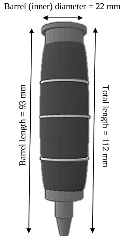
Fig. 2.11. Diagram showing dimensions of modified syringe for 3D food printing use (Note: unit dimensions are in mm)
