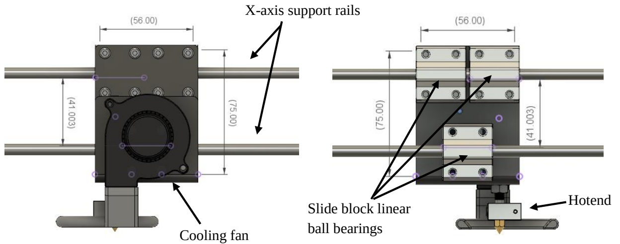
Fig. 2.10. 2D Sketch of the Cartesian 3D printer print head prior to modification (Front and Rear view) (Note: unit dimensions are in mm) (Adapted from Valsecchi, 2018).
