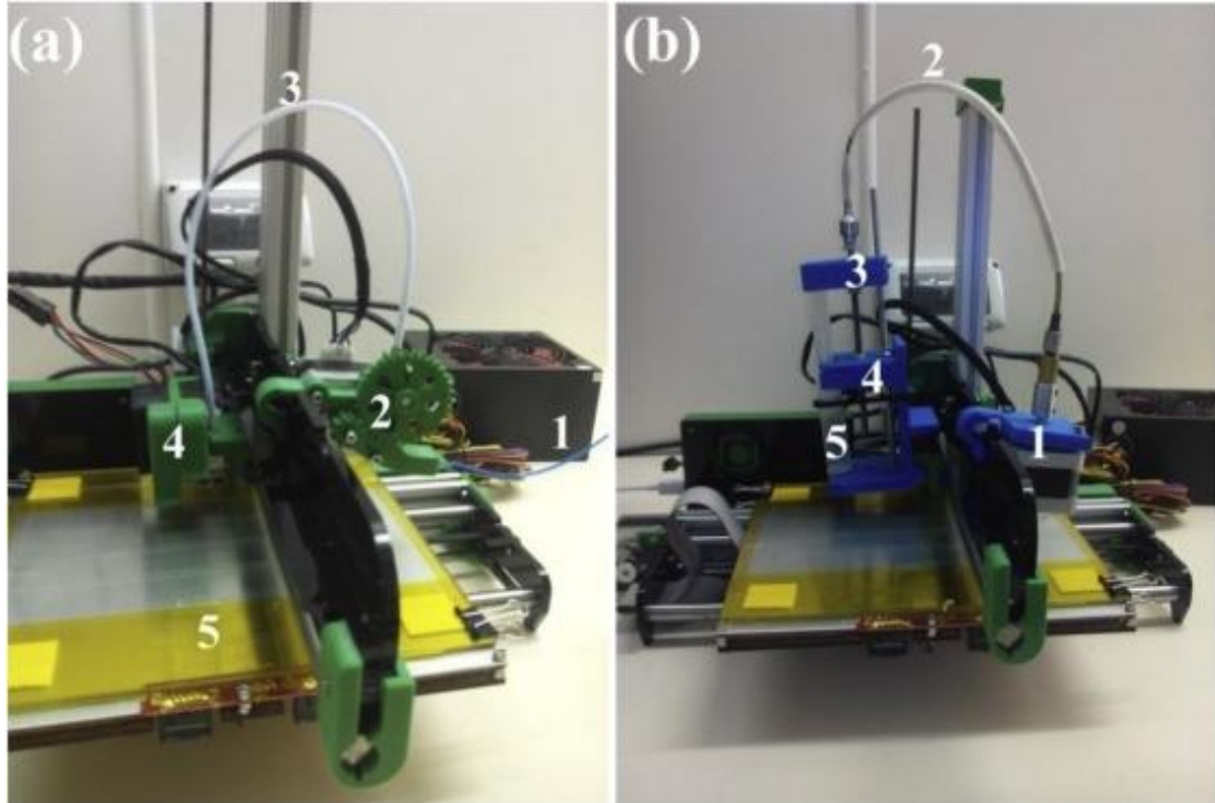
Fig. 2.8. Images of the Reprap Pro Ormerod 1 printer equipped with the plastic printing setup: (a) 1. PLA filament; 2. Extruder drive; 3. Filament Bowden tube; 4. Print head; 5. Print bed, and (b) the syringe-based food printing configuration: 1. Extruder motor mount and motor; 2. Flexible drive shaft; 3. Syringe plunger-holder; 4. Syringe mount; 5. Syringe (Obtained with permission from Le Tohic et al. , 2018).
