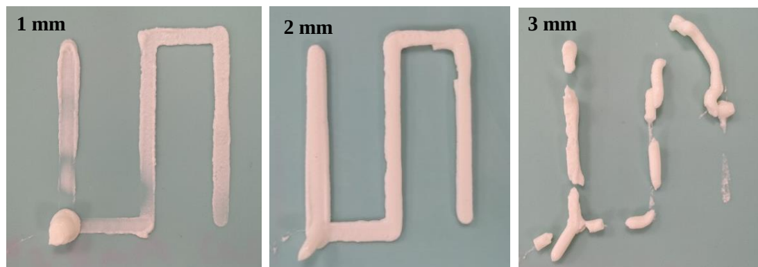
Fig. 2.17. Images of cream cheese 3D-printed in a continuous line shape where the nozzle is 1, 2 or 3 mm away from the print bed (Nozzle diameter = 2 mm)
