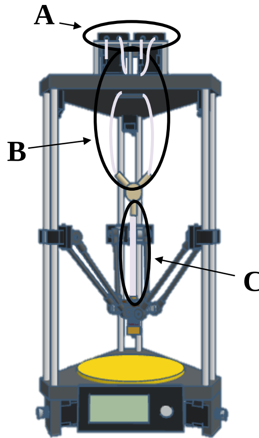
Fig. 2.5. Diagram demonstrating locations of tubing sections A (In/outlet tube), B (Peristaltic pump tubing), and C (Combined flow from Y-connector to nozzle)
