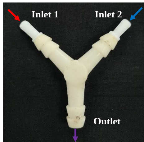
Fig. 2.4. Y-connector used to join silicone tubing from both peristaltic pumps to combine two inlet feeds.
