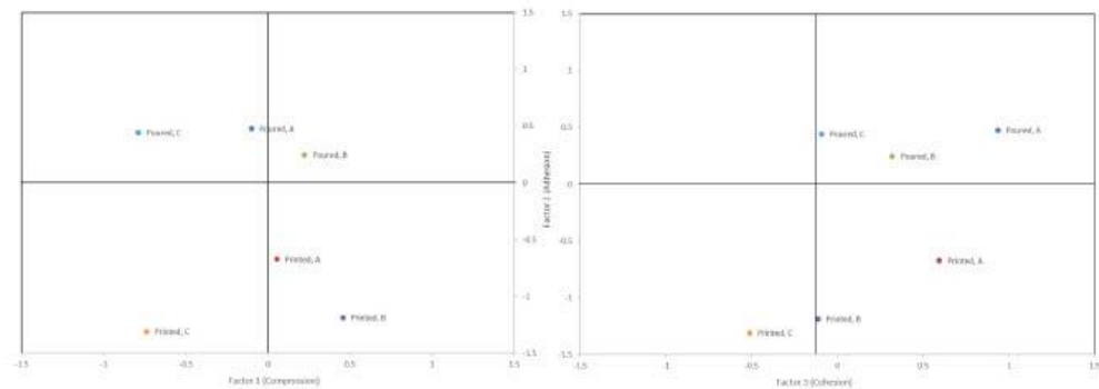
Fig. 9. Quality chart with the factor scores of the samples (averages of 3 independent repeat measurements) of the pH dataset (Recipes A–C).
