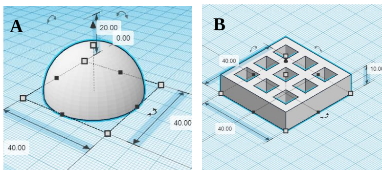
Fig. 4.1A and B. 3D-model dimensions of (A) hemisphere and (B) lattice (Note: dimensions are in mm)
