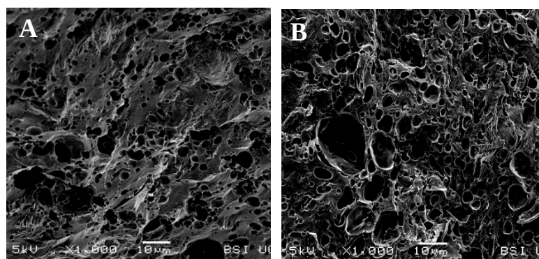
Fig. 3.11. SEM Micrographs showing Fig. 16A – recipe D, 3D-printed at 40°C (Magnification x 1,000) and Fig. 16B – recipe D, 3D-printed at 65°C (Magnification x 1,000)
