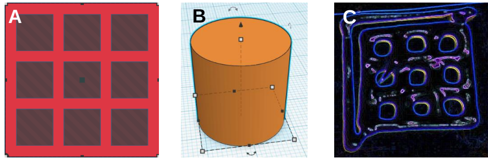
Fig. 3.4. A = CAD drawing of 40 mm square grid structure, B = CAD drawing of of 20 mm cylinder (AR = 1), C = Example of ‘Find Edges’ function of ImageJ analysis software. This function enables the user to measure the perimeter of the edges with increased accuracy in comparison to measurements using the original image without this function.
