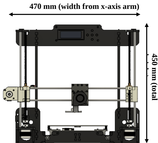
Fig. 2.6. 2D Sketch of Cartesian 3D printer prior to modification (Front view) (Note: unit dimensions are in mm) (Adapted from Valsecchi, 2018).
