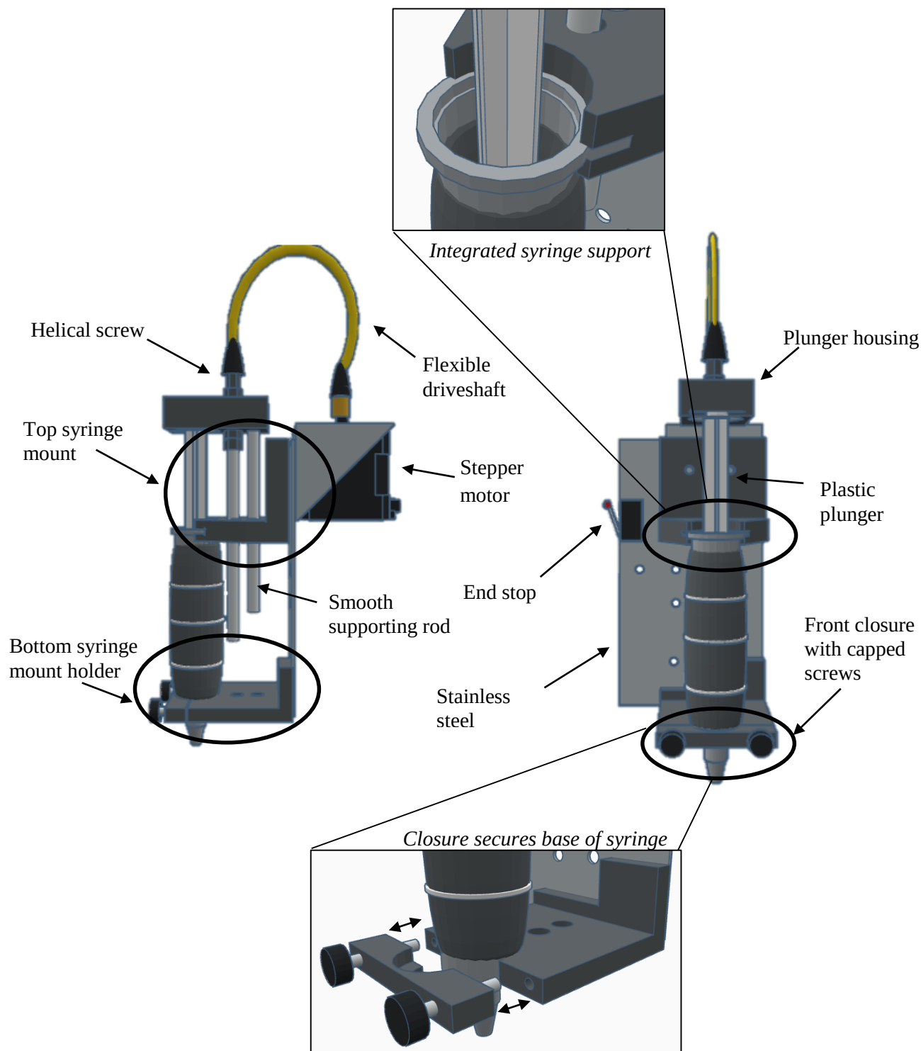
Fig. 2.9. Modified print head for Cartesian 3D printer (Side and front view)
