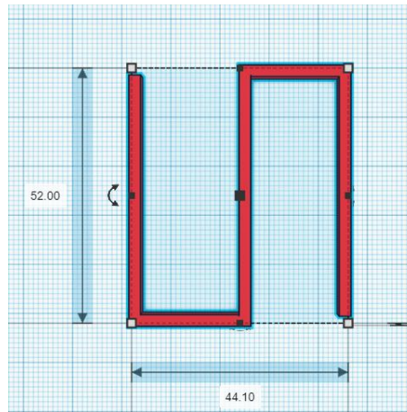
Fig. 2.14. Continuous line design. Line width/height – 2 mm. Total area – 380 mm 2 (Note: dimensional units are in mm)
