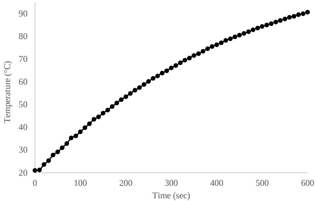
Fig. 2.12. Rate of heating of modified 3D food printer syringe for the Cartesian 3D printer
