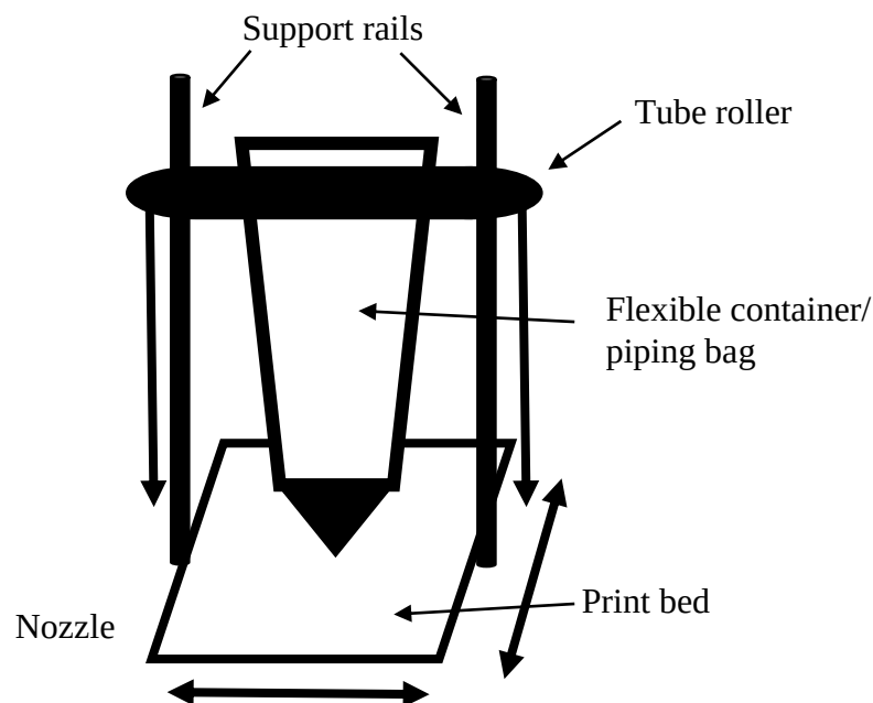
Fig. 7.1. Mock-up of possible alternative printing design involving a tube and roller system
