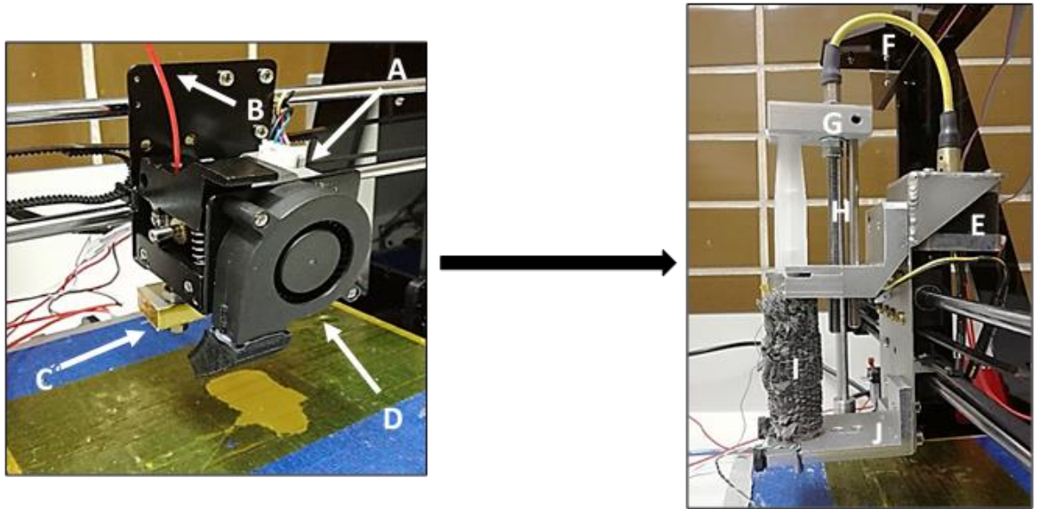
Fig. 3.1. A - Stepper Motor, B - Polylactic Acid (PLA) Filament, C - Hotend, D - Hotend Fan, E - Stepper Motor, F - Flexible Drive Shaft, G - Plunger Housing, H – Helical Screw, I- Syringe Barrel with Insulation, J - Syringe mount
