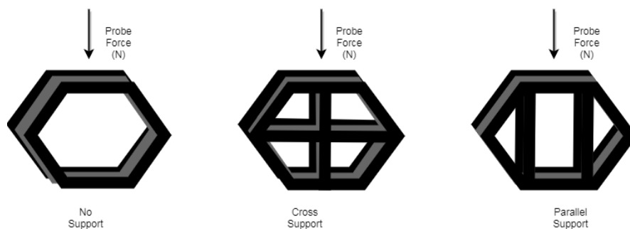
Fig. 1.4. Three different structural designs of printed chocolates analysed for snap quality using uniaxial compression (adapted from Mantihal et al. , 2017).
