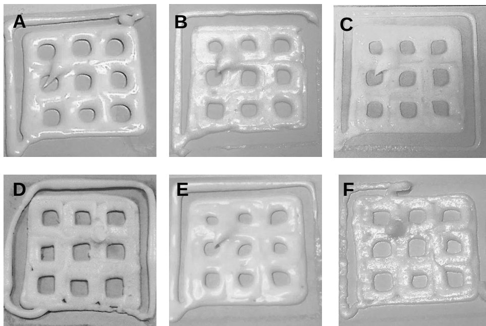
Fig. S3.1A-F. 40 mm x 2 mm printed grid structures with varying TSC contents (at 55% total moisture content), A = 1.5% TSC, B = 2% TSC, C = 2.5% TSC and with varying total moisture contents (with 2.5% TSC), D = 47% Total moisture, E = 50% Total moisture and F = 55% Total moisture
