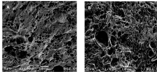
Fig. 11. SEM Micrographs showing Fig. 16A – recipe D, 3D printed at 40 °C (Magnification \times 1000 ) and Fig. 16B – recipe D, 3D printed at 65 °C (Magnification \times 1000 ).
