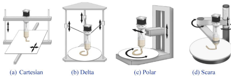
Fig. 2.1. Illustration of the various types of FDM printers available, including the primary difference between their movement paths (Obtained with permission from Sun et al. , 2018).
