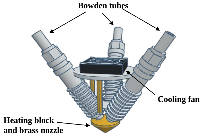
Fig. 2.2. Original Delta print head hotend and nozzle prior to modification.
