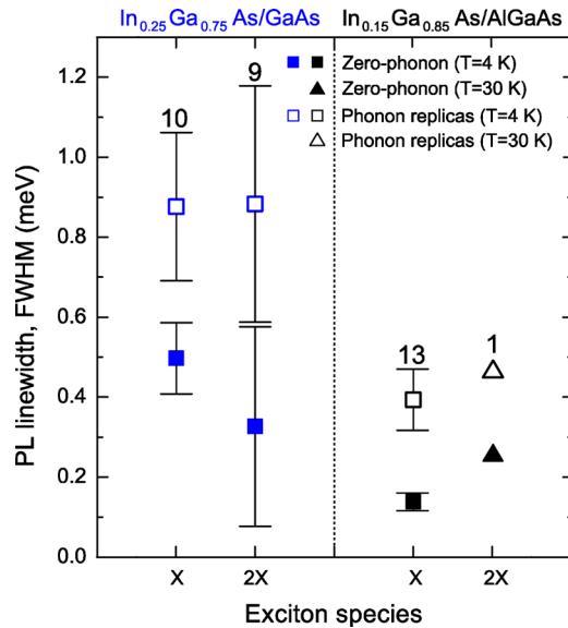
FIG. 3. (Color online) Measured linewidths (FWHM) represented by the mean values of in total 10 (13) different \text{In}_{0.25}\text{Ga}_{0.75}\text{As}/\text{GaAs} ( \text{In}_{0.15}\text{Ga}_{0.85}\text{As}/\text{AlGaAs} ) QDs. The bars indicate the standard deviation from the mean, and the numbers above indicate the number of measured QDs. In order to facilitate measurements of the biexciton phonon replica for the \text{In}_{0.15}\text{Ga}_{0.85}\text{As}/\text{AlGaAs} QDs, the temperature had to be raised to 30 K.
