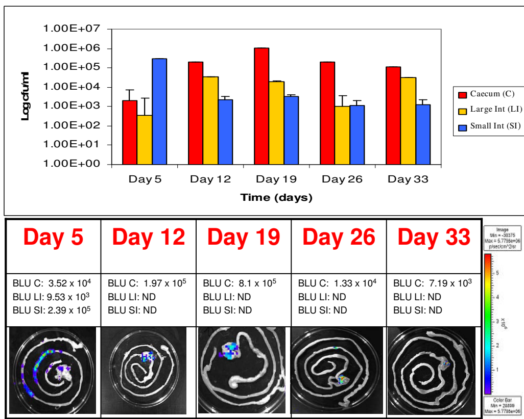
Figure 7 Correlation between bioluminescence and colony forming units (pLuxMC2). Illustrates the log colony forming units per ml from groups of mice feed pLuxMC2 for three days followed by thirty days of persistence study. The recovered gastrointestinal tracts (GIT) at each of the five time points were divided into the major physical sections and the average cfu/ml from the homogenised tissue samples are represented in red ( ) for the caecum, yellow ( ) for the large intestine and the small intestine in blue ( ). The image panel in both (a) and (b) represents an intact excised GIT at each time point. These images were obtained using an IVIS 100 system with 5 min of exposure and a binning value of 8. The color bar indicates the bioluminescence signal intensity (in photons s^{-1} cm^{-2} sr^{-1} ). ND, not detectable (bioluminescence counts less than 1 \times 10^4 photons s^{-1} ). BLU, bioluminescence counts (photons s^{-1} cm^{-2} sr^{-1} ); BLU C, recovered from caecum; BLU LI, from the large intestine and BLU SI from the small intestine.
