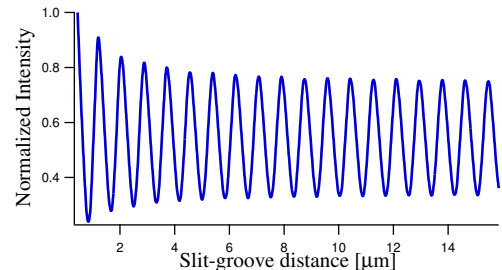
FIG. 2: Blue curve plots the same FDTD calculation as in Fig. 1 but extended to 16 \mu\text{m} slit-groove distance.
