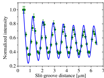
FIG. 1: Comparison of FDTD simulation and experiment. Green points are experimental data taken from [3]. Blue curve shows the FDTD result.
