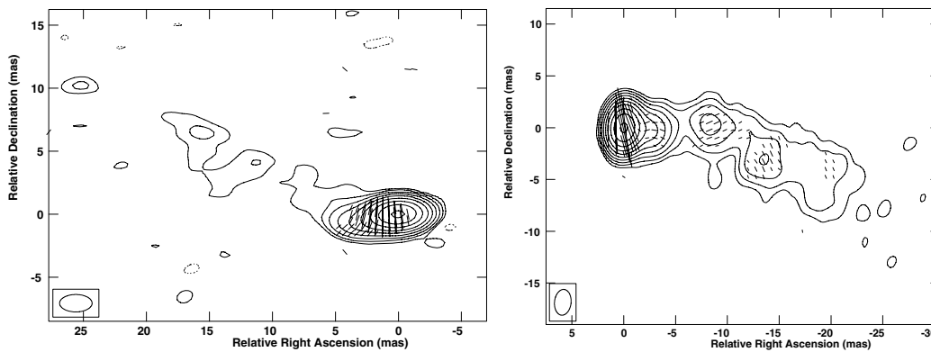
Figure 8. Total-intensity images with \chi vectors superimposed. Left-hand panel: The HBL 1133+704, epoch 1998.49. Contours are -0.35, 0.35, 0.70, 1.40, 2.80, 5.70, 11.50, 22.50, 45 and 90 per cent of the peak surface brightness of 98 \text{ mJy beam}^{-1} , \chi vectors: 1 \text{ mas} = 1.7 \text{ mJy beam}^{-1} . Right-hand panel: The LBL 1147+245, epoch 1995.53. Contours are -0.17, 0.17, 0.35, 0.70, 1.40, 2.80, 5.6, 11, 23, 45 and 90 per cent of the peak surface brightness of 479.4 \text{ mJy beam}^{-1} , \chi vectors: 1 \text{ mas} = 2.5 \text{ mJy beam}^{-1} .
