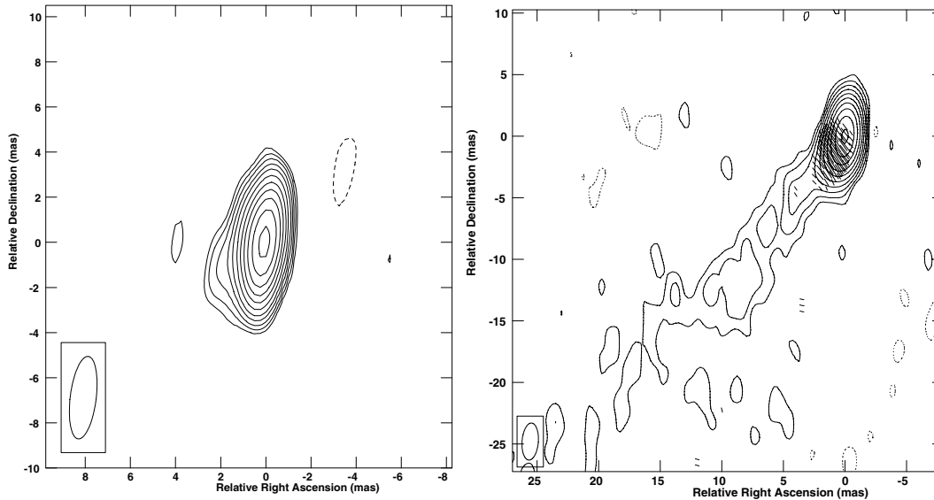
Figure 9. Total-intensity images of the HBL 1215+303 with \chi vectors superimposed. Left-hand panel: Epoch 1993.15 (no polarization detected). Contours are -2.8, 2.8, 4.0, 5.6, 8, 11, 16, 23, 32, 45, 64 and 90 per cent of the peak surface brightness of 33.4 \text{ mJy beam}^{-1} . Right-hand panel: Epoch 1998.49. Contours are -0.17, 0.17, 0.35, 0.70, 1.40, 2.80, 5.70, 11.50, 22.50, 45 and 90 per cent of the peak surface brightness of 231 \text{ mJy beam}^{-1} , \chi vectors: 1 \text{ mas} = 2 \text{ mJy beam}^{-1} .
