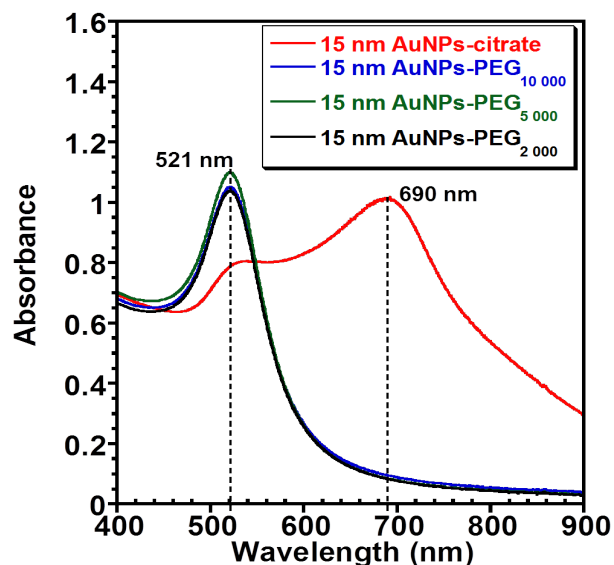
Figure S1. Uv-visible absorbance data showing the effect of salt (0.157 M NaCl) on: citrate-stabilised Au NPs, Au NPs stabilised with mPEG 2000 -SH ligands, Au NPs stabilised with mPEG 5000 -SH ligands and Au NPs stabilised with mPEG 10000 -SH ligands. Spectrum were taken 1 minute after adding NaCl.
