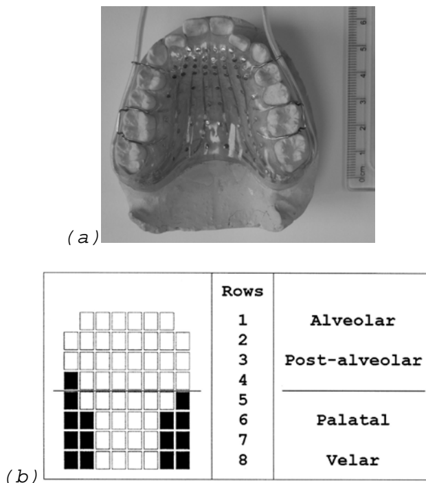
Figure 1. A Reading EPG plate of a normal speaker placed on top of a plaster impression of the hard palate and teeth is shown in (a). A single EPG frame, showing a typical contact pattern for a high vowel /i/ or /u/ is shown in (b), along with EPG frame row numbers and the phonetic regions of the palate.
