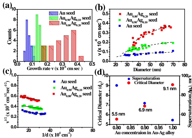
Figure 4. (a) Growth rate distributions with different catalyst systems showing the highest Ge nanowire growth rate with Au 0.80 Ag 0.20 -Ge seeds. Plots in part (b) show the quadratic dependence of the growth rate with nanowire diameter grown with three different seeds, (c) plots of the square root of the growth velocity showing the linear dependence with inverse diameter, agreeing well with Gibbs-Thompson effect. Part (d) shows the gradual decrease in the critical diameter of Ge nanowires and an increase in the supersaturation with Ag incorporation in the Au seed.
