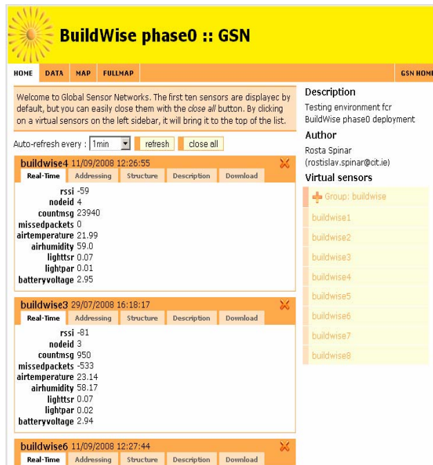
Figure 8. GSN web based WSN Interface
