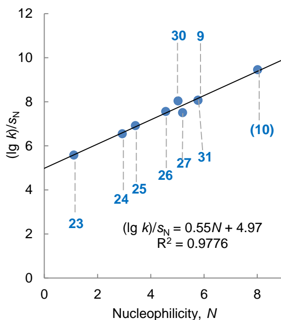
Figure 7. Plot of (\lg k/s_N) vs. N for vinyl cation 3 , from its reactions with various nucleophiles.
