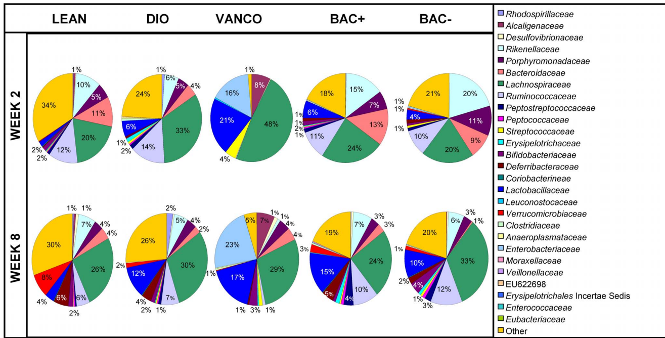
Figure 4. Microbial distribution at family level. Family level microbial distribution in all data sets at intervention week 2 and week 8. The pie charts represent total percentage read number for the corresponding colour coded family ( n = 9-10 per group). doi:10.1371/journal.pone.0065790.g004
