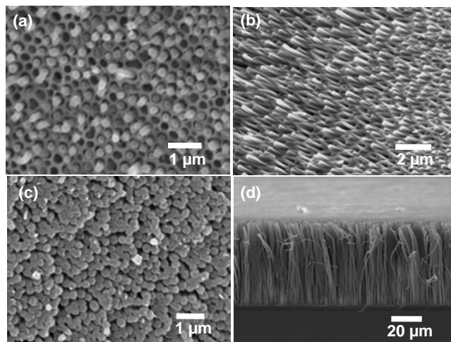
Figure 1 Scanning electron microscope images of arrays of mesoporous carbon nanofibres after being calcined at 600 °C for 3 hours. (a) top and (b) side views of mesoporous carbon nanofibre arrays within the pores of AAO membranes, (c) Top and (d) side views of nanofibre arrays prepared on a silicon wafer by a supercritical CO 2 drying process following the dissolving of AAO membrane.
