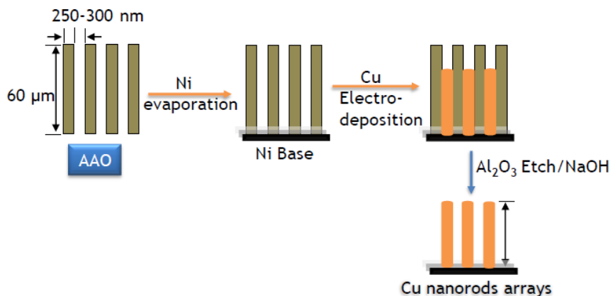
Figure 1. Schematic illustration of the synthesis process of the high aspect ratio Cu nanorod arrays.
