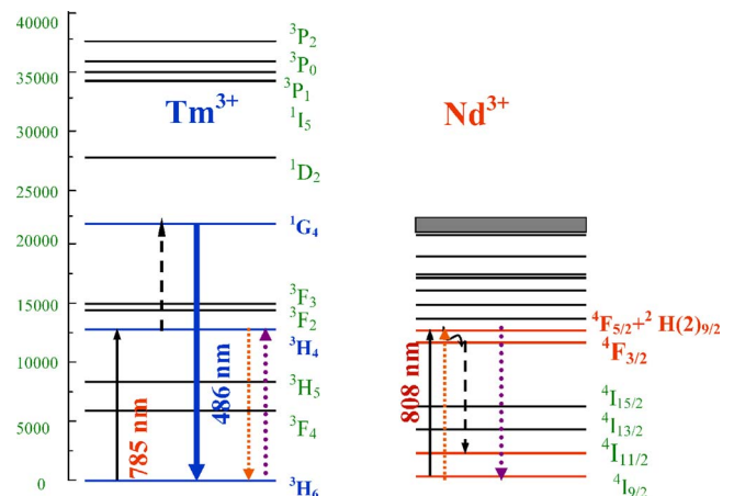
FIG. 12. (Color online) Energy level scheme of Tm 3+ and Nd 3+ in YAG and energy transfer upconversion mechanism responsible for the blue emission in the codoped crystal.
