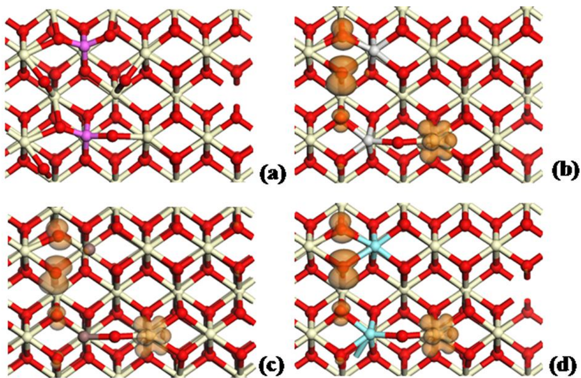
Figure 8: Spin density for two substituted 3+ dopants with a compensating oxygen vacancy. (a): Al 3+ , (b) Sc 3+ , (c) In 3+ and (d) Y 3+ .
